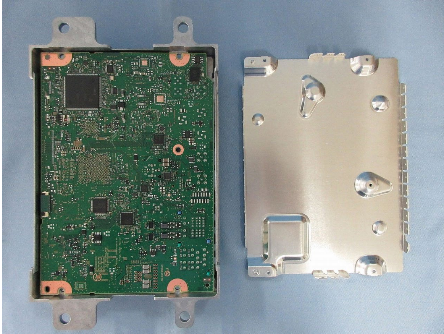
PCB-MAIN S-side
