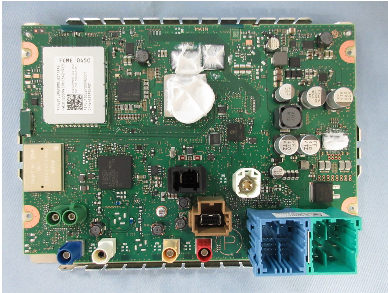
PCB-MAIN C-side
