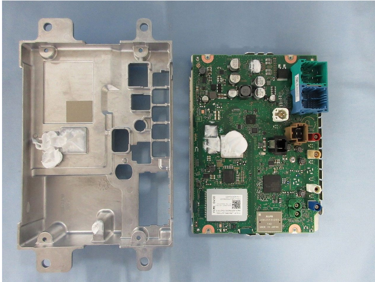
PCB-MAIN C-side
