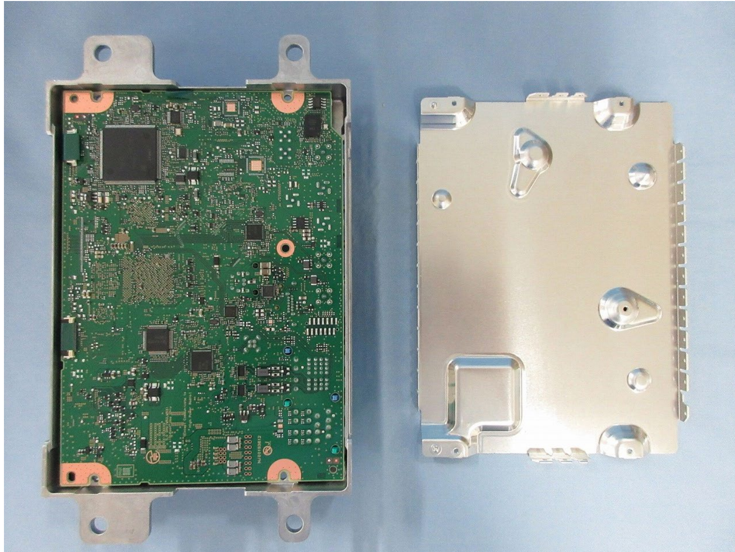
PCB-MAIN S-side
