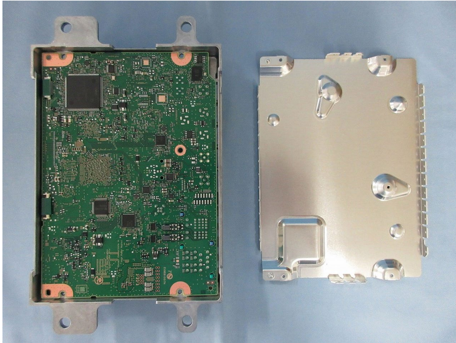
PCB-MAIN S-side
