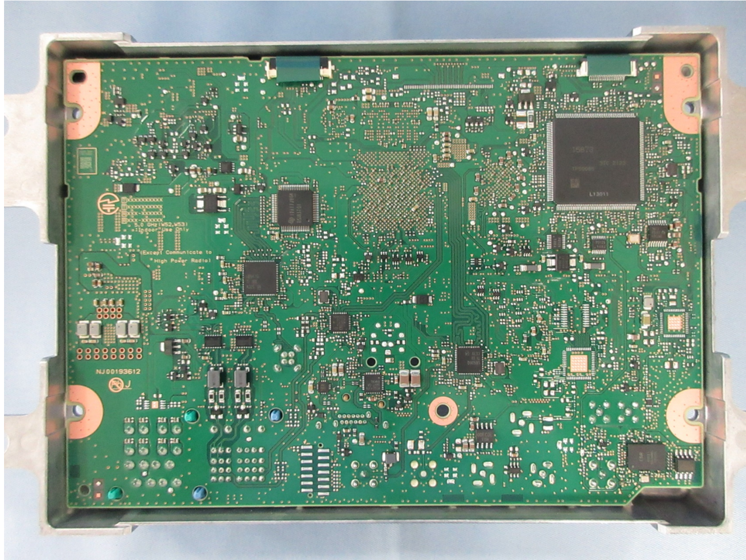
PCB-MAIN S-side
