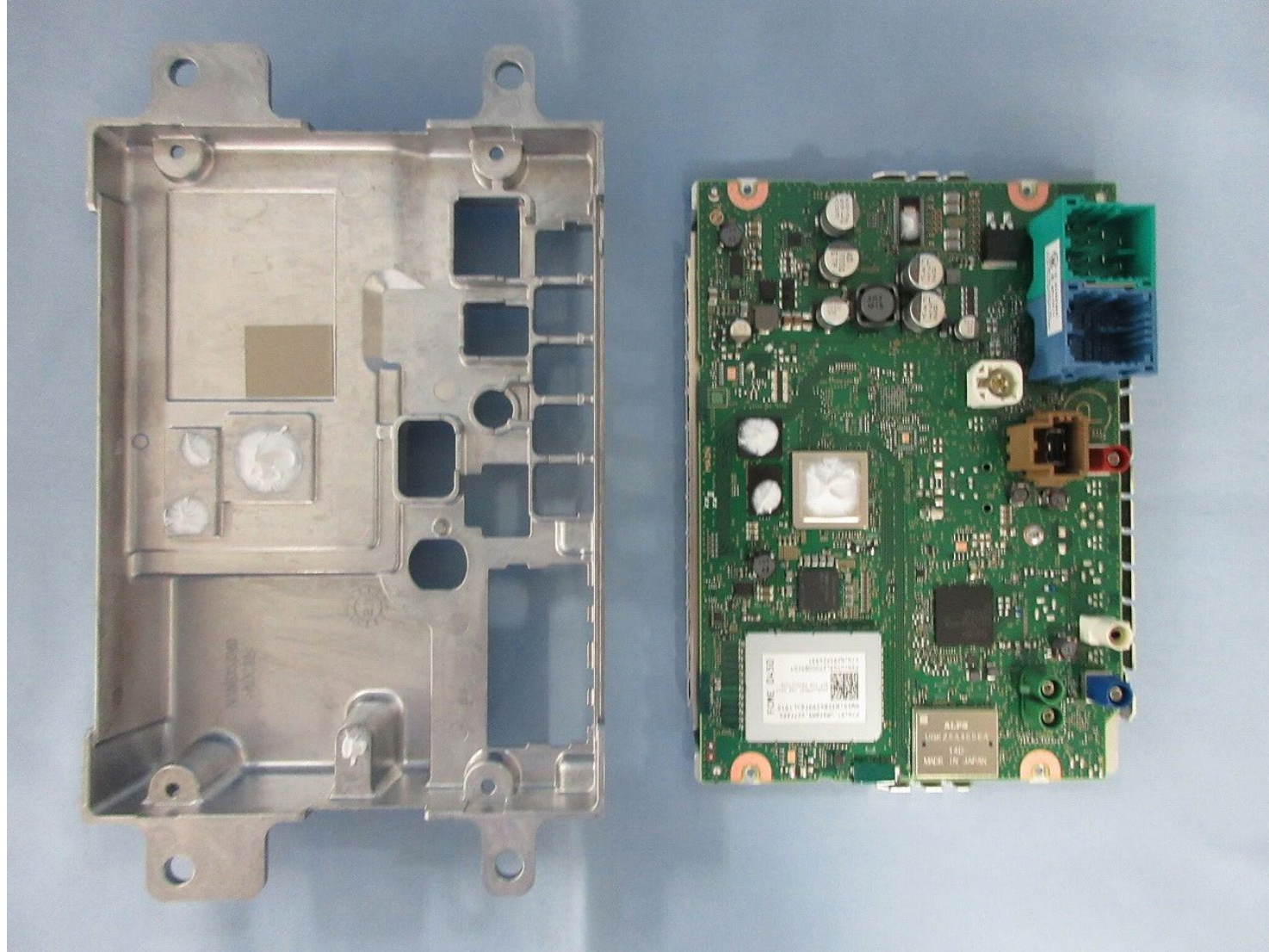
PCB-MAIN C-side
