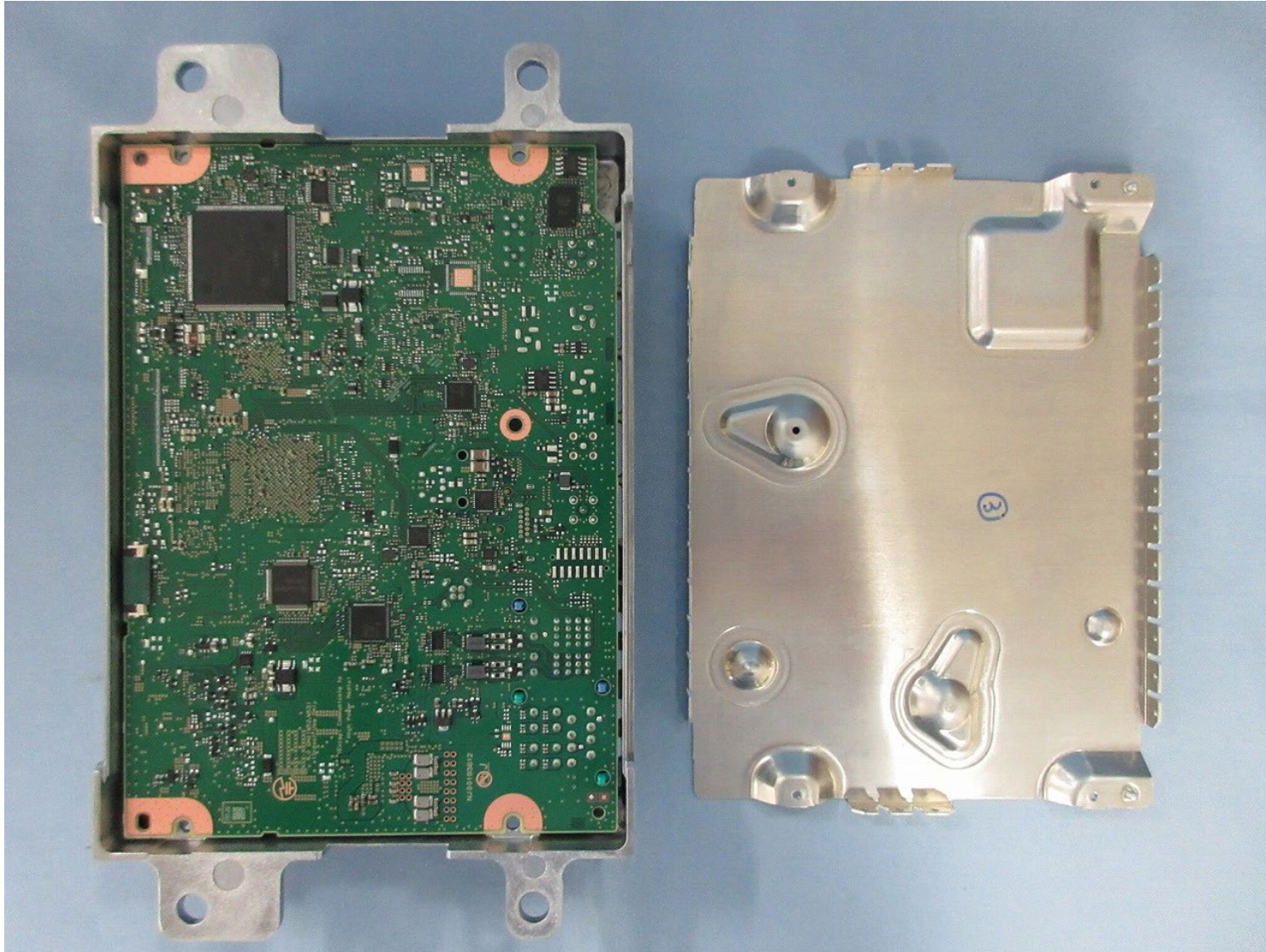
PCB-MAIN S-side
