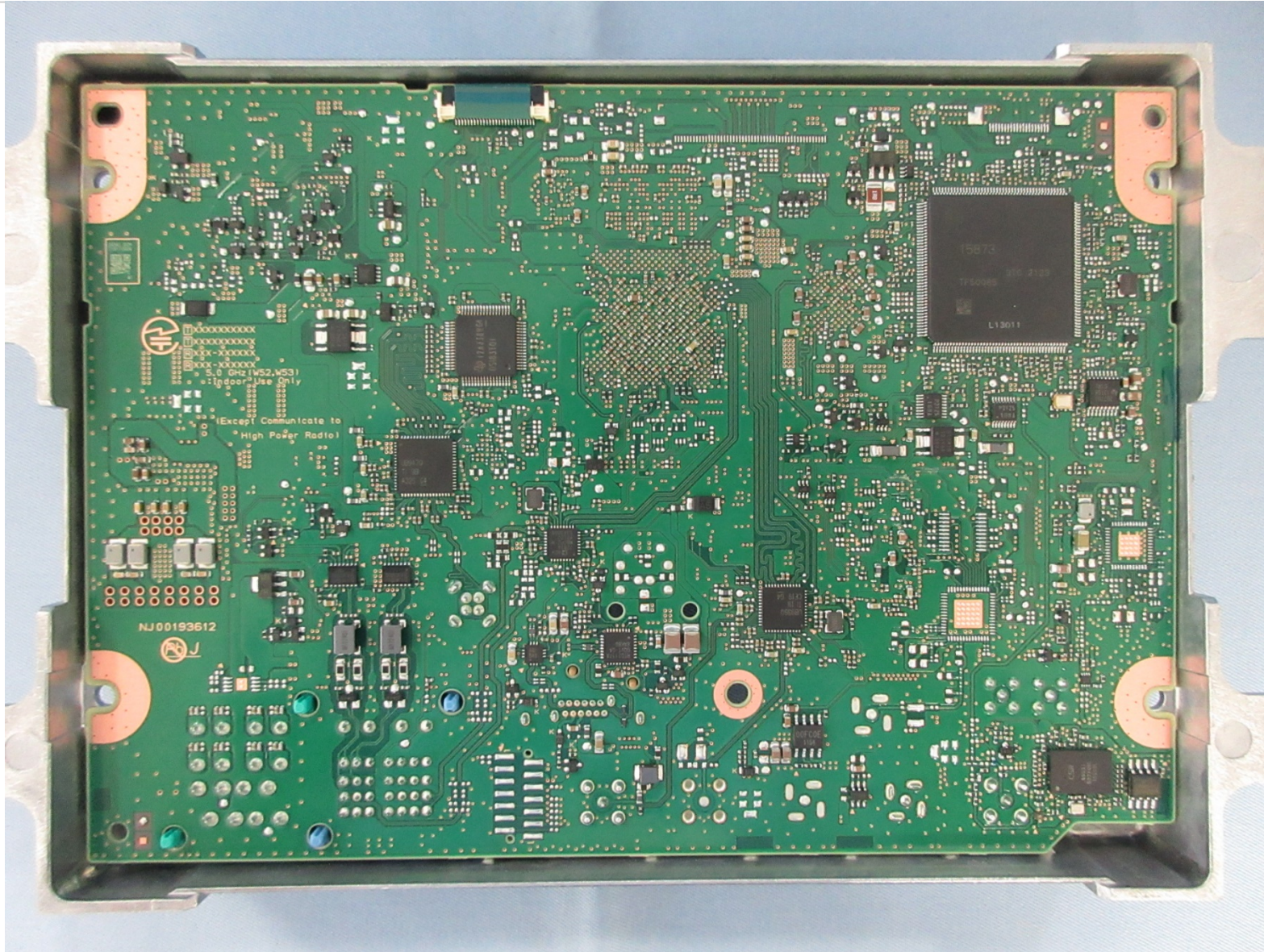
PCB-MAIN S-side
