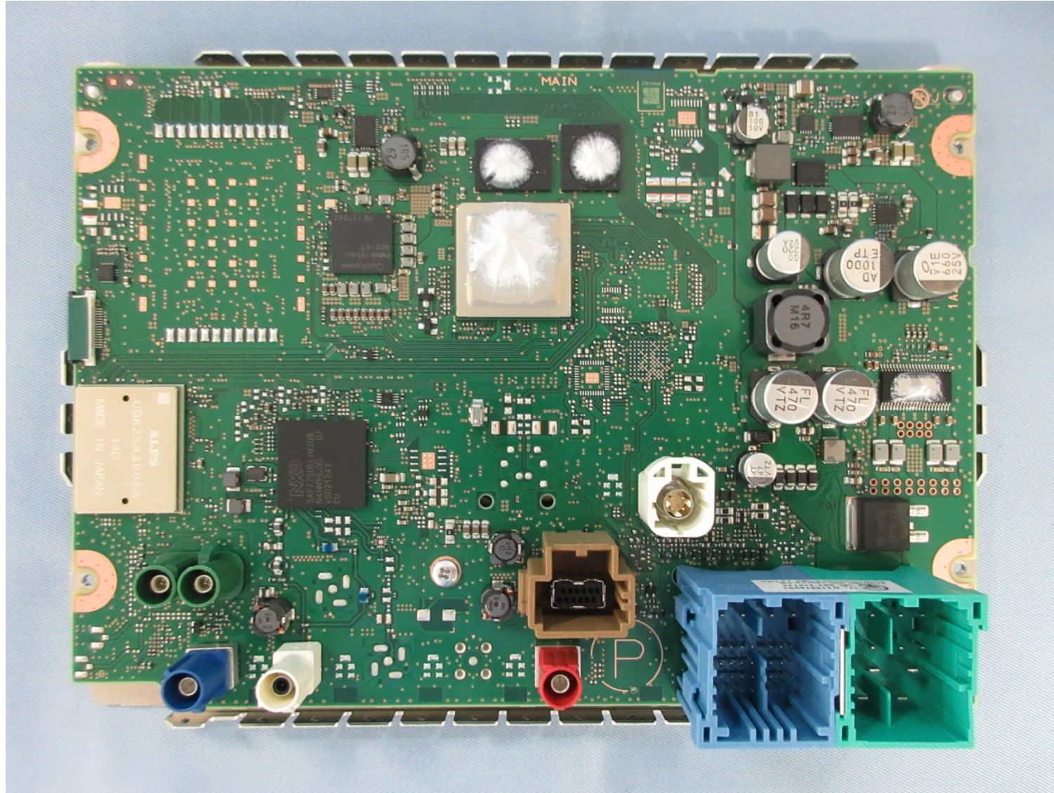
PCB-MAIN C-side
