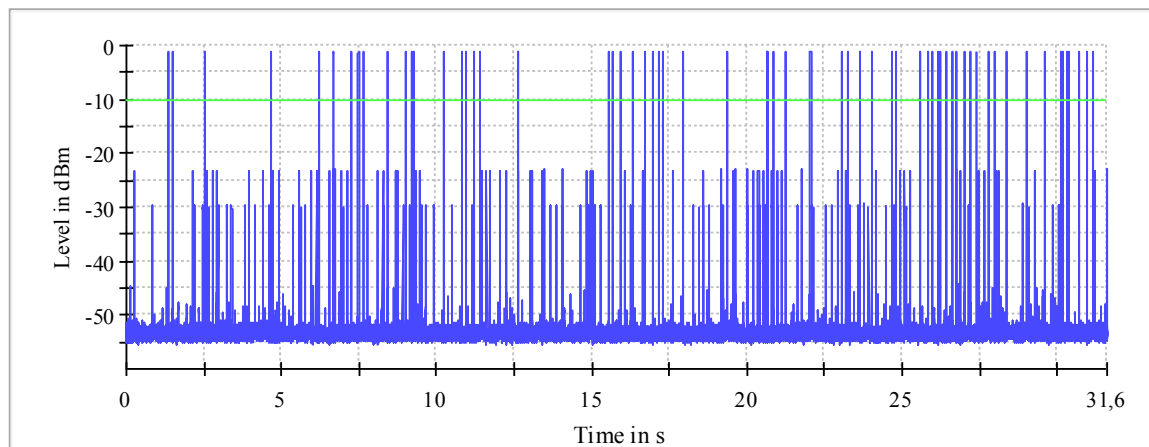
Plot 21: Mode 3, Time of Channel Occupancy, high channel
