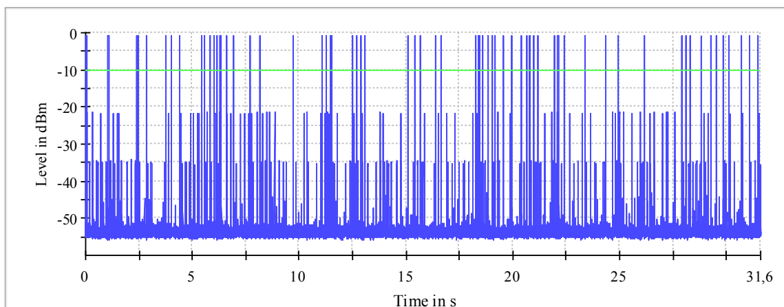
Plot 17: Mode 2, Time of Channel Occupancy, mid channel
