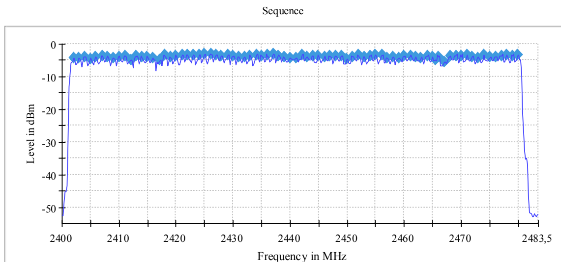
Plot 11: Mode 2, Hopping Frequencies
