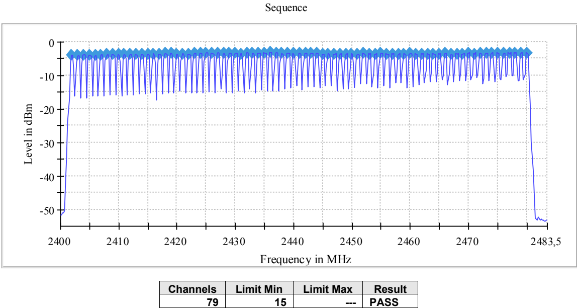
Plot 10: Mode 1, Hopping Frequencies
