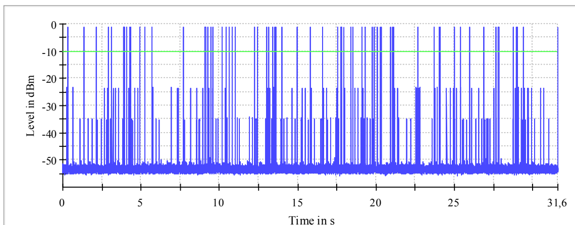
Plot 15: Mode 1, Time of Channel Occupancy, high channel
