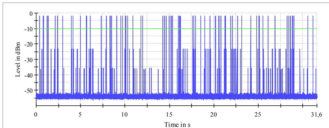
Plot 13: Mode 1, Time of Channel Occupancy, low channel
