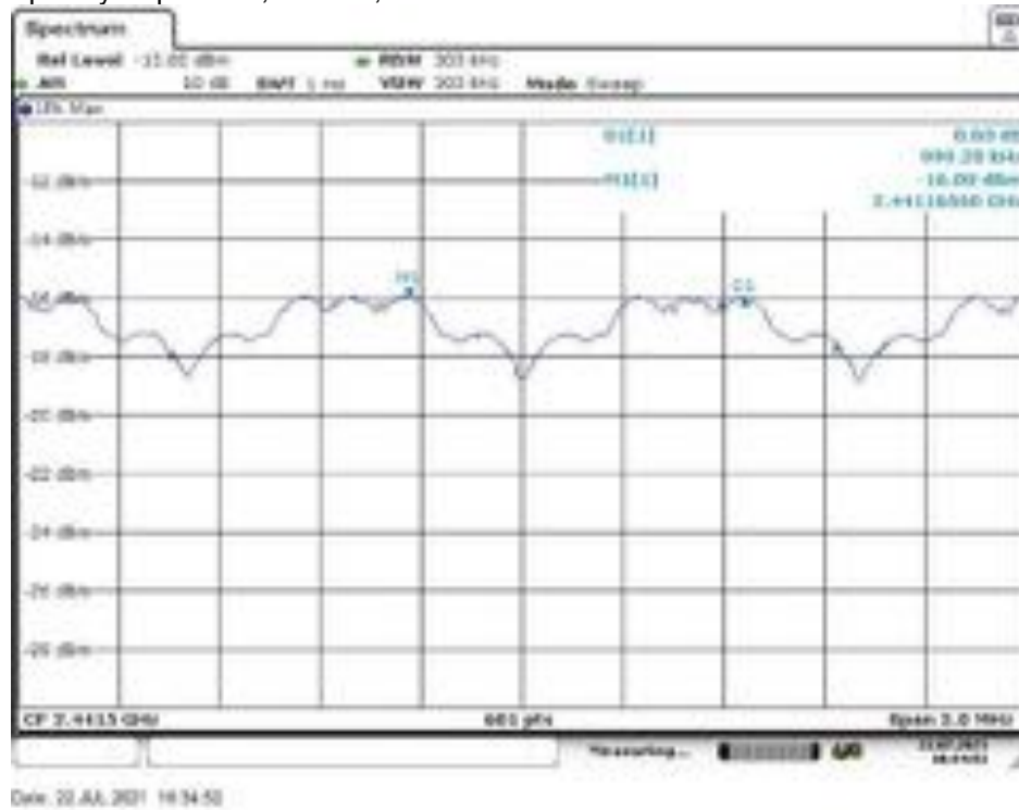
Plot 5: Carrier Frequency Separation, Mode 2, mid channel*
