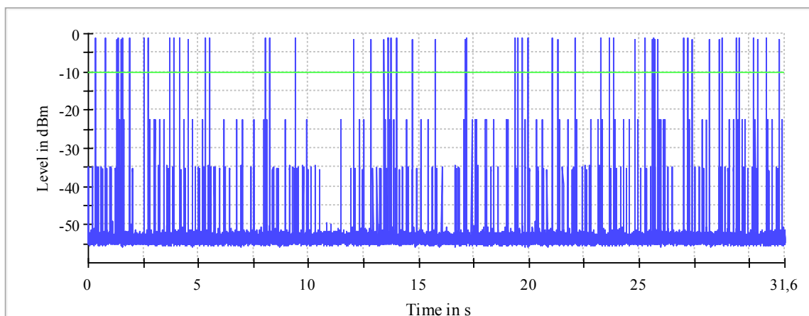
Plot 14: Mode 1, Time of Channel Occupancy, mid channel
