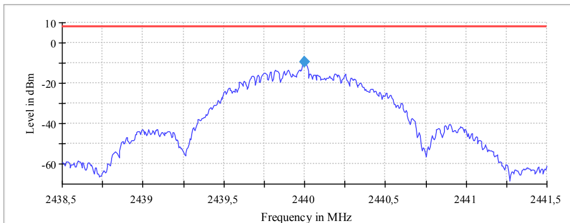
Plot 14: Mode 1, Peak PSD, mid channel
