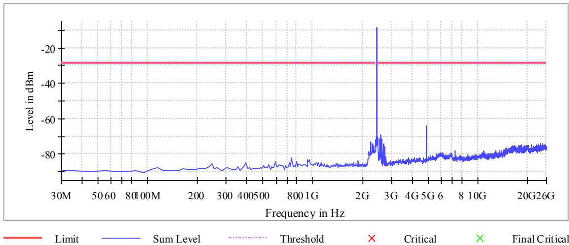
Plot 21: Mode 1, CSE, mid channel
