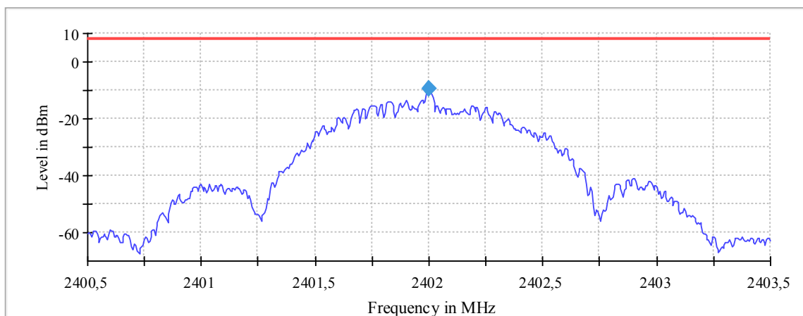
Plot 13: Mode 1, Peak PSD, low channel
