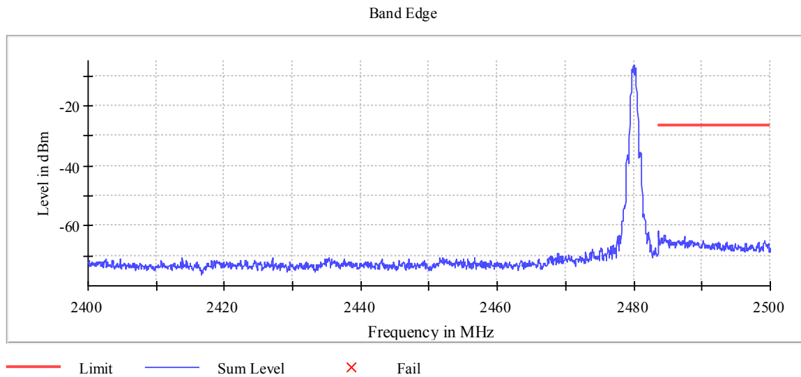
Plot 17: Mode 1, BEC, high channel
