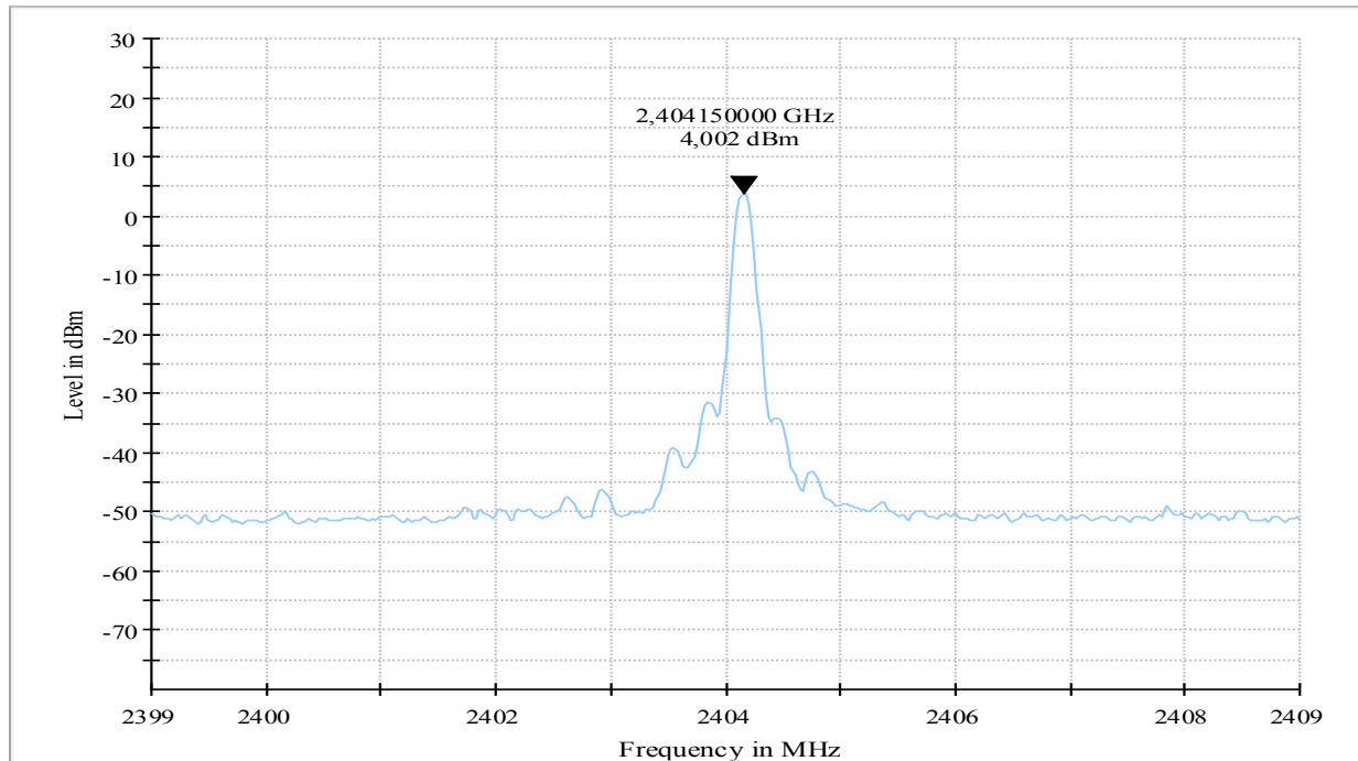
Plot 10: Mode 1, Peak EIRP, low channel
