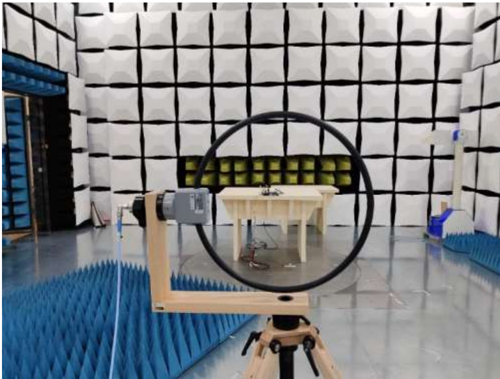
Photo No. 37: Test set-up 8.1, test antenna view
