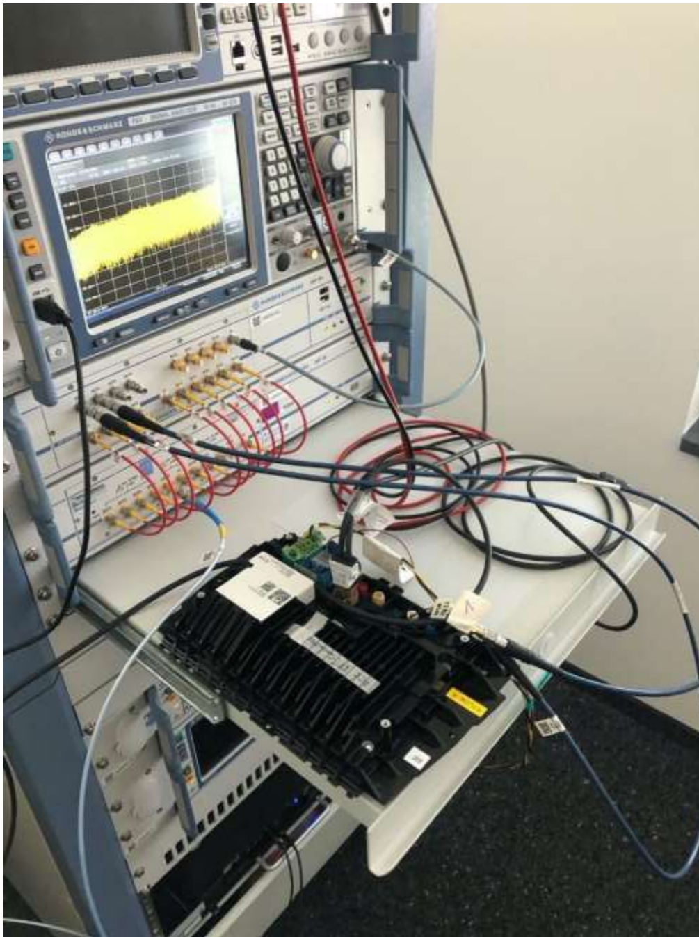
Photo No. 39: test set-up 8.4 with R1LOW-R connected with TS8997
