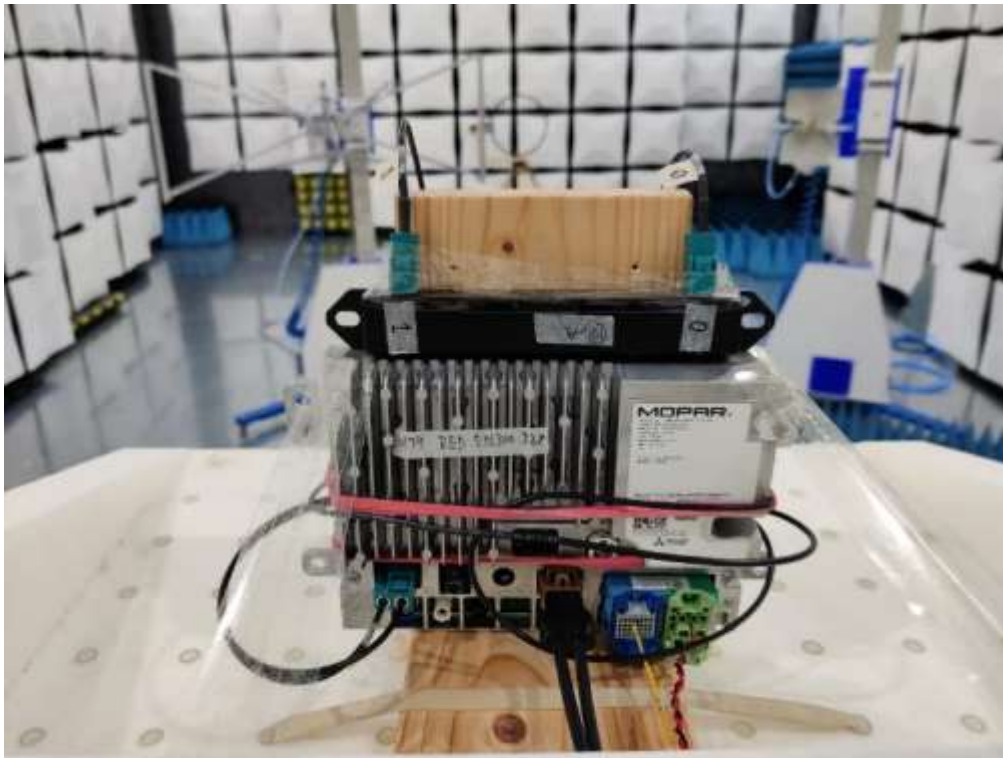
Photo No. 35: Test set-up 8.2, test antenna view
