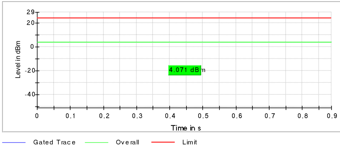
Plot 147: Mode 4, U-NII-1, AVGPm-G Gated Average Power Measurement, low channel
