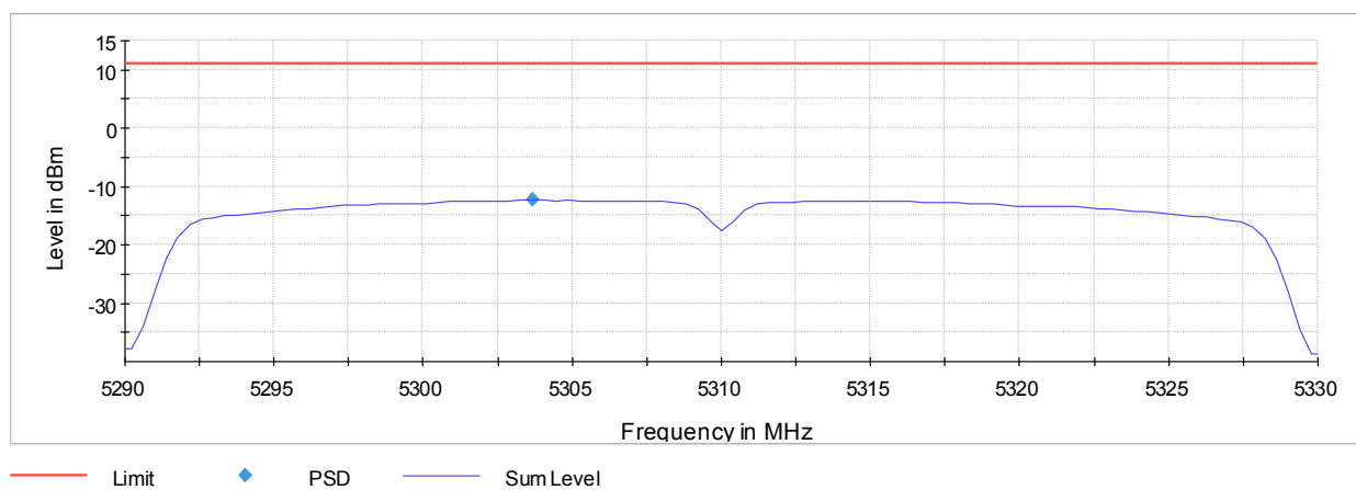
Plot 237: Mode 3, U-NII-2A, Peak PSD, high channel
