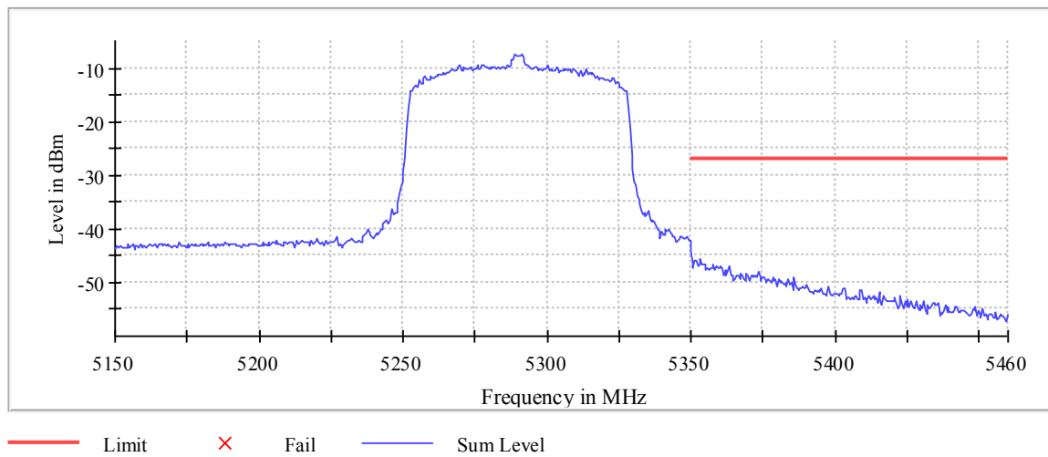
Plot 262: Mode 6, BEC, U-NII-1 & U-NII-2A, high channel, 5290 MHz
