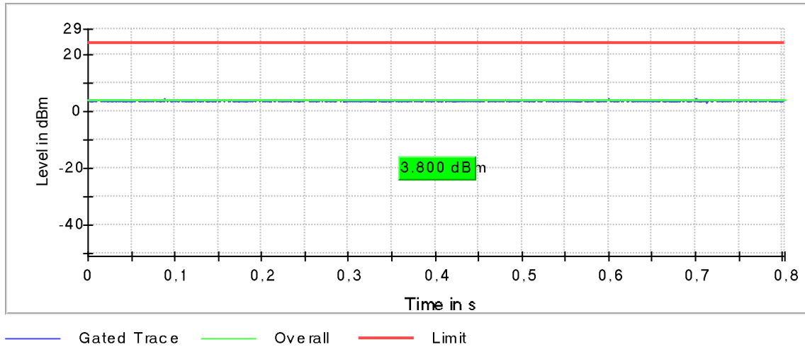
Plot 171: Mode 5, U-NII-2A, AVGP-M-G Gated Average Power Measurement, low channel
