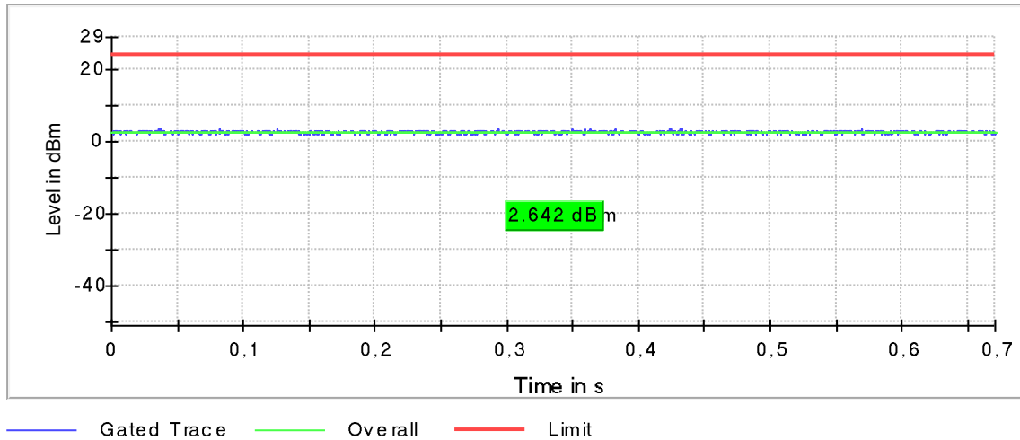
Plot 182: Mode 6, U-NII-2C, AVGPM-G Gated Average Power Measurement, high channel
