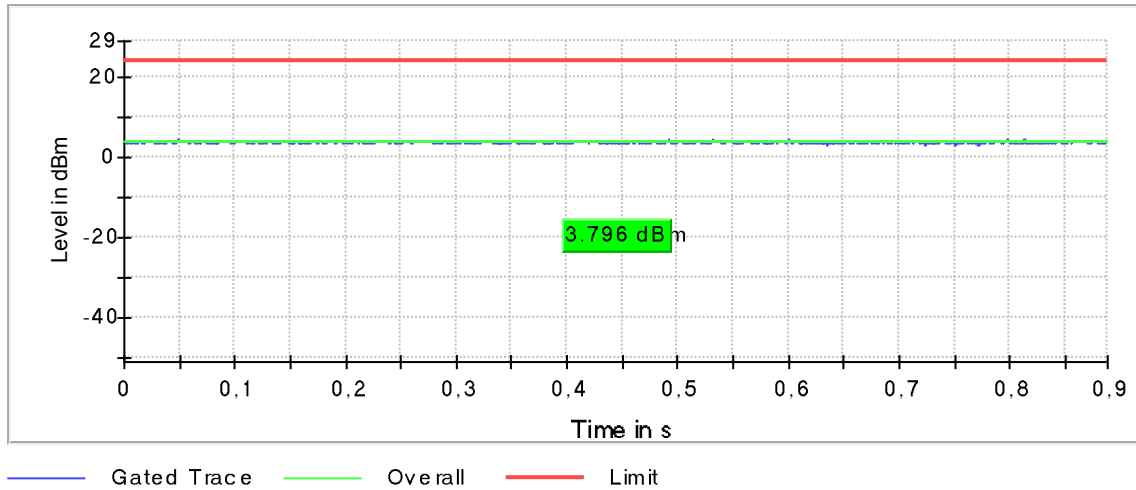
Plot 153: Mode 4, U-NII-2C, AVGP-M-G Gated Average Power Measurement, low channel
