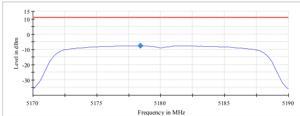
Plot 195: Mode 1, U-NII-1, Peak PSD, low channel
