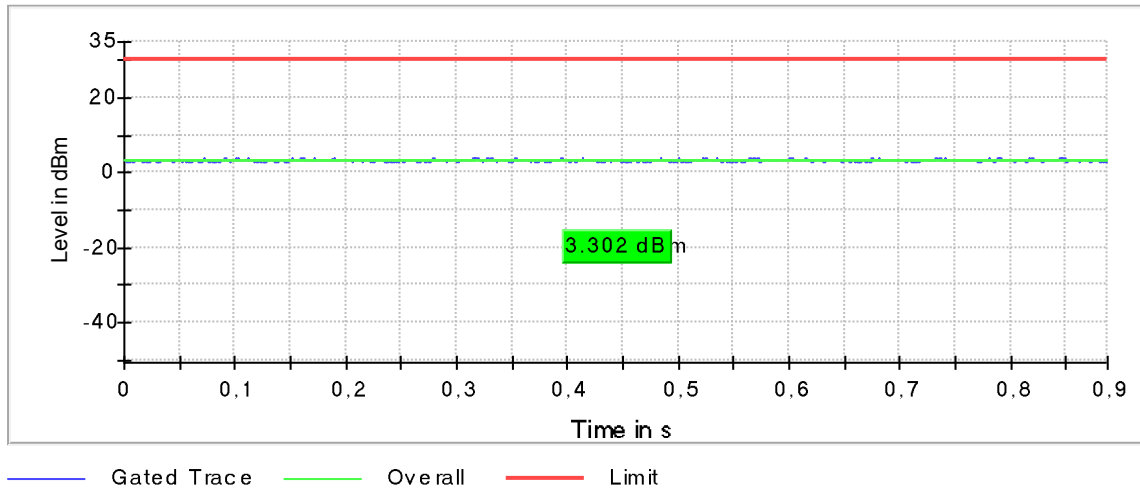
Plot 145: Mode 2, U-NII-3, AVGPM-G Gated Average Power Measurement, mid channel
