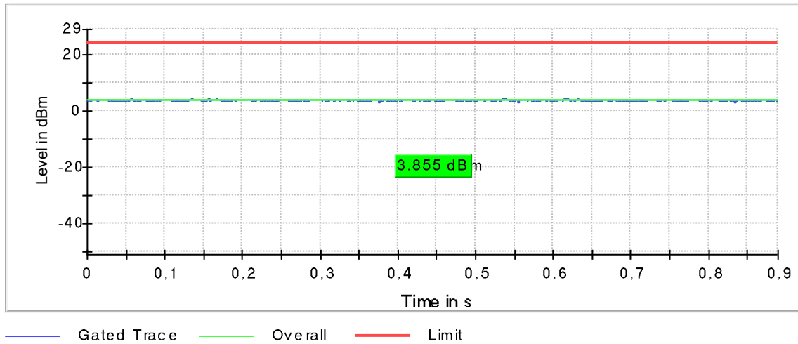
Plot 154: Mode 4, U-NII-2C, AVGP-M-G Gated Average Power Measurement, mid channel
