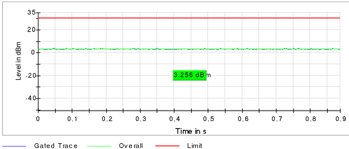
Plot 158: Mode 4, U-NII-3, AVGPM-G Gated Average Power Measurement, mid channel
