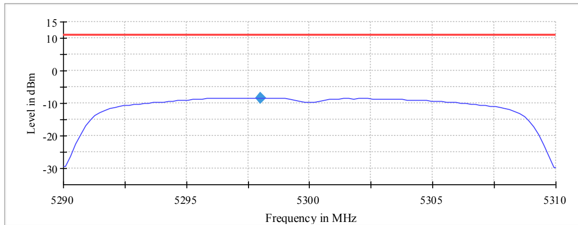
Plot 225: Mode 4, U-NII-2A, Peak PSD, mid channel
