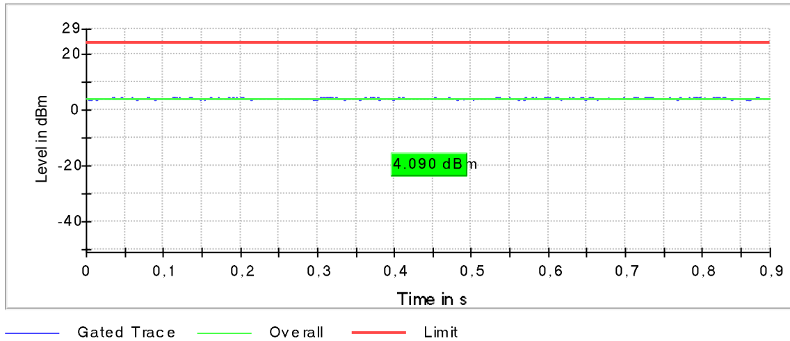
Plot 137: Mode 2, U-NII-2A, AVGP-M-G Gated Average Power Measurement, low channel
