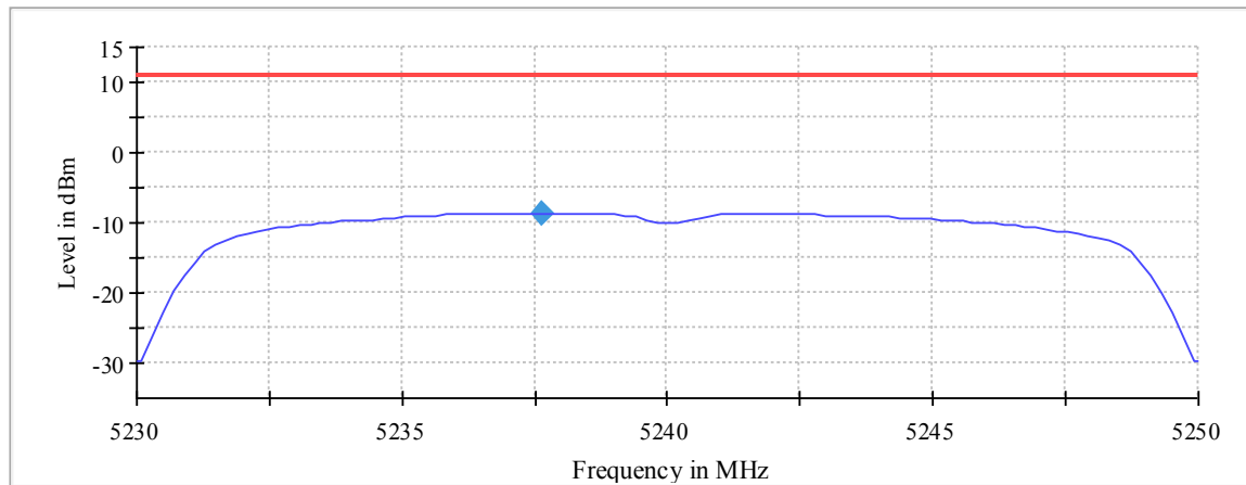
Plot 223: Mode 4, U-NII-1, Peak PSD, high channel
