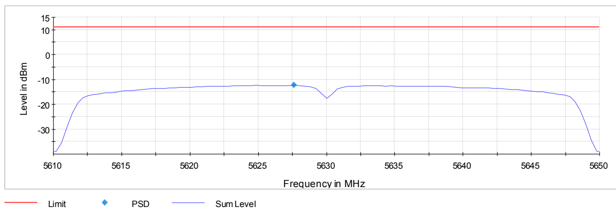
Plot 239: Mode 3, U-NII-2C, Peak PSD, mid channel
