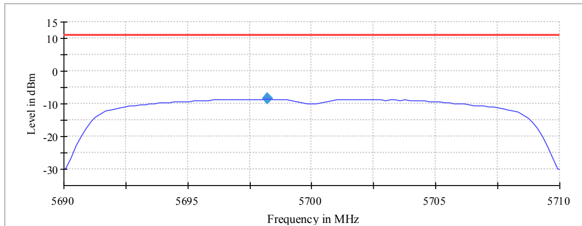
Plot 216: Mode 2, U-NII-2C, Peak PSD, high channel
