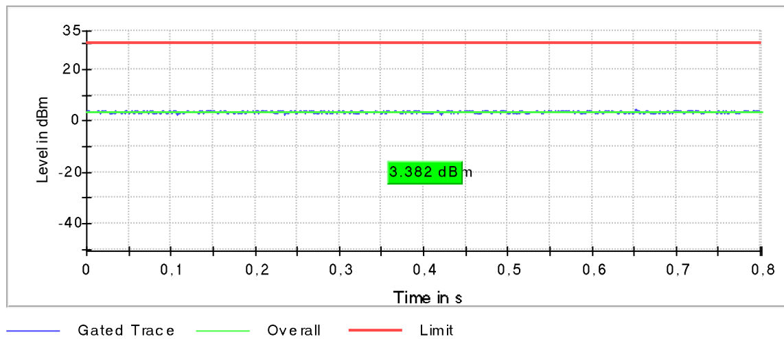
Plot 177: Mode 3, U-NII-3, AVGP-M-G Gated Average Power Measurement, high channel
