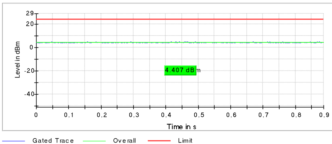
Plot 139: Mode 2, U-NII-2A, AVGP-M-G Gated Average Power Measurement, high channel
