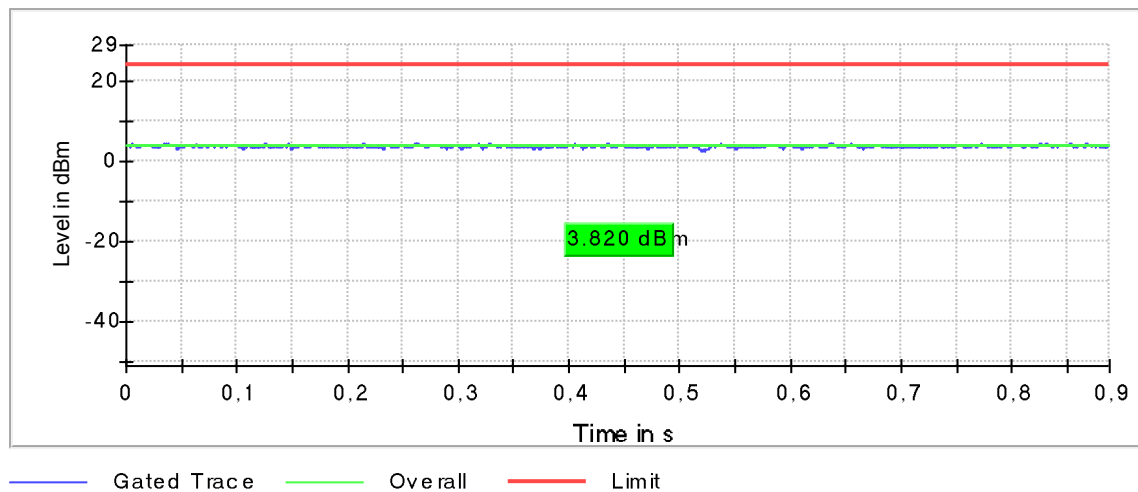
Plot 155: Mode 4, U-NII-2C, AVGP-M-G Gated Average Power Measurement, high channel
