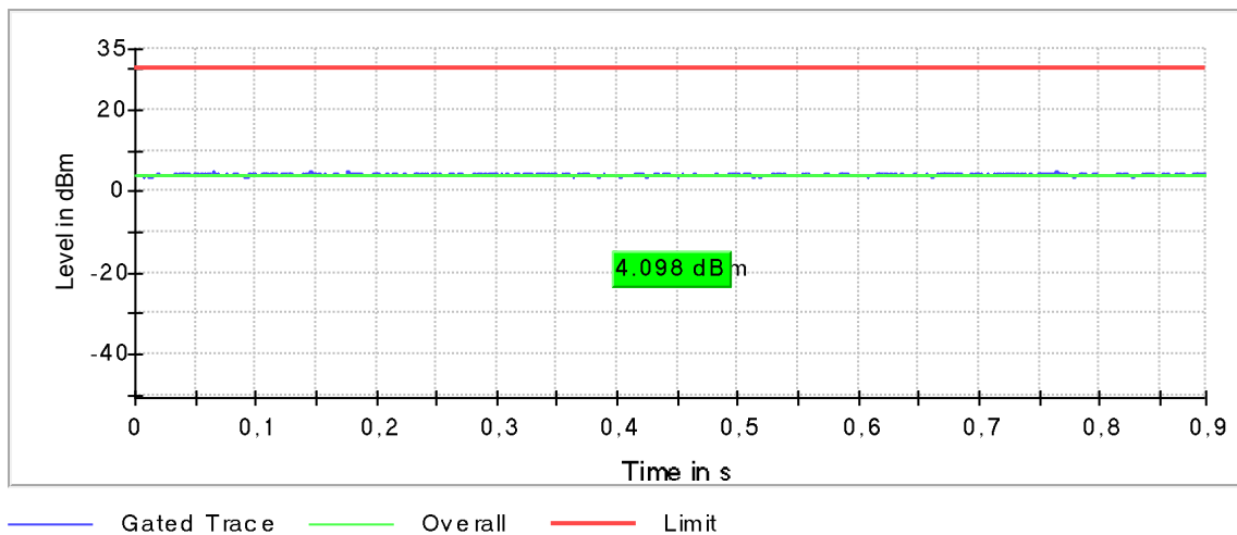
Plot 157: Mode 4, U-NII-3, AVGPM-G Gated Average Power Measurement, low channel
