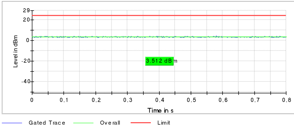
Plot 164: Mode 3, U-NII-2C, AVGP-M-G Gated Average Power Measurement, low channel
