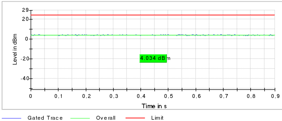
Plot 150: Mode 4, U-NII-2A, AVGPm-G Gated Average Power Measurement, low channel
