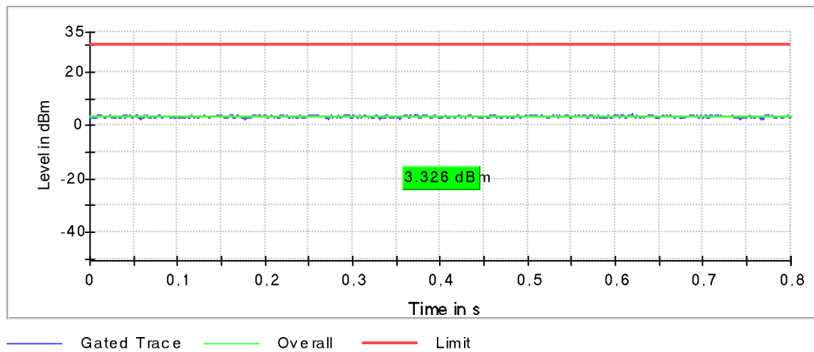
Plot 168: Mode 3, U-NII-3, AVGP-M-G Gated Average Power Measurement, high channel
