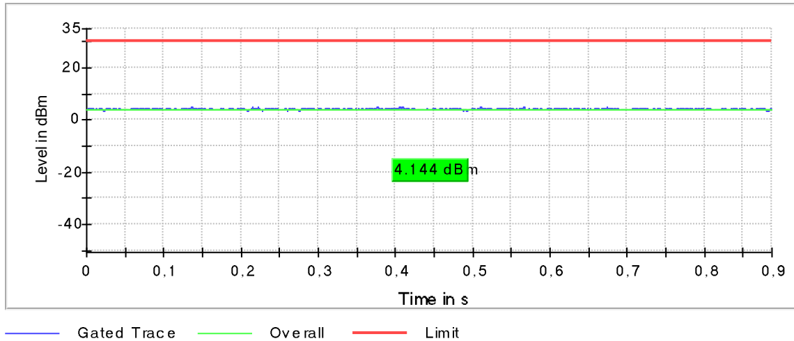
Plot 144: Mode 2, U-NII-3, AVGPM-G Gated Average Power Measurement, low channel
