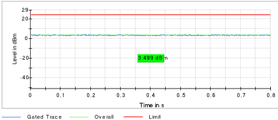
Plot 166: Mode 3, U-NII-2C, AVGPM-G Gated Average Power Measurement, high channel
