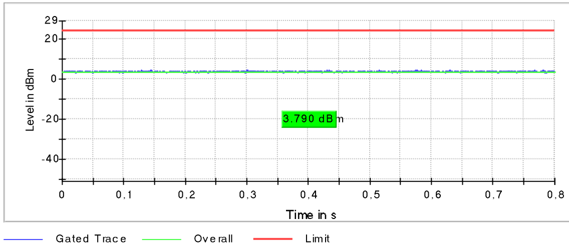
Plot 174: Mode 5, U-NII-2C, AVGP-G Gated Average Power Measurement, mid channel
