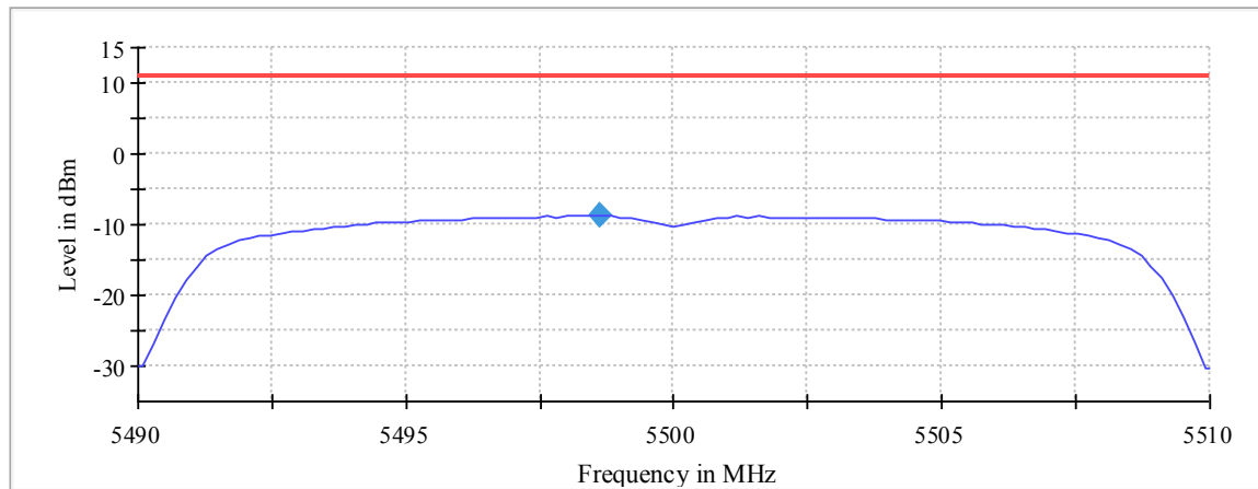
Plot 227: Mode 4, U-NII-2C, Peak PSD, low channel
