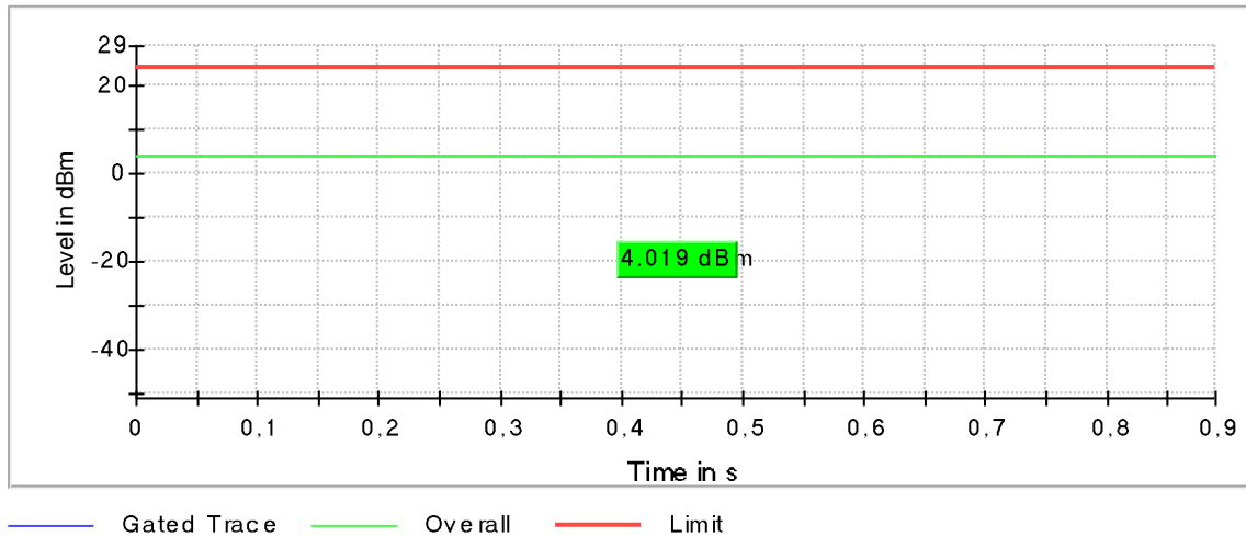
Plot 148: Mode 4, U-NII-1, AVGPm-G Gated Average Power Measurement, mid channel
