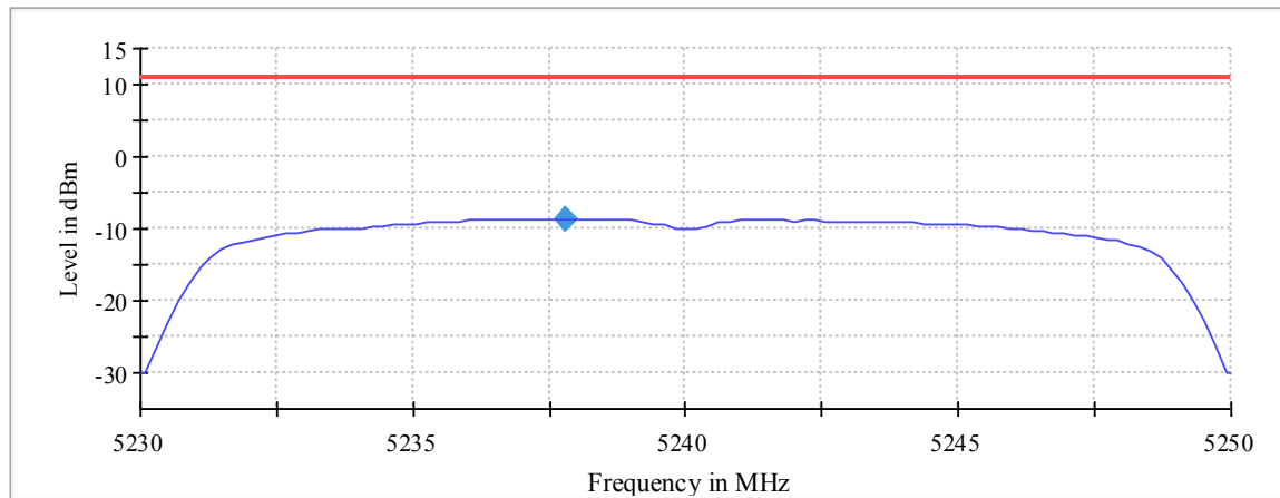
Plot 210: Mode 2, U-NII-1, Peak PSD, high channel
