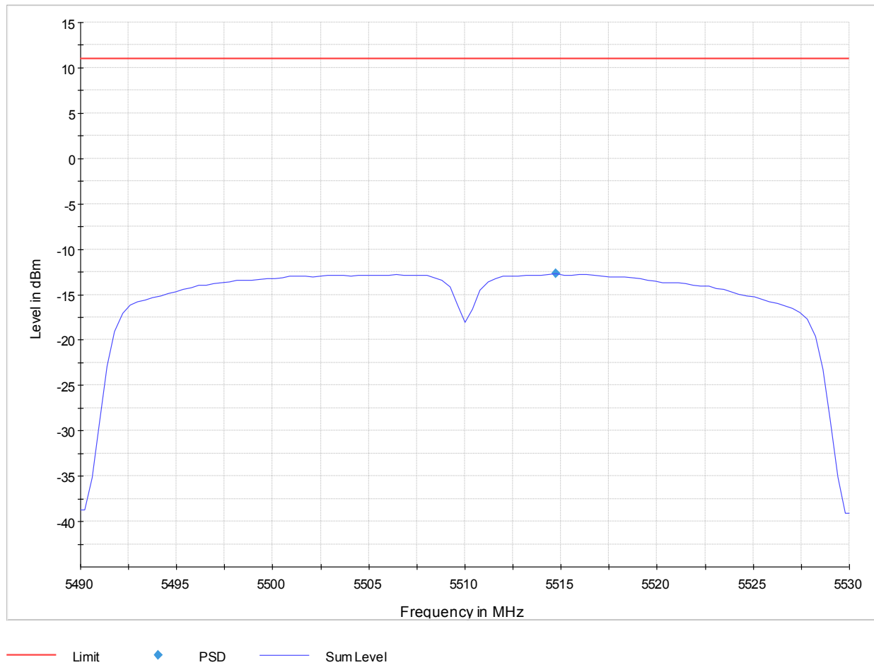
Plot 239: Mode 3, U-NII-2C, Peak PSD, mid channel
