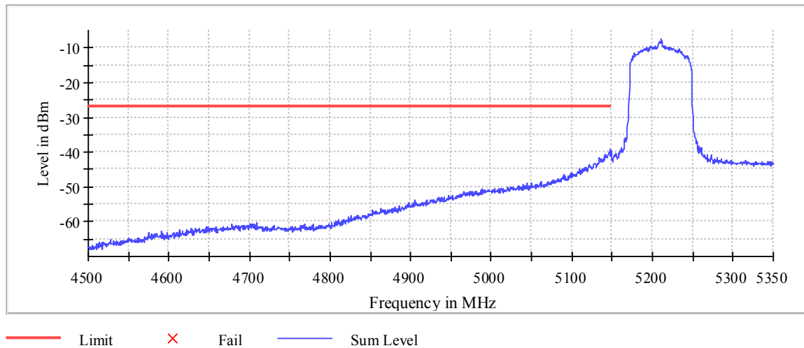
Plot 261: Mode 6, BEC, U-NII-1 & U-NII-2A, low channel, 5210 MHz
