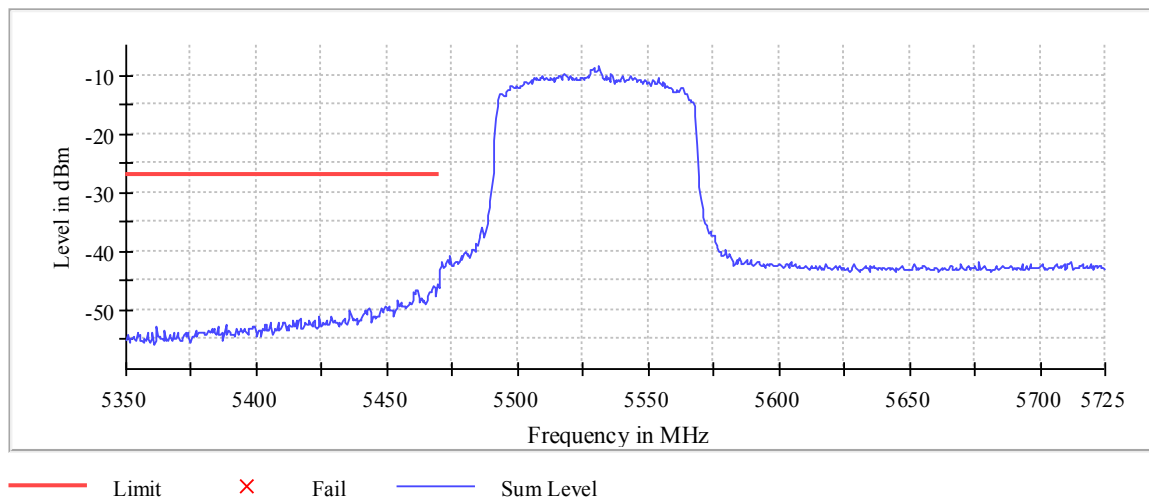
Plot 263: Mode 6, BEC, U-NII-2C, low channel, 5530 MHz
