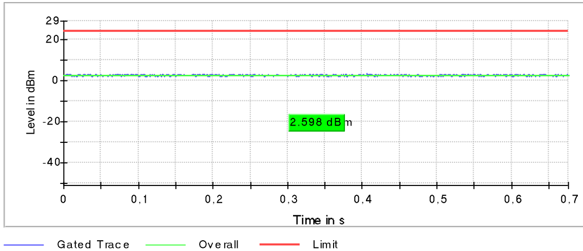
Plot 180: Mode 6, U-NII-2C, AVGP-M-G Gated Average Power Measurement, low channel
