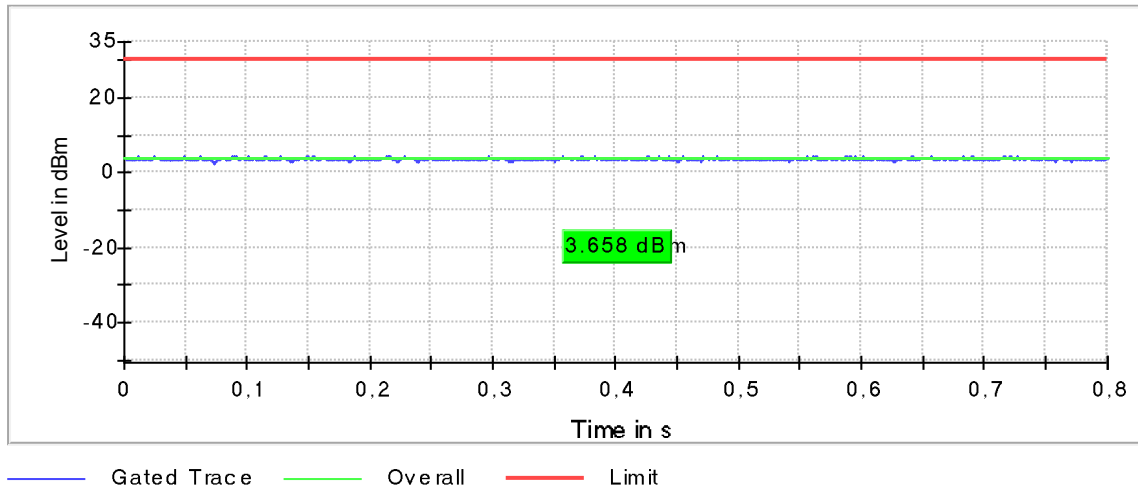
Plot 167: Mode 3, U-NII-3, AVGPM-G Gated Average Power Measurement, low channel
