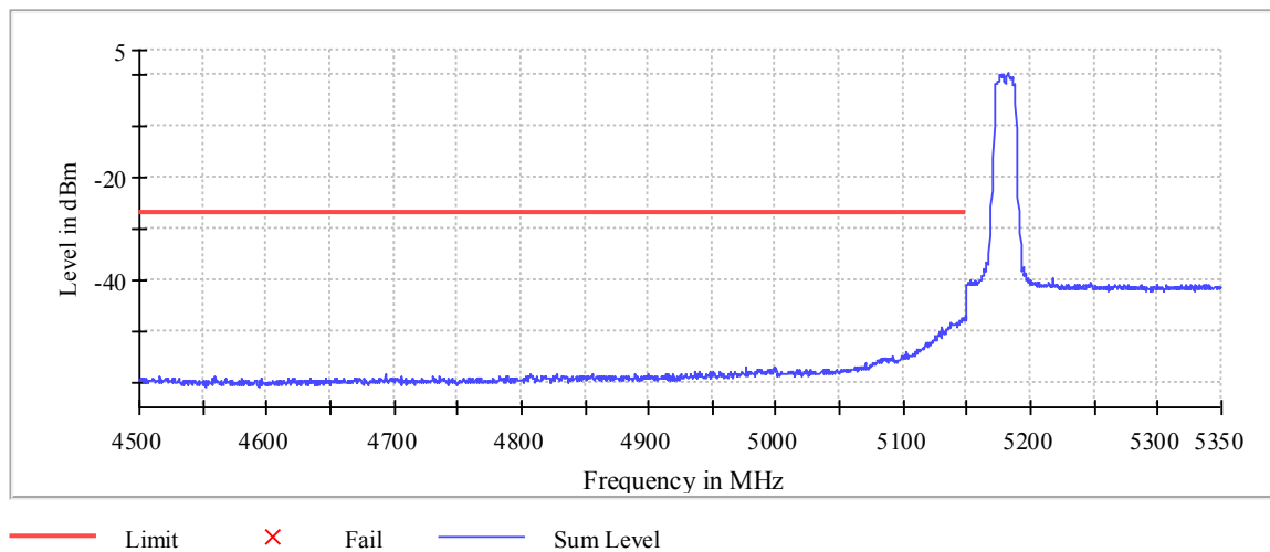
Plot 249: Mode 1, BEC, U-NII-1 & U-NII-2A, low channel, 5180 MHz
