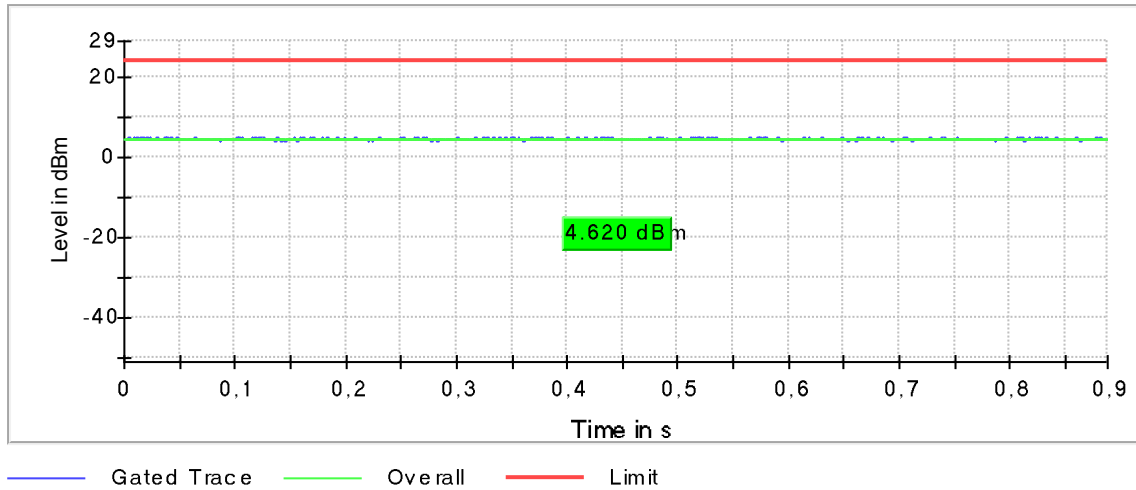
Plot 136: Mode 2, U-NII-1, AVGP-M-G Gated Average Power Measurement, high channel
