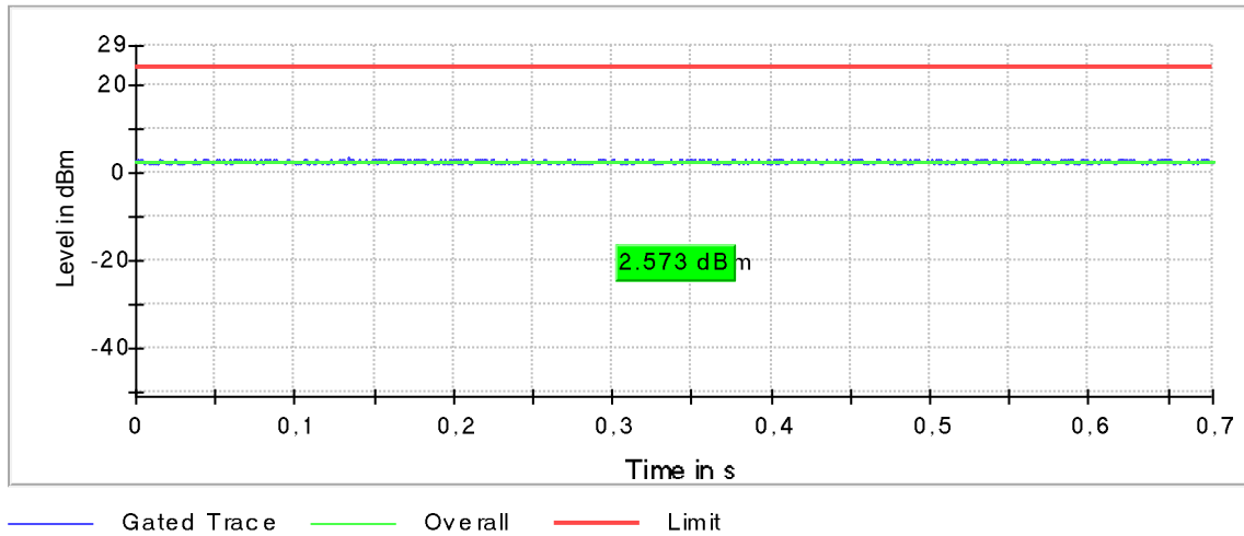
Plot 181: Mode 6, U-NII-2C, AVGP-M-G Gated Average Power Measurement, mid channel
