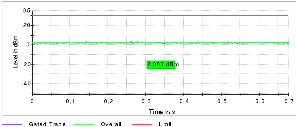
Plot 183: Mode 6, U-NII-3, AVGPM-G Gated Average Power Measurement, mid channel
