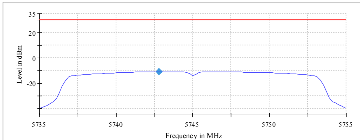
Plot 205: Mode 1, U-NII-3, Peak PSD, low channel
