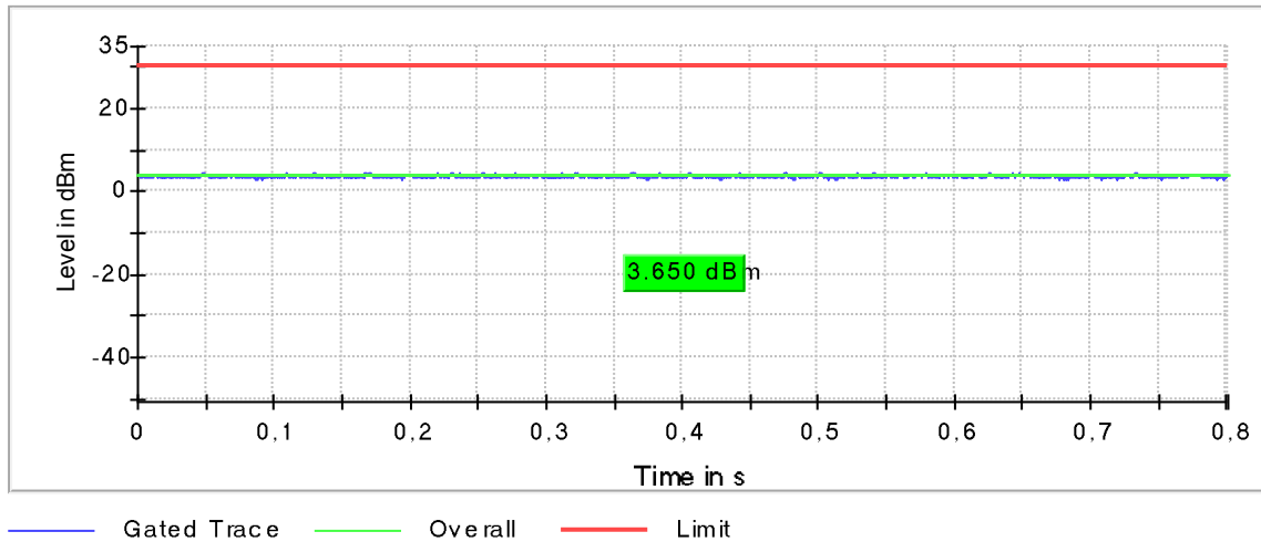
Plot 176: Mode 5, U-NII-3, AVGPM-G Gated Average Power Measurement, low channel
