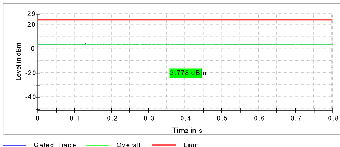
Plot 162: Mode 3, U-NII-2A, AVGP-M-G Gated Average Power Measurement, low channel
