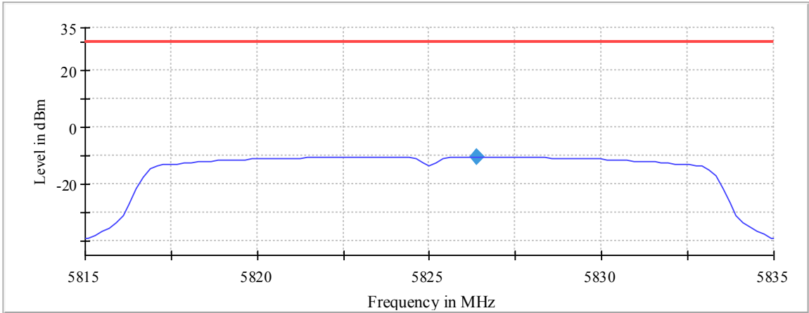
Plot 207: Mode 1, U-NII-3, Peak PSD, high channel
