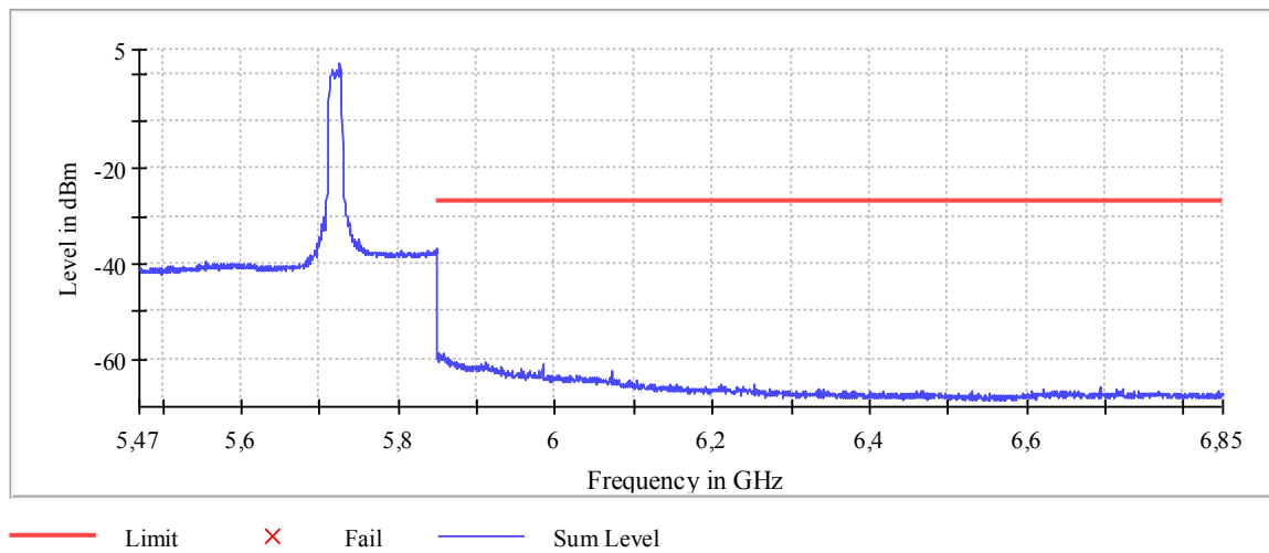
Plot 252: Mode 1, BEC, U-NII-2C, high channel
