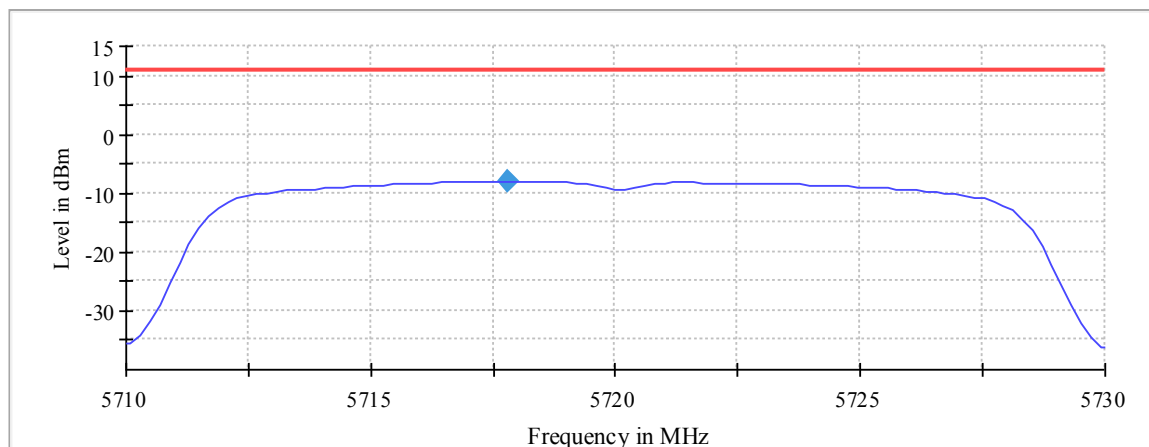
Plot 204: Mode 1, U-NII-2C, Peak PSD, channel 144
