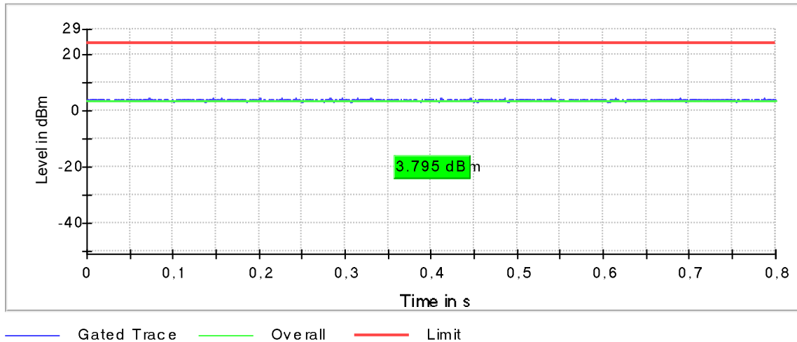
Plot 165: Mode 3, U-NII-2C, AVGP-M-G Gated Average Power Measurement, mid channel
