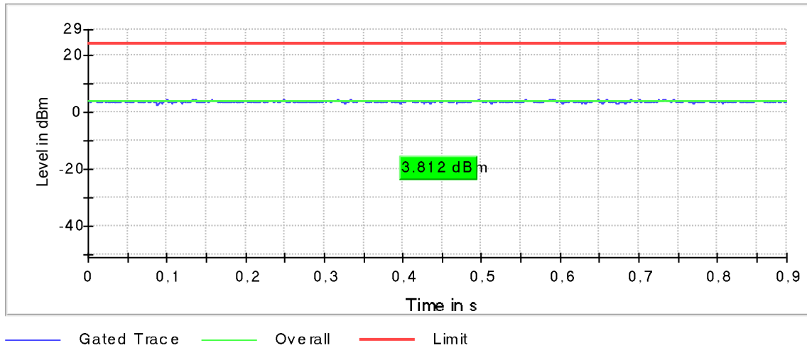
Plot 143: Mode 2, U-NII-2C, AVGP-M-G Gated Average Power Measurement, channel 144
