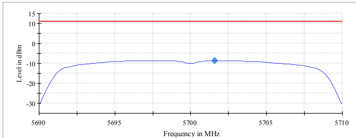
Plot 229: Mode 4, U-NII-2C, Peak PSD, high channel
