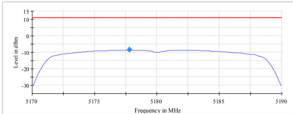
Plot 221: Mode 4, U-NII-1, Peak PSD, low channel
