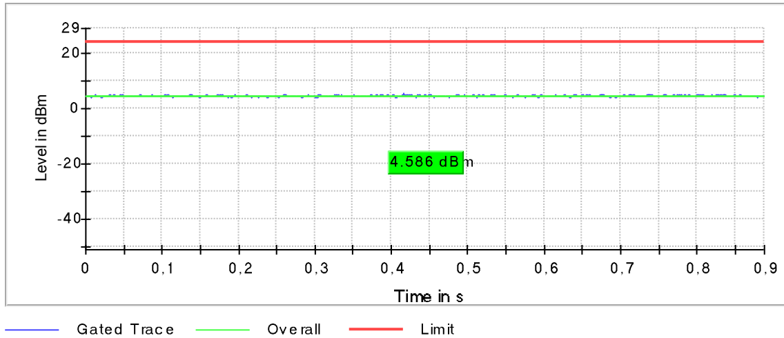
Plot 149: Mode 4, U-NII-1, AVGPm-G Gated Average Power Measurement, high channel
