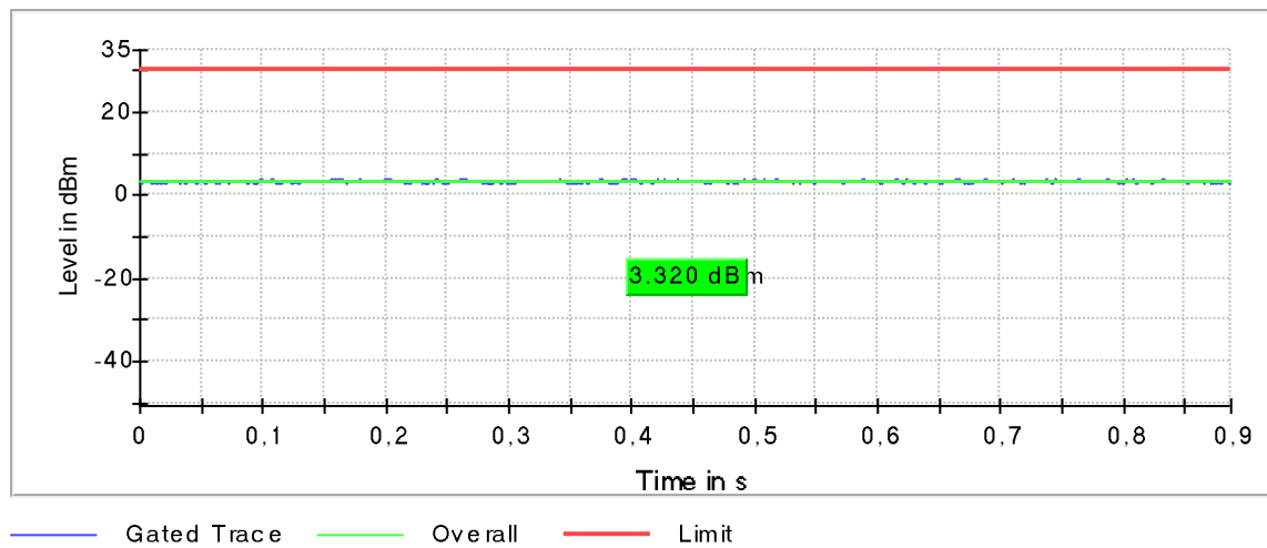
Plot 159: Mode 4, U-NII-3, AVGPM-G Gated Average Power Measurement, high channel
