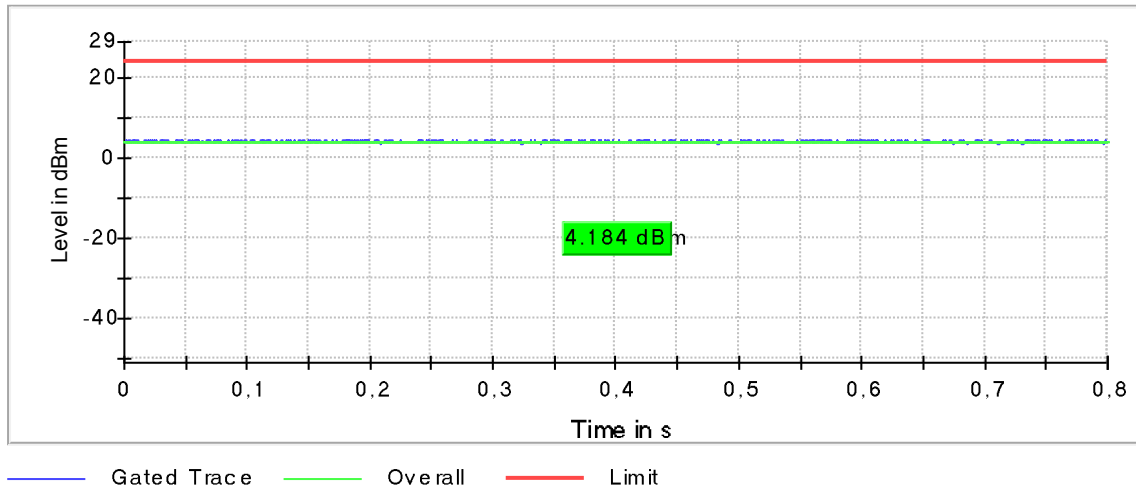
Plot 172: Mode 5, U-NII-2A, AVGP-M-G Gated Average Power Measurement, high channel
