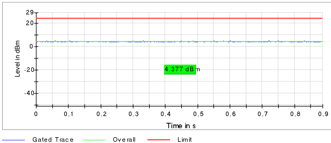
Plot 152: Mode 4, U-NII-2A, AVGPM-G Gated Average Power Measurement, high channel
