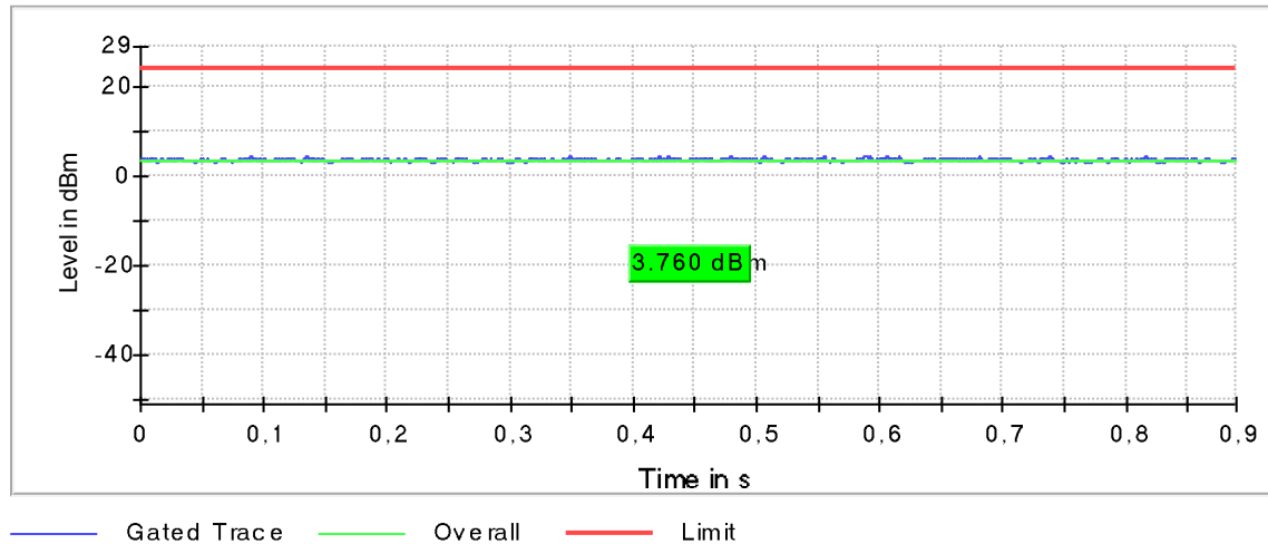
Plot 156: Mode 4, U-NII-2C, AVGP-M-G Gated Average Power Measurement, channel 144
