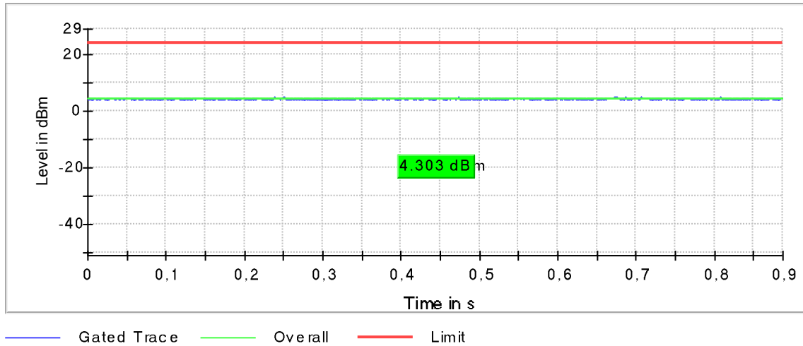
Plot 138: Mode 2, U-NII-2A, AVGP-M-G Gated Average Power Measurement, mid channel
