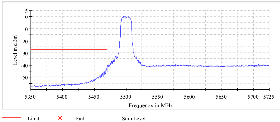
Plot 251: Mode 1, BEC, U-NII-2C, low channel
