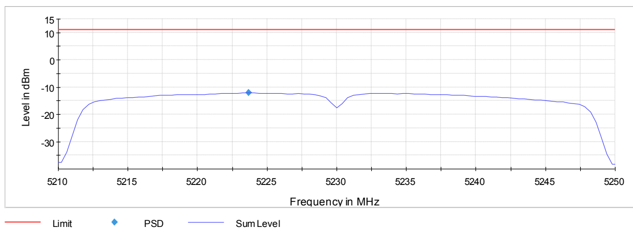
Plot 235: Mode 3, U-NII-1, Peak PSD, high channel
