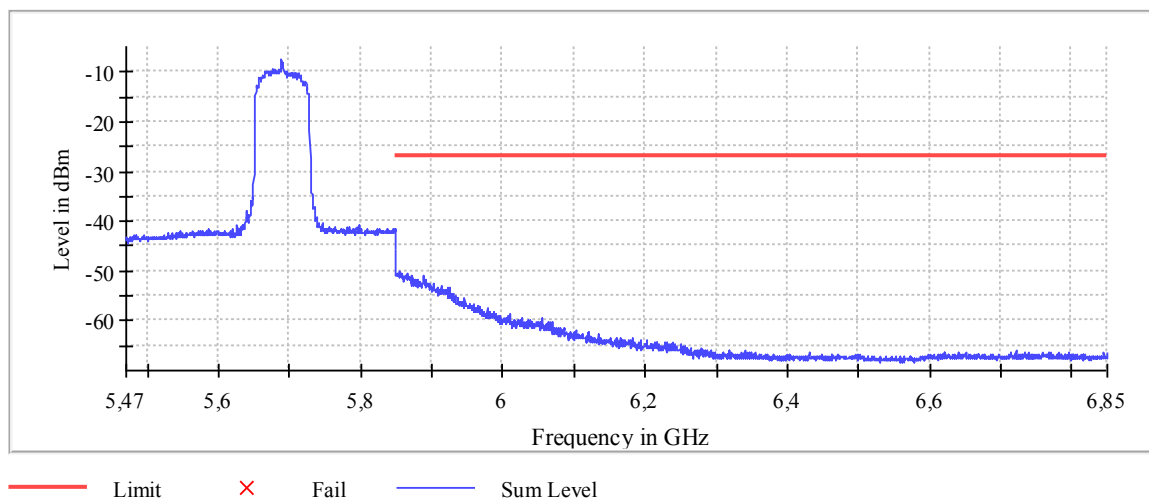
Plot 264: Mode 6, BEC, U-NII-2C, high channel, 5690
