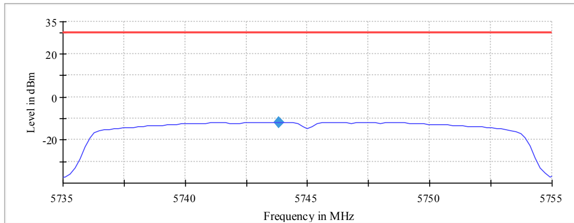
Plot 218: Mode 2, U-NII-3, Peak PSD, low channel
