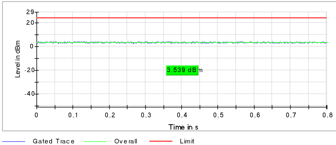
Plot 175: Mode 5, U-NII-2C, AVGPM-G Gated Average Power Measurement, high channel
