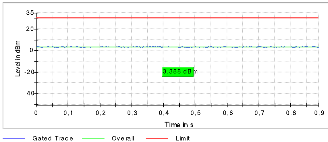
Plot 146: Mode 2, U-NII-3, AVGPM-G Gated Average Power Measurement, high channel
