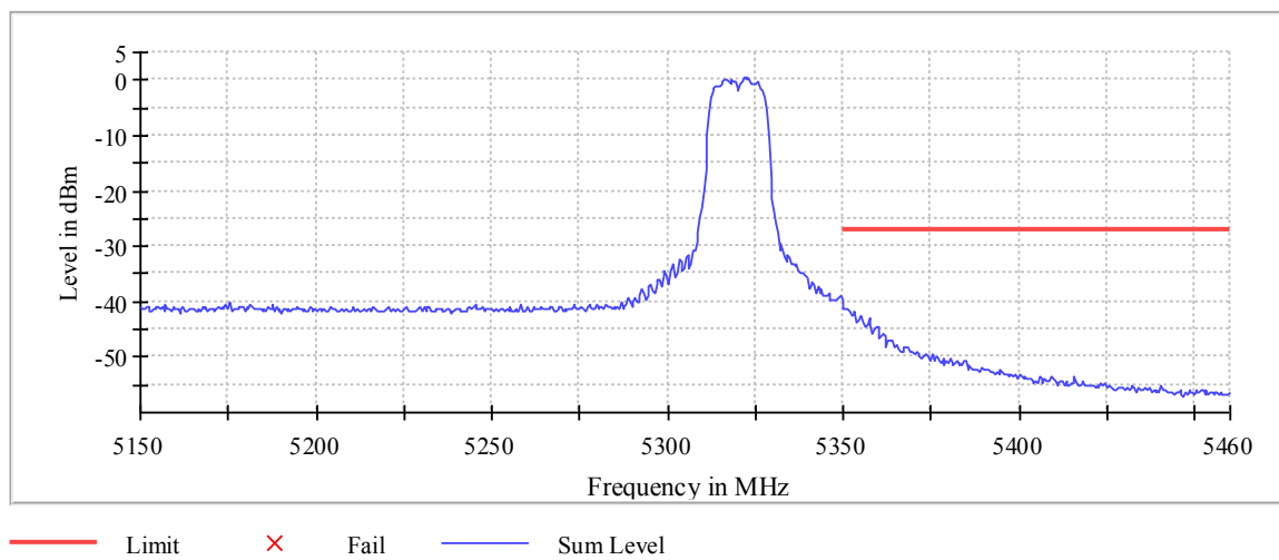
Plot 250: Mode 1, BEC, U-NII-1 & U-NII-2A, high channel, 5320 MHz
