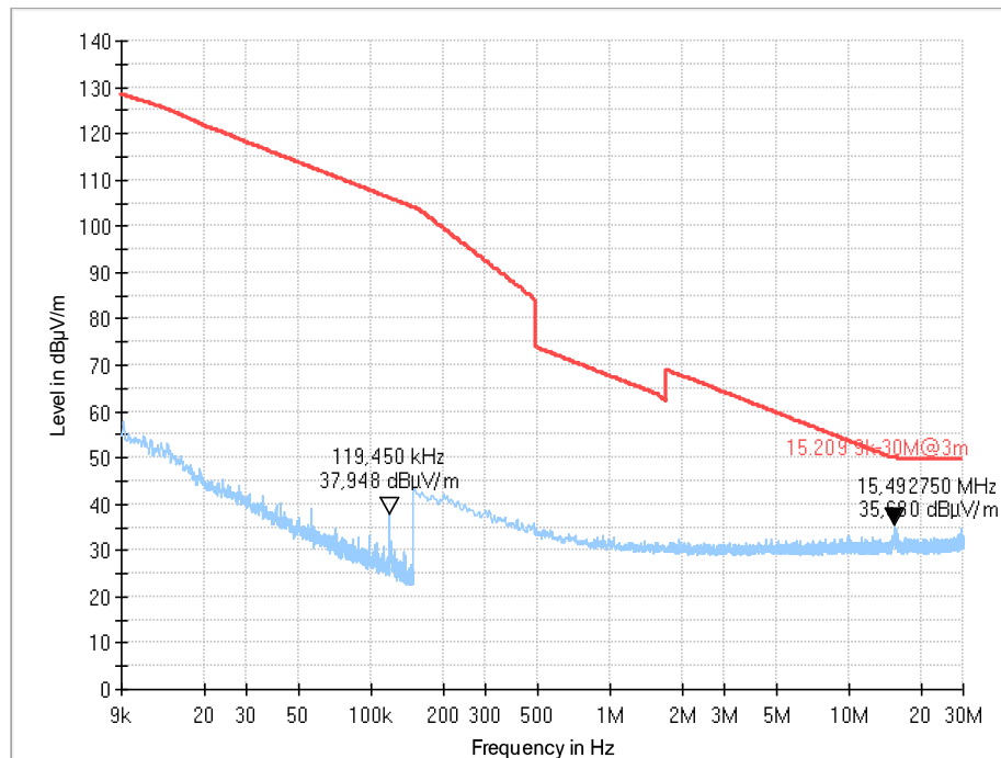
Plot 313: Mode 1, RSE 9 kHz – 30 MHz, channel 144, loop antenna (EUT laying)
