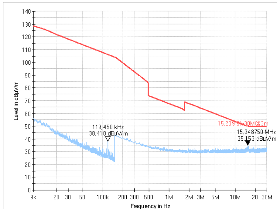
Plot 305: Mode 1, RSE 9 kHz – 30 MHz, channel 64, loop antenna (EUT laying)
