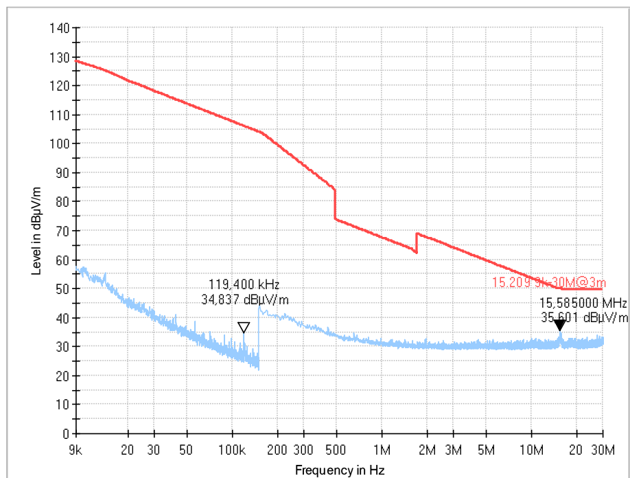
Plot 304: Mode 1, RSE 9 kHz – 30 MHz, channel 52, loop antenna (EUT standing)
