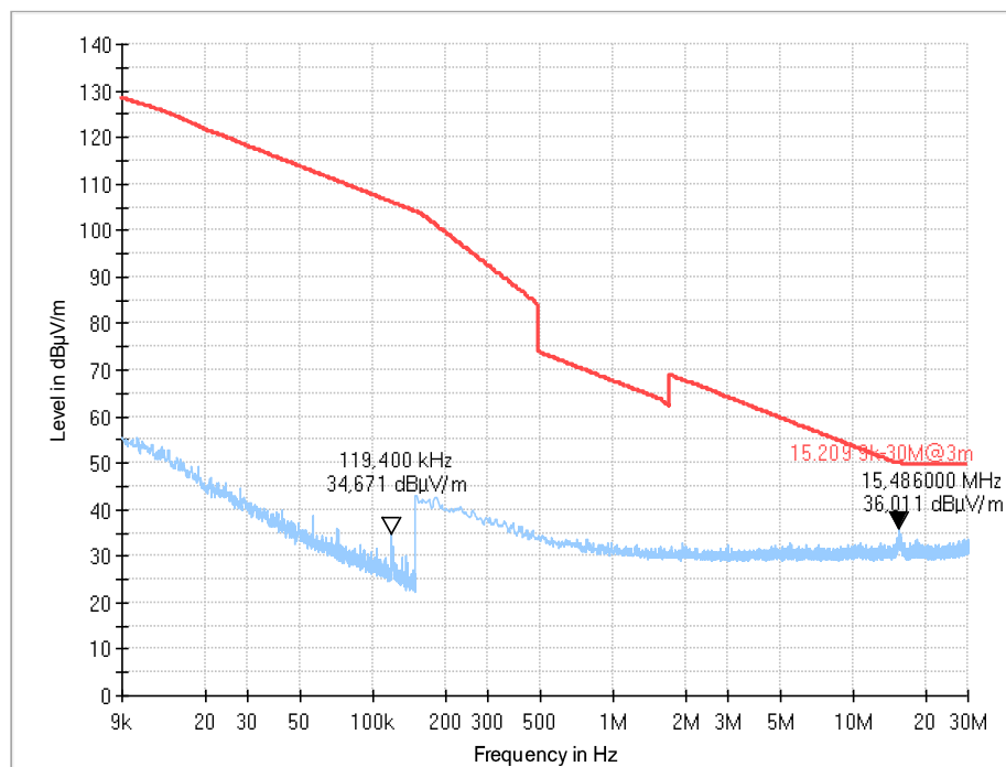
Plot 316: Mode 1, RSE 9 kHz – 30 MHz, channel 149, loop antenna (EUT standing)
