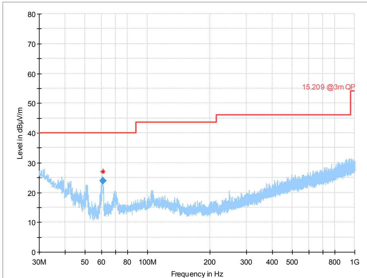
Plot 48: Mode 1, RSE 30 MHz – 1 GHz, high channel, horizontal / vertical polarisation
