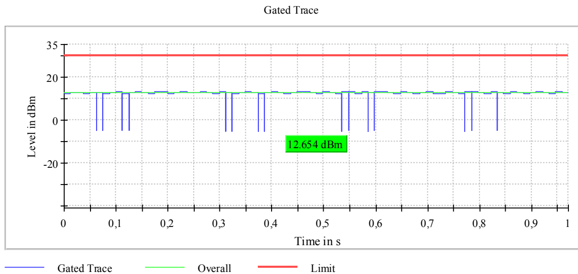
Plot 34: Mode 1, AVGPM-G Gated Average Power Measurement, high channel
