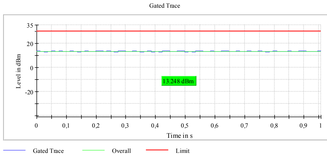
Plot 3: Mode 1, AVGPM-G Gated Average Power Measurement, high channel
