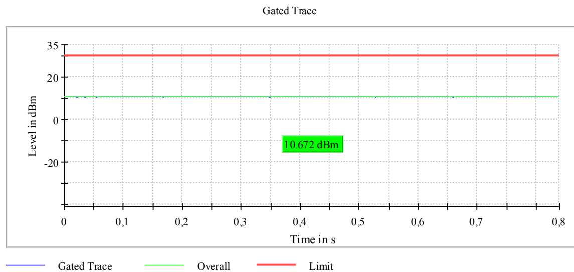
Plot 8: Mode 3, AVGPM-G Gated Average Power Measurement, mid channel
