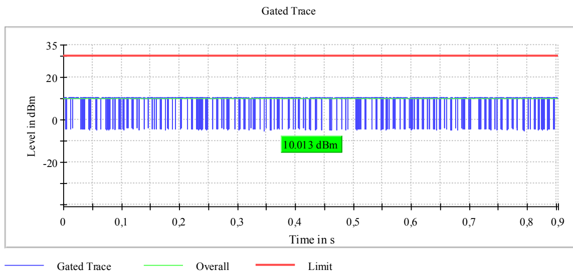
Plot 39: Mode 3, AVGPM-G Gated Average Power Measurement, mid channel
