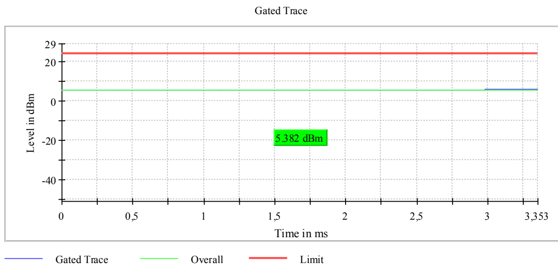
Plot 7: Mode 1, U-NII-2C, AVGPM-G Gated Average Power Measurement, low channel
