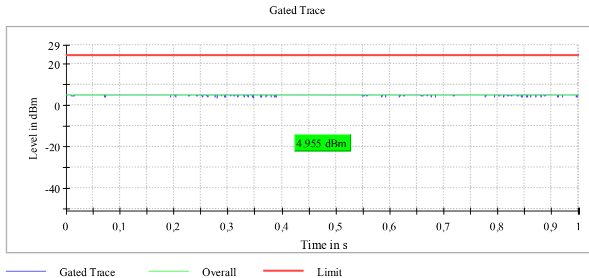
Plot 45: Mode 1, U-NII-1, AVGP-M-G Gated Average Power Measurement, high channel
