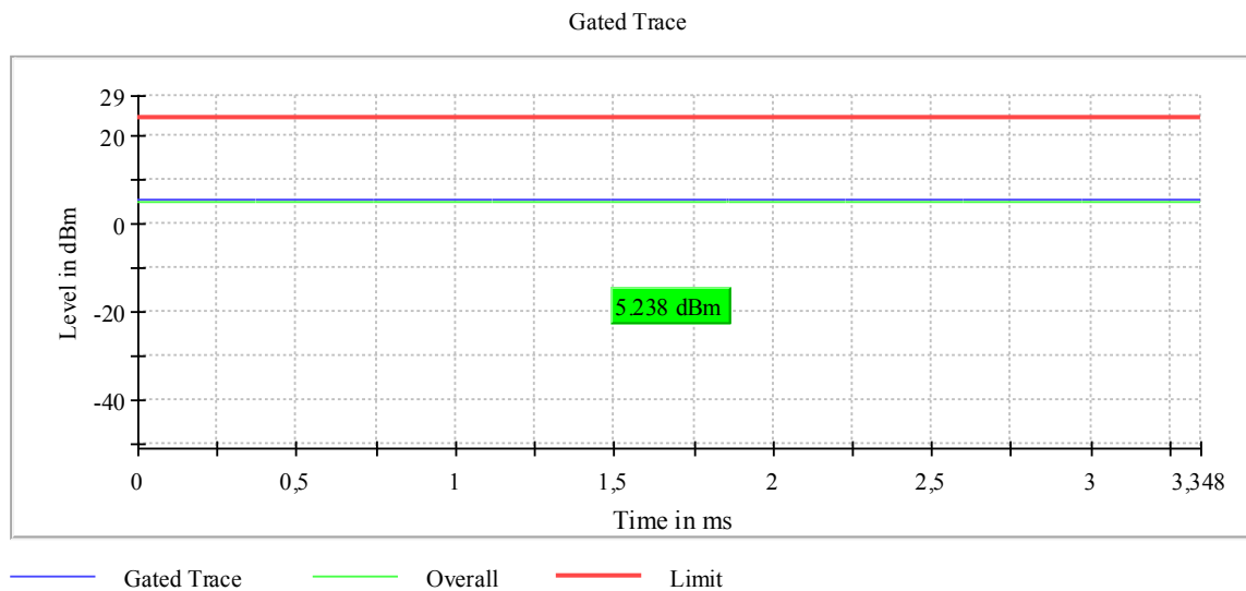
Plot 5: Mode 1, U-NII-2A, AVGP-M-G Gated Average Power Measurement, mid channel
