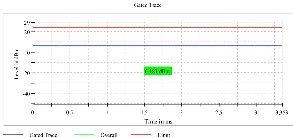
Plot 9: Mode 1, U-NII-2C, AVGP-M-G Gated Average Power Measurement, high channel
