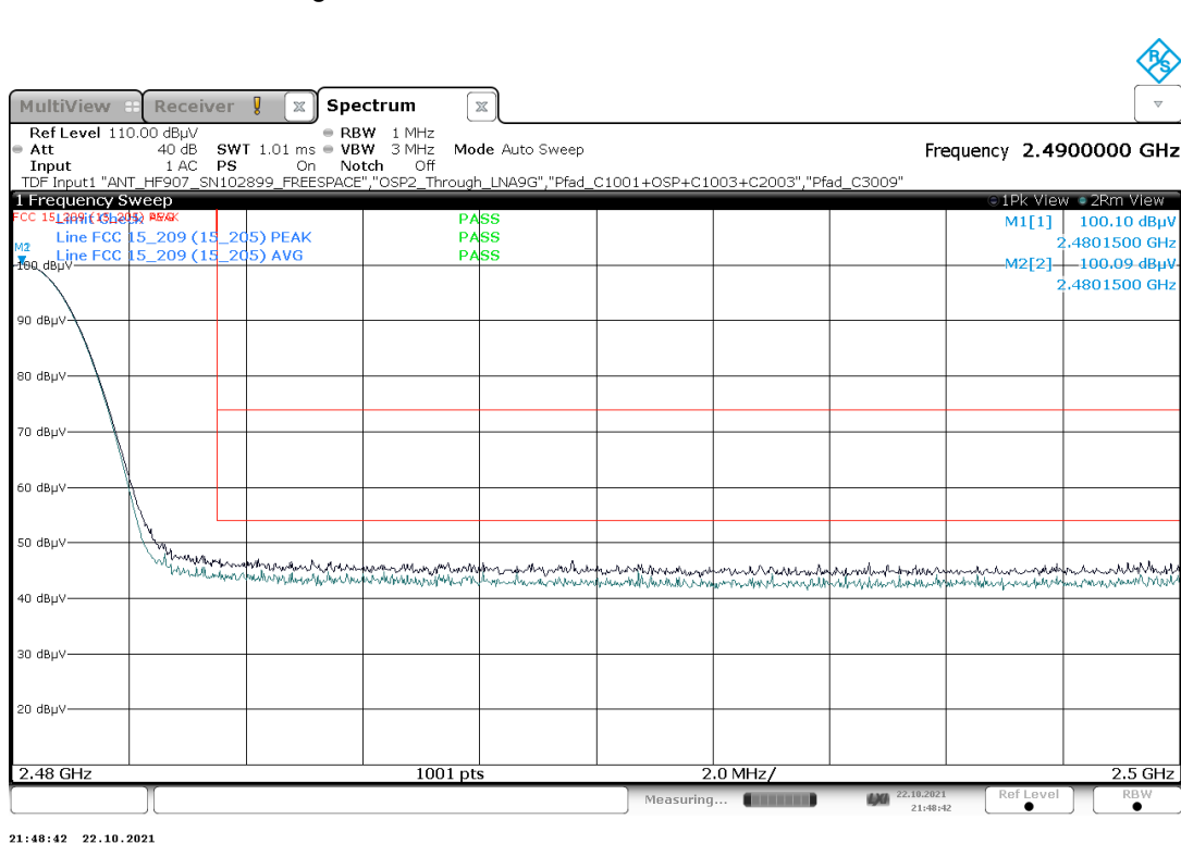
Plot 7: Mode 1, BEC, high channel 39, 2480 MHz
