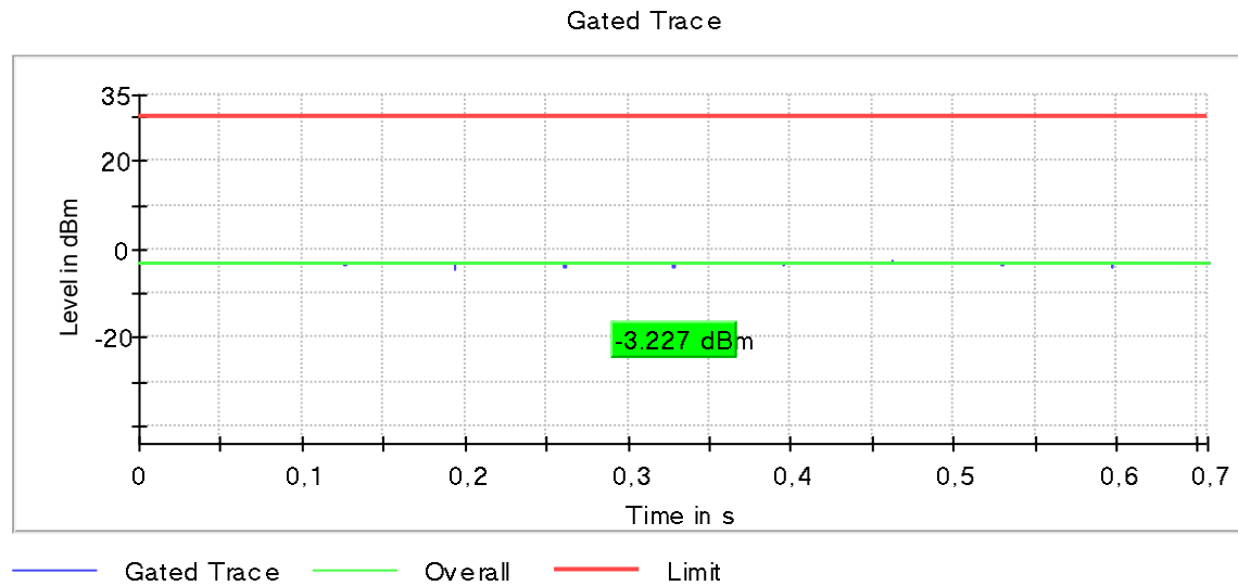
Plot 12: Test Mode 1, GFSK, 1 Mbit/s, RF output power, high channel 39, 2480 MHz
