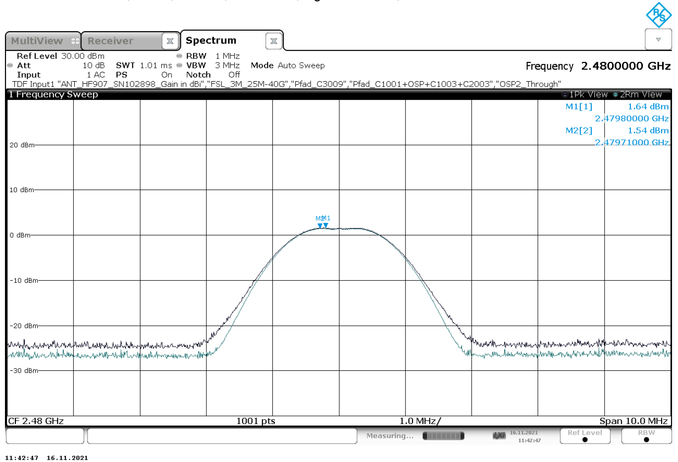
Plot 14: Test Mode 1, GFSK, 1 Mbit/s, Peak EIRP, high channel 39, 2480 MHz
