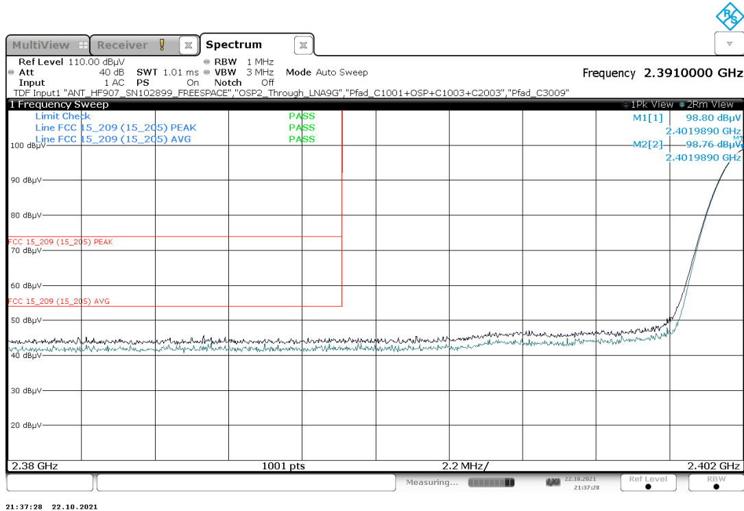
Plot 6: Mode 1, BEC, low channel 37, 2402 MHz
