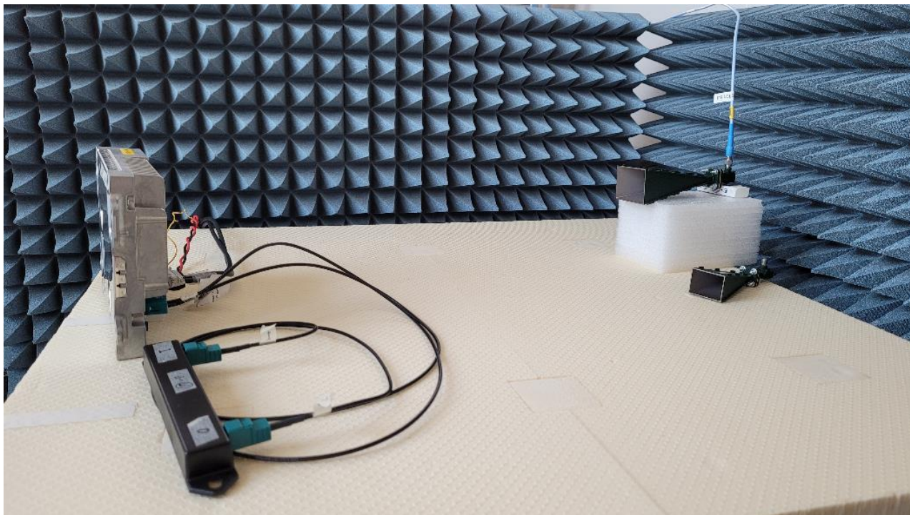
Photo No. 36: Test set-up 8.3
