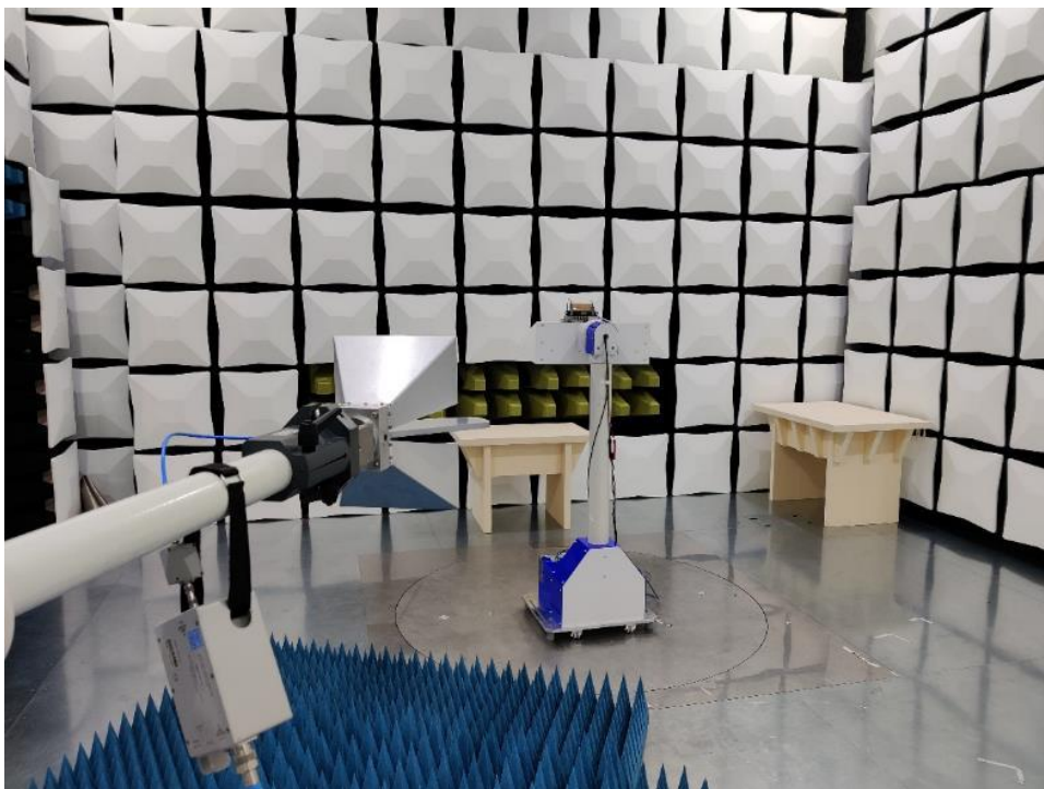
Photo No. 33: Test set-up 8.2, test antenna view
