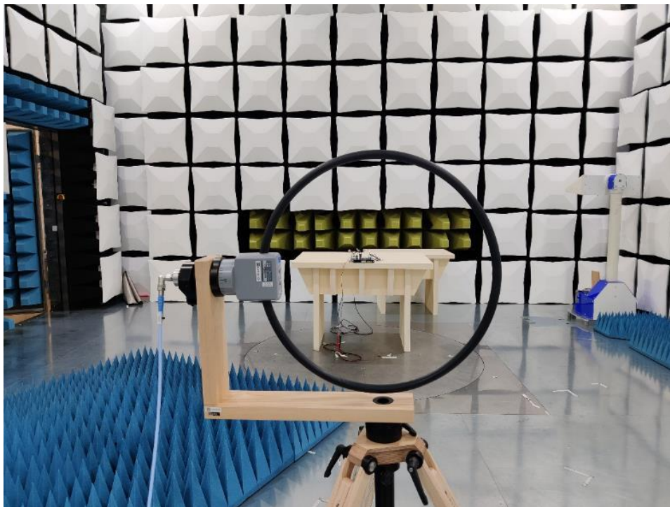
Photo No. 35: Test set-up 8.1, test antenna view
