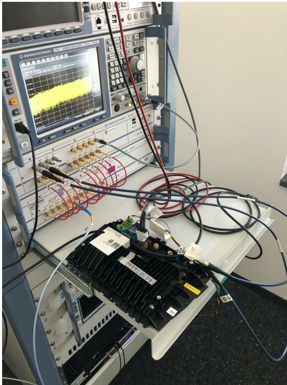
Photo No. 37: test set-up 8.4 with R1LOW-R connected with TS8997
