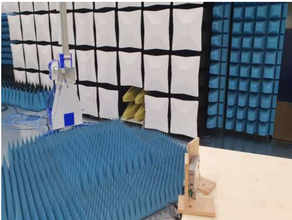
Photograph 2: Radiated emission 1...18 GHz
