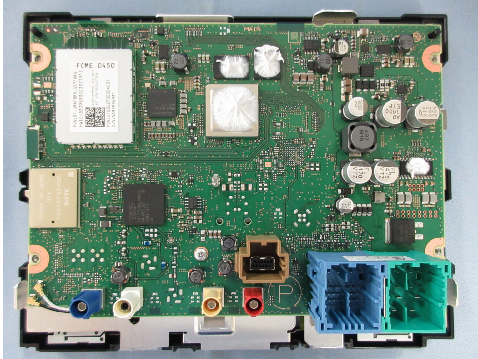
PCB-MAIN C-side
