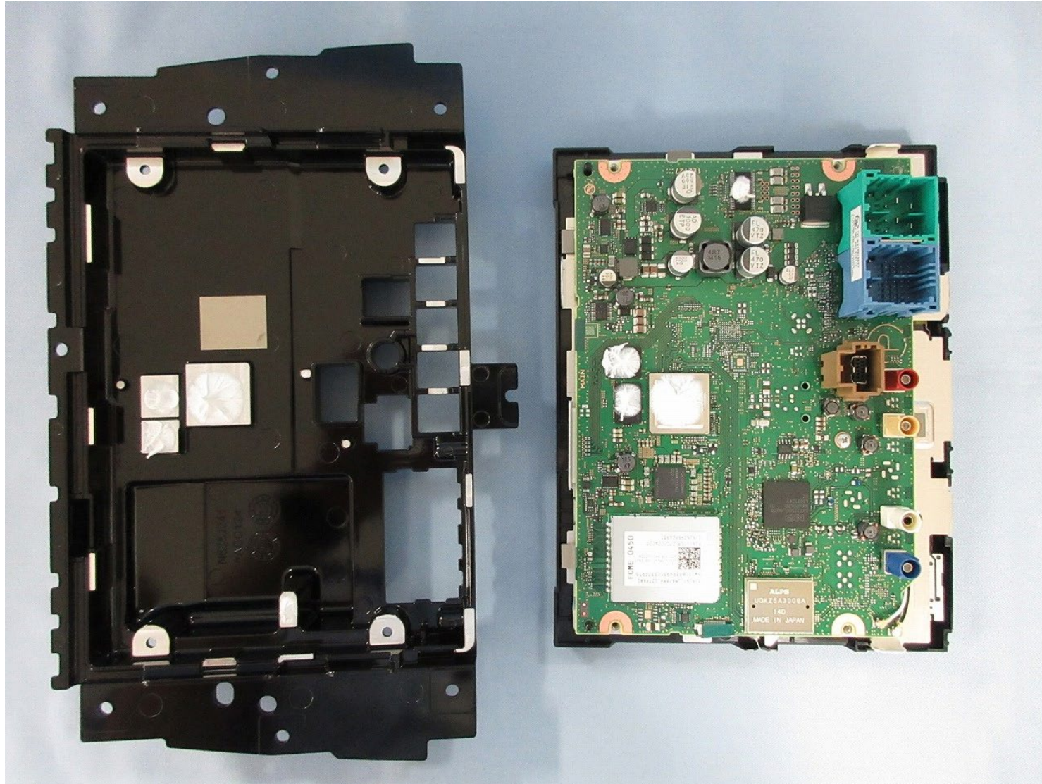
PCB-MAIN C-side
