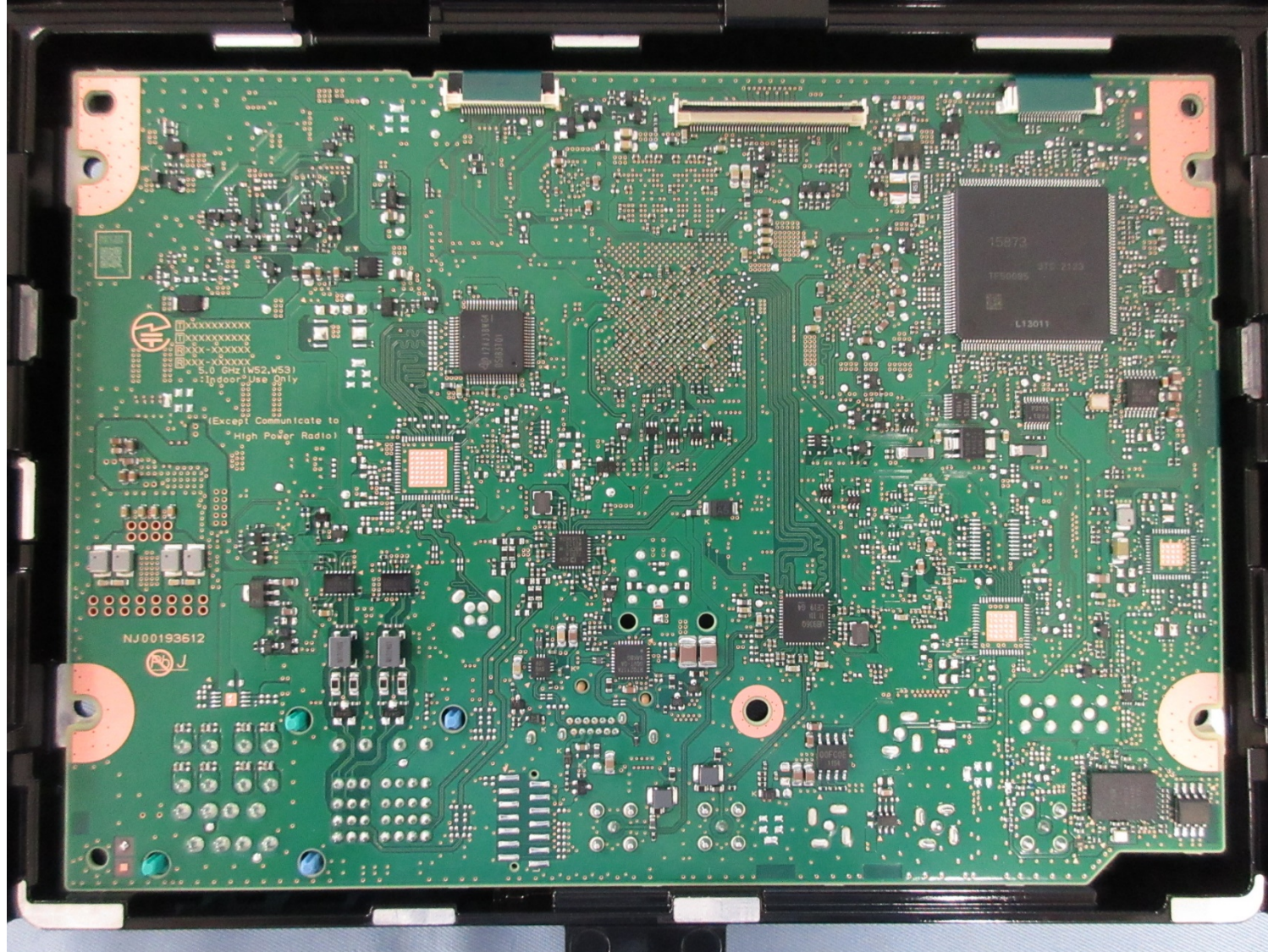
PCB-MAIN S-side
