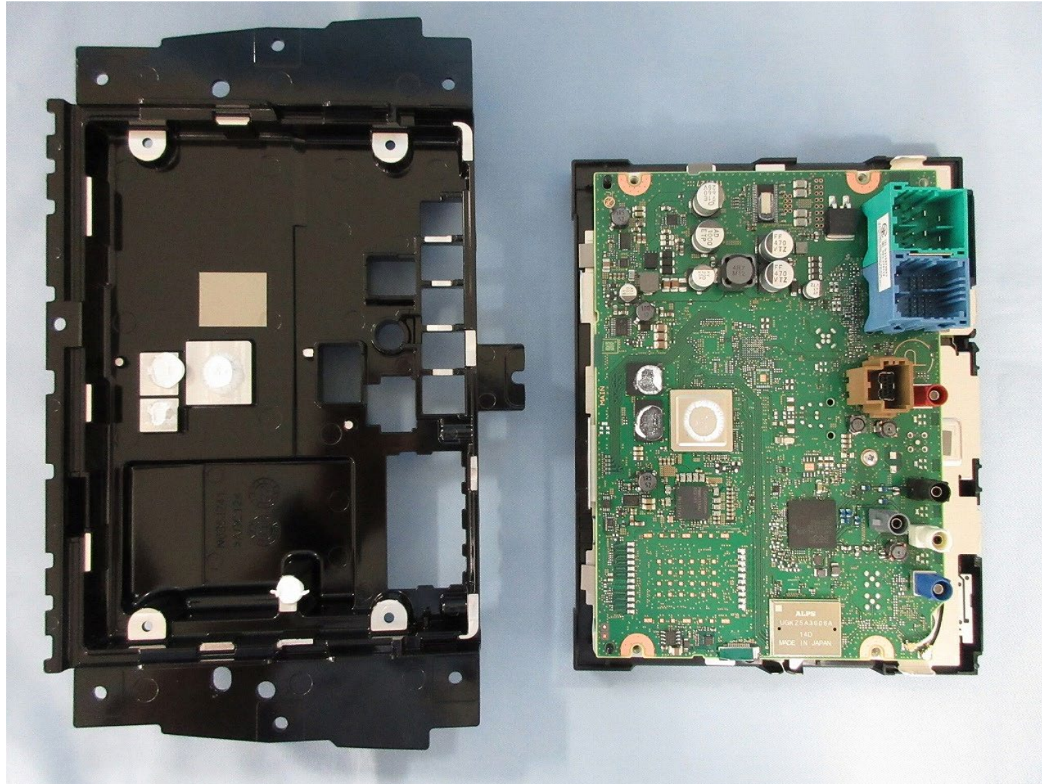
PCB-MAIN C-side
