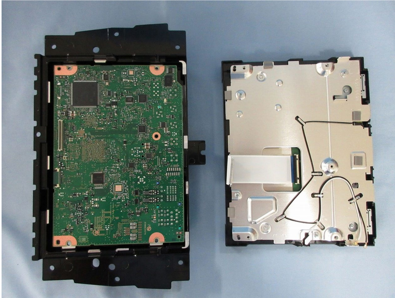
PCB-MAIN S-side
