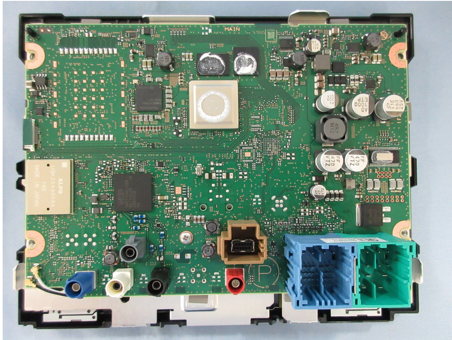
PCB-MAIN C-side
