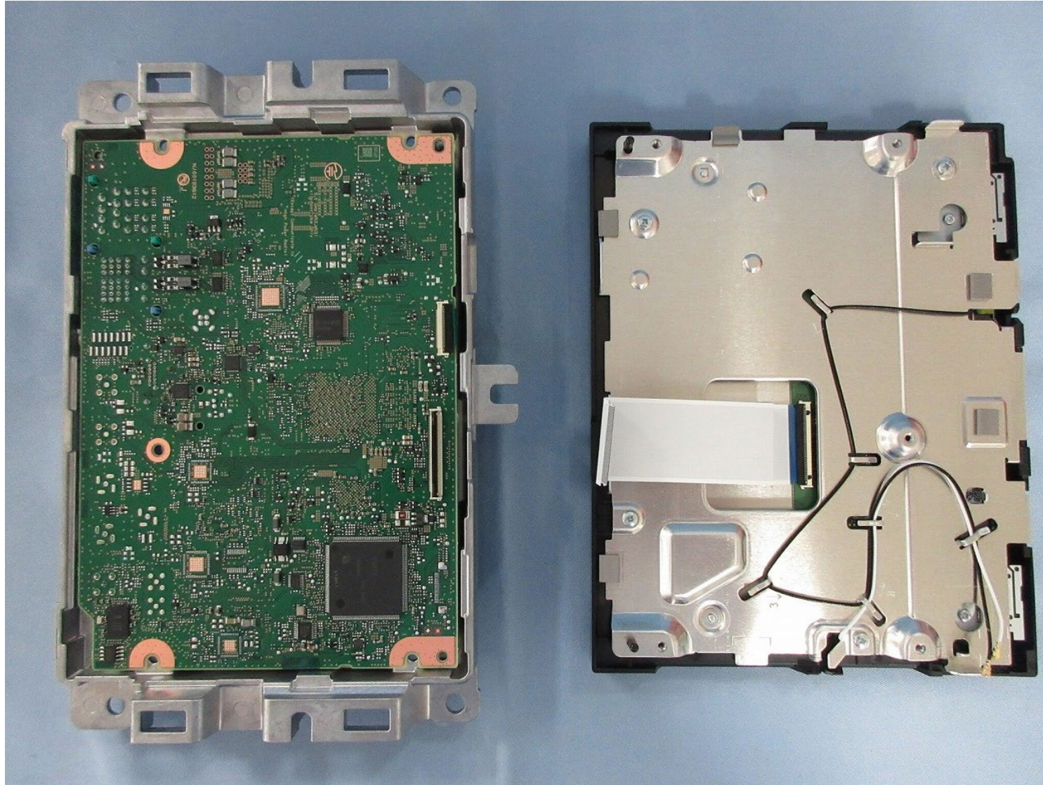
PCB-MAIN S-side
