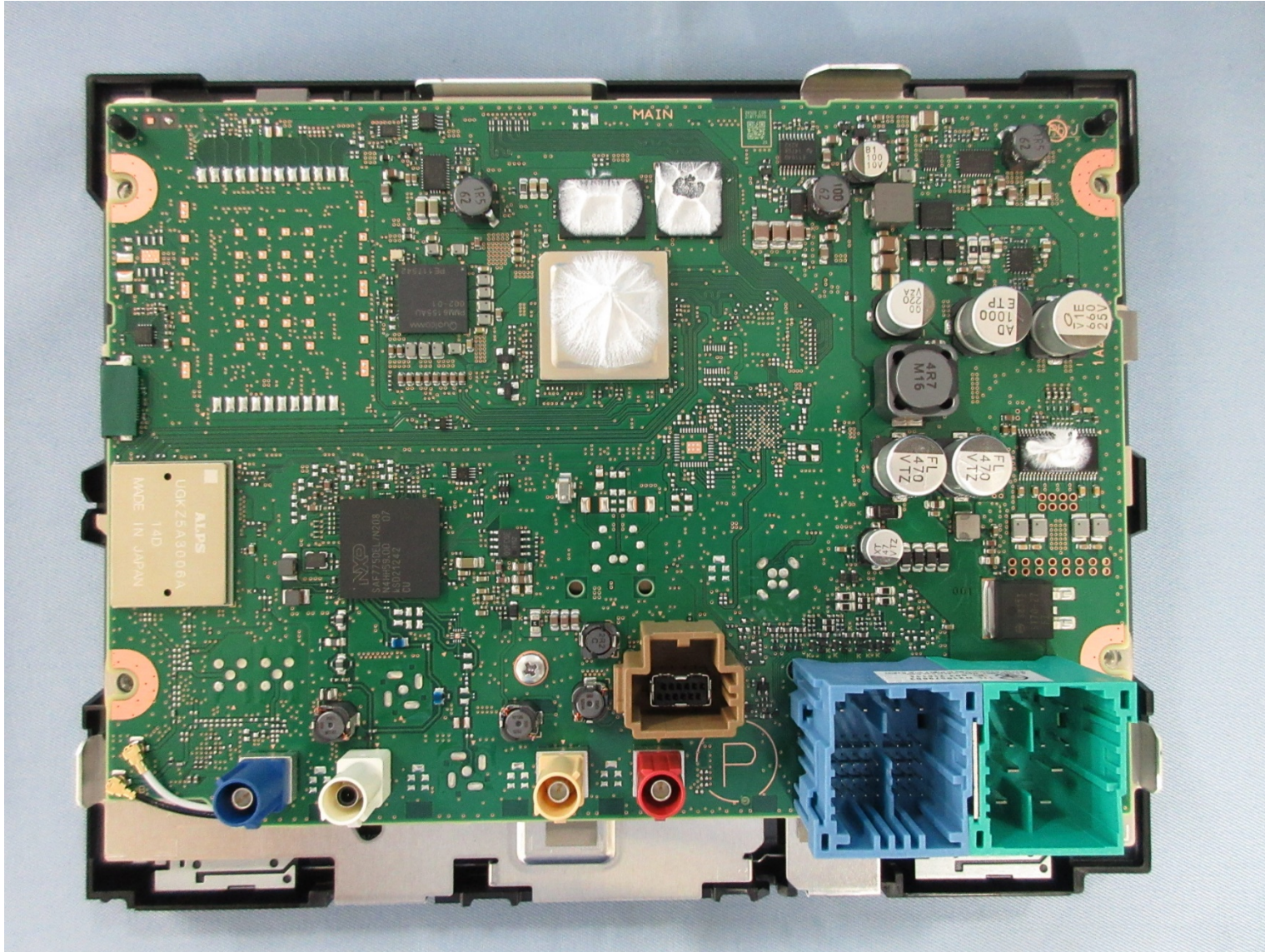
PCB-MAIN C-side
