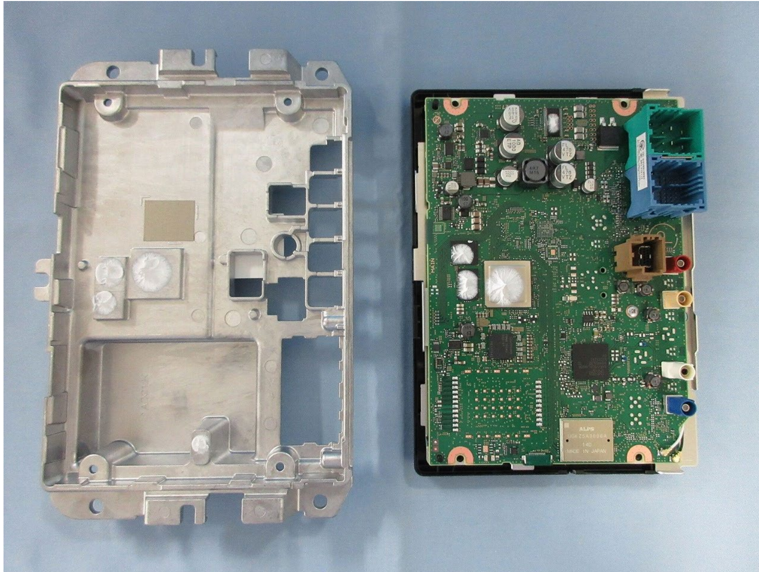
PCB-MAIN C-side
