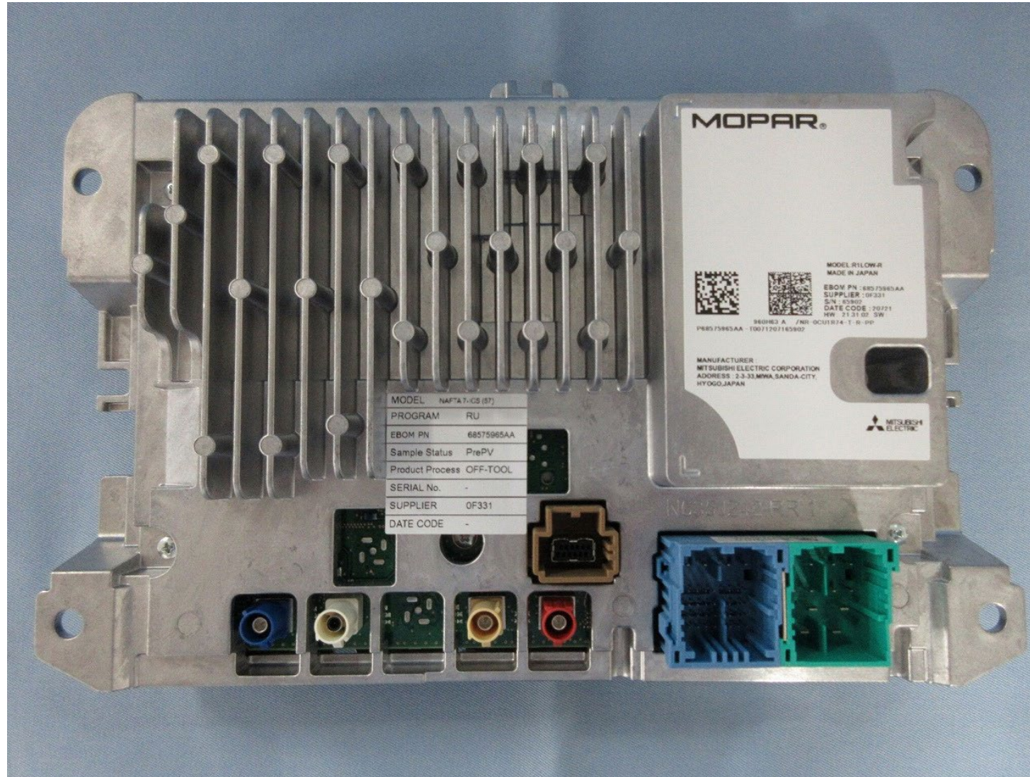
Rear side
