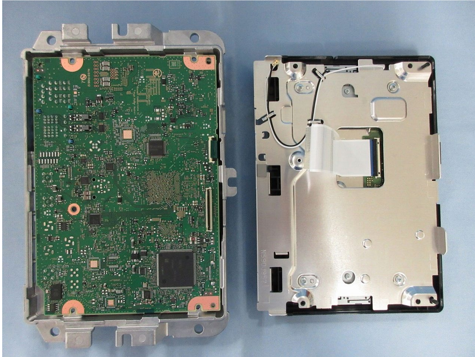
PCB-MAIN S-side
