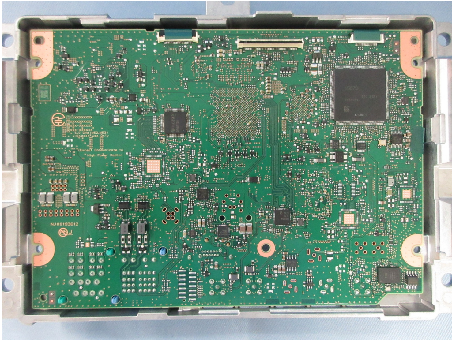
PCB-MAIN S-side
