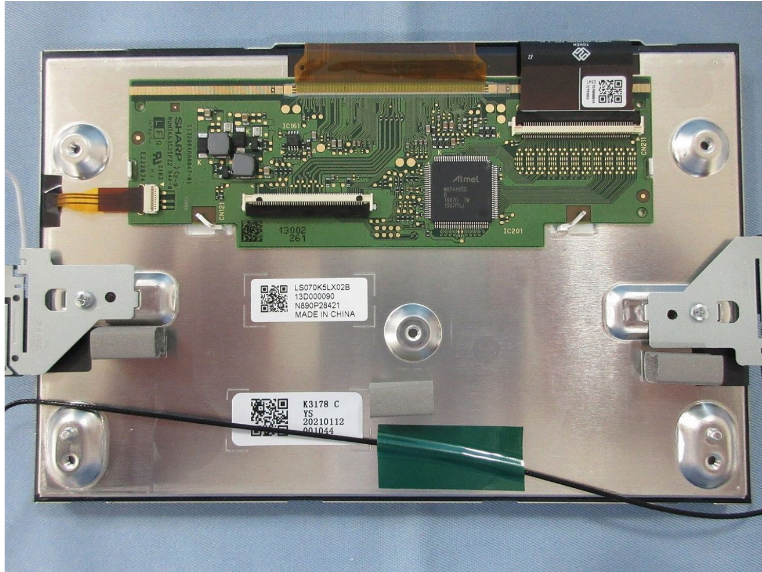
Rear side
