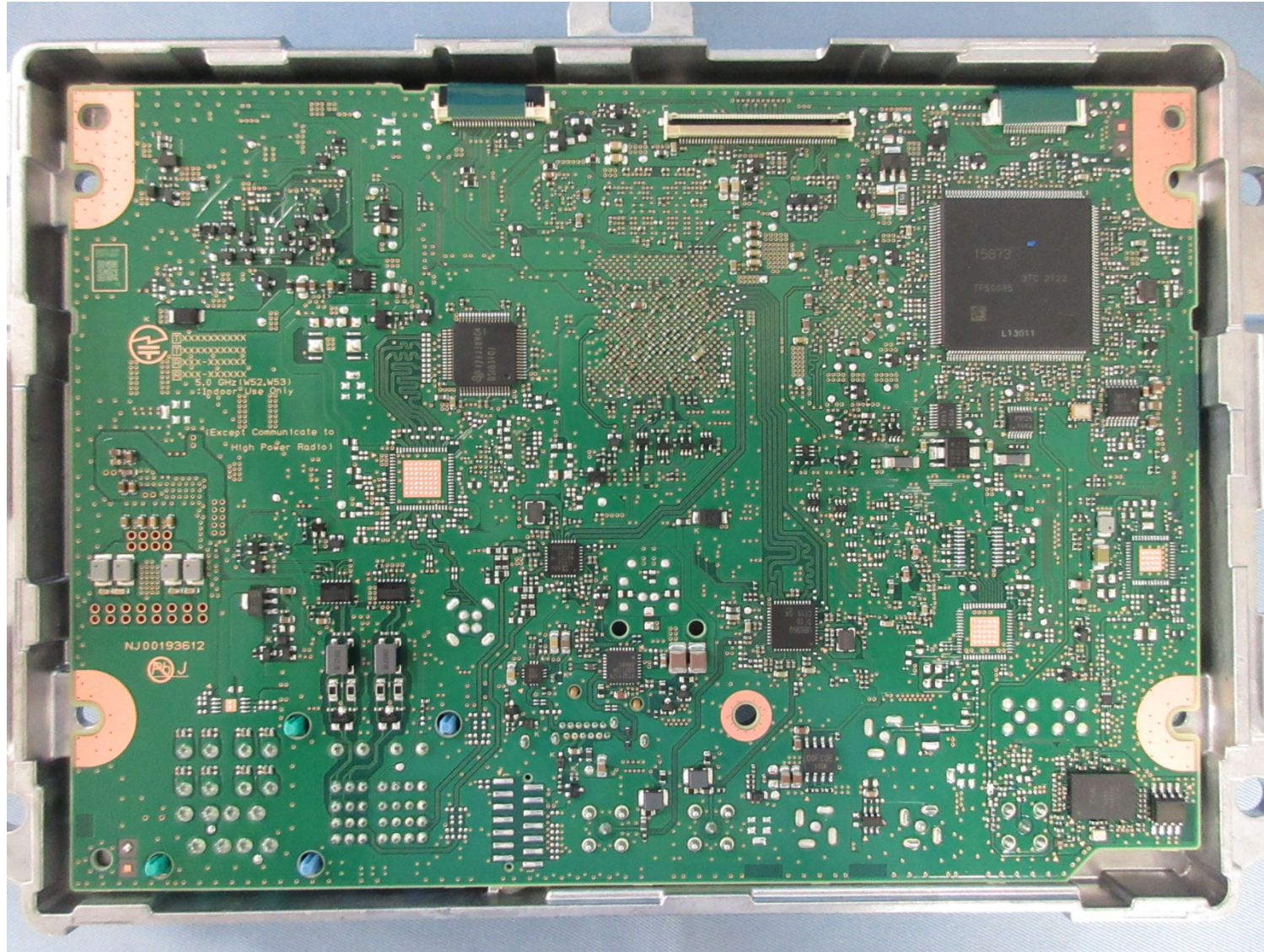
PCB-MAIN S-side
