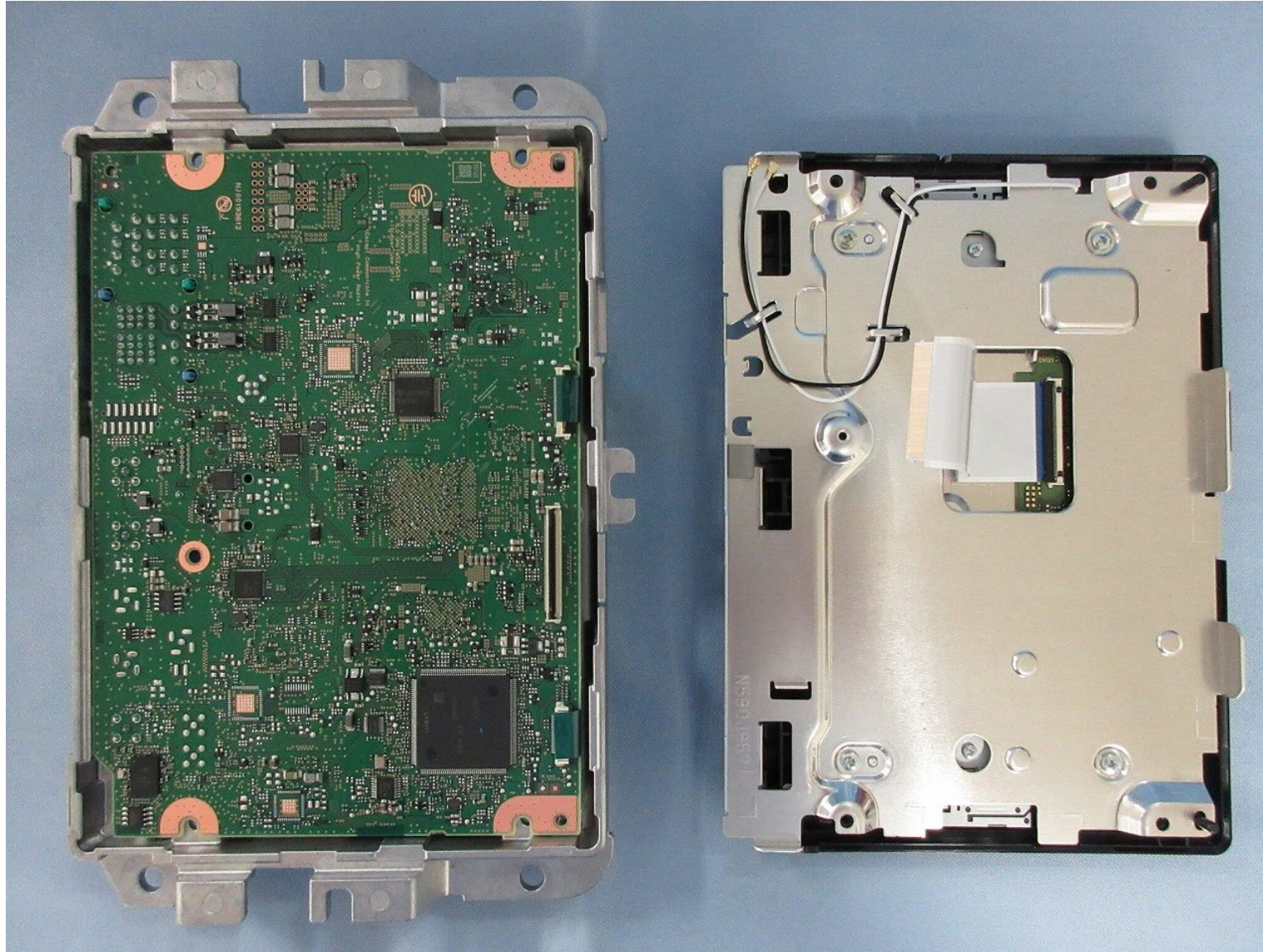
PCB-MAIN S-side
