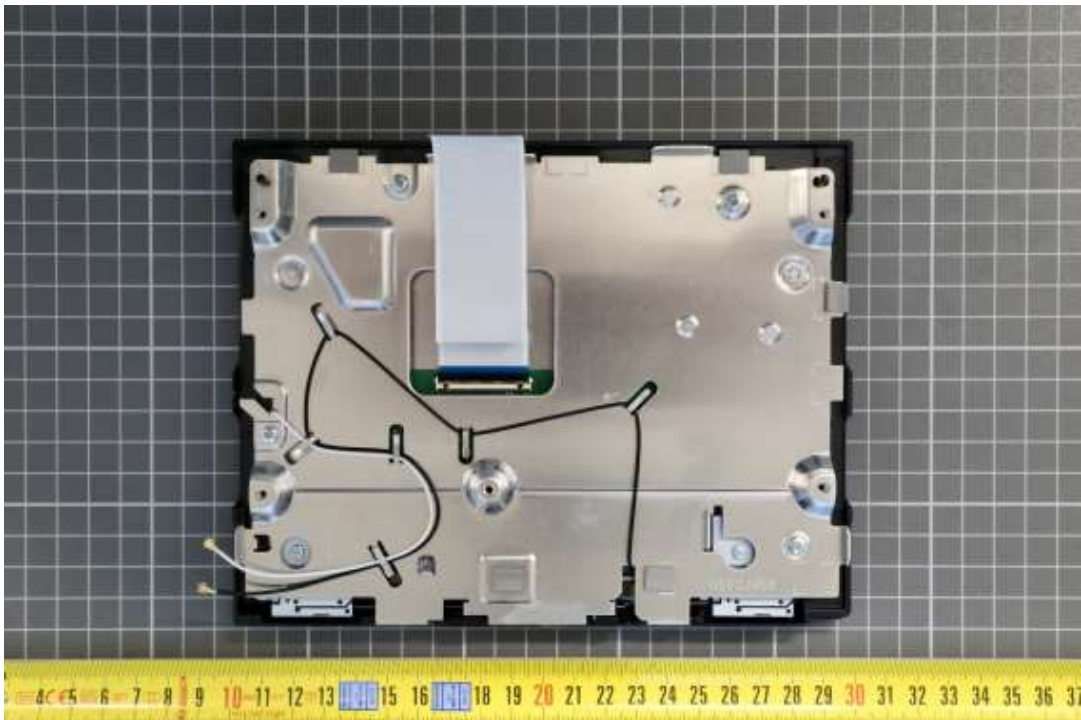
Photograph 40: EUT D
