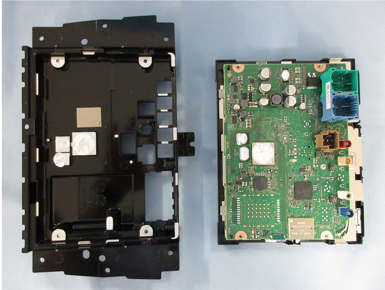
PCB-MAIN C-side
