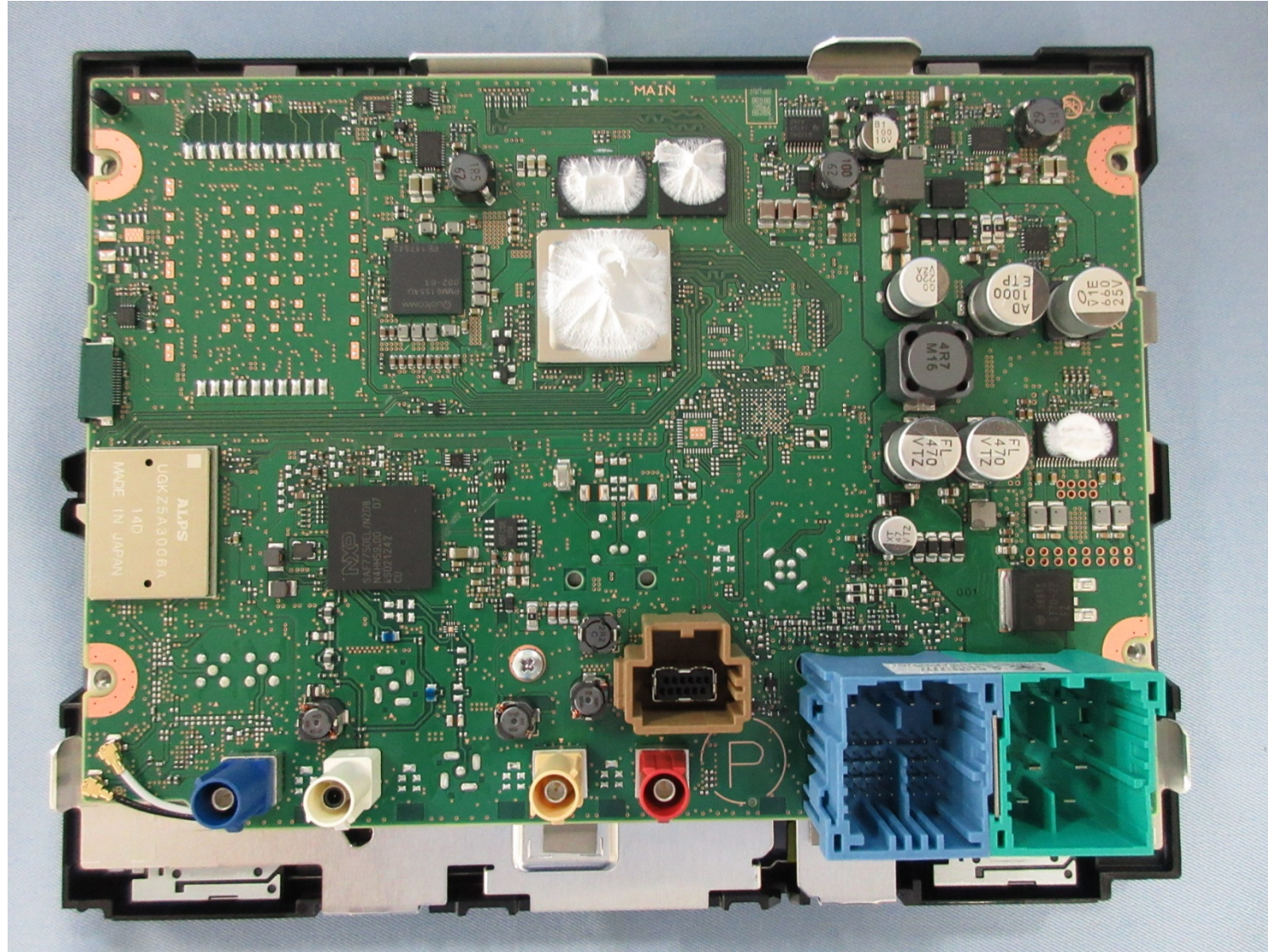
PCB-MAIN C-side
