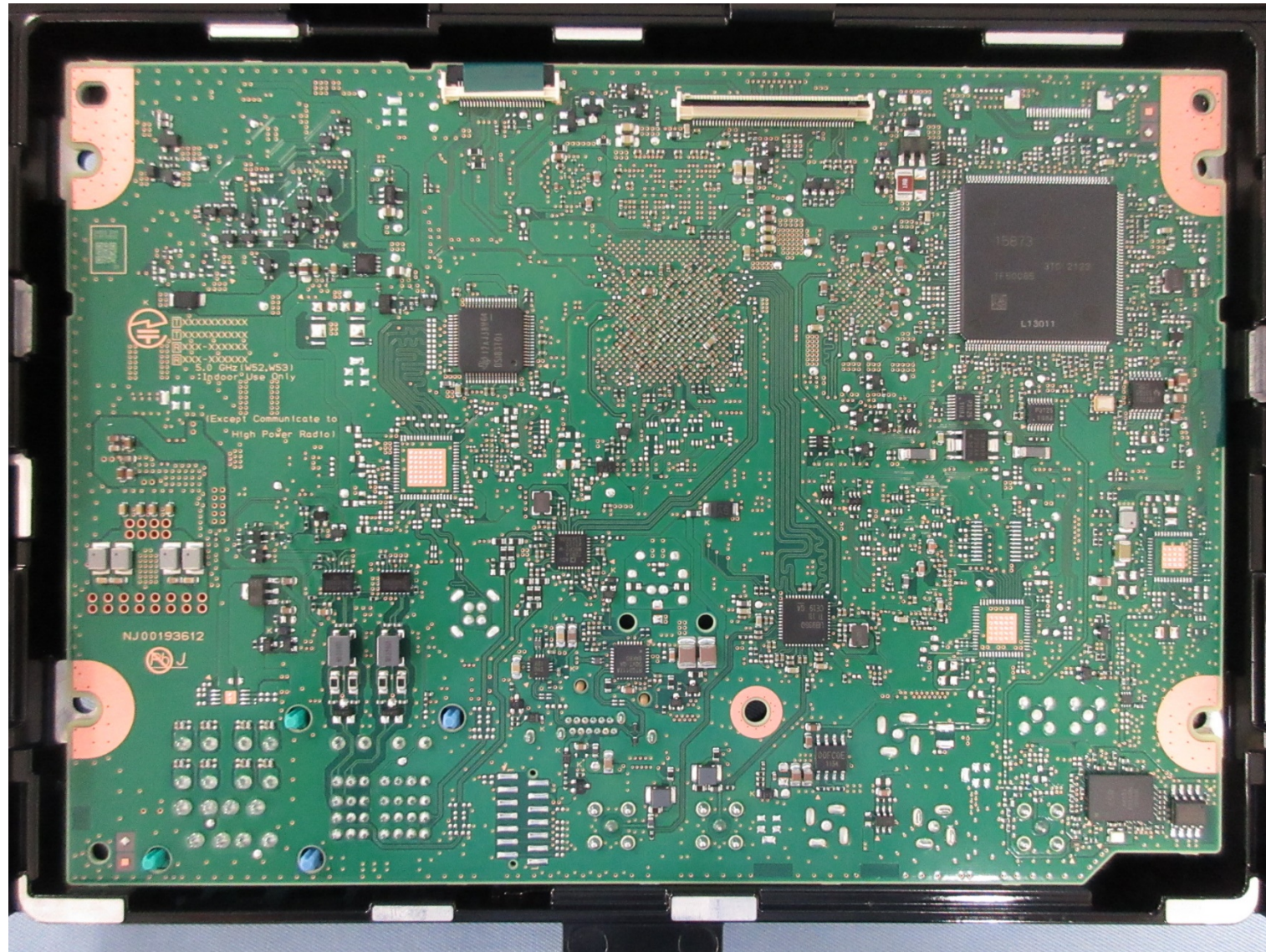
PCB-MAIN S-side
