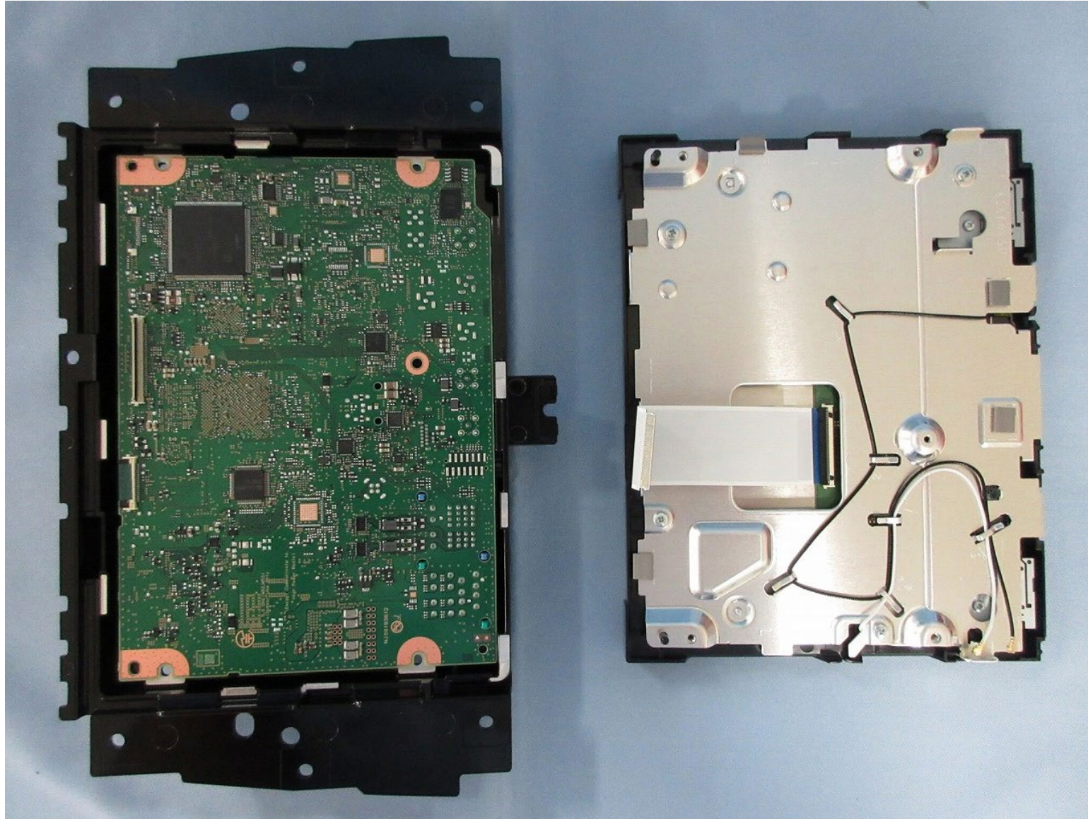
PCB-MAIN S-side
