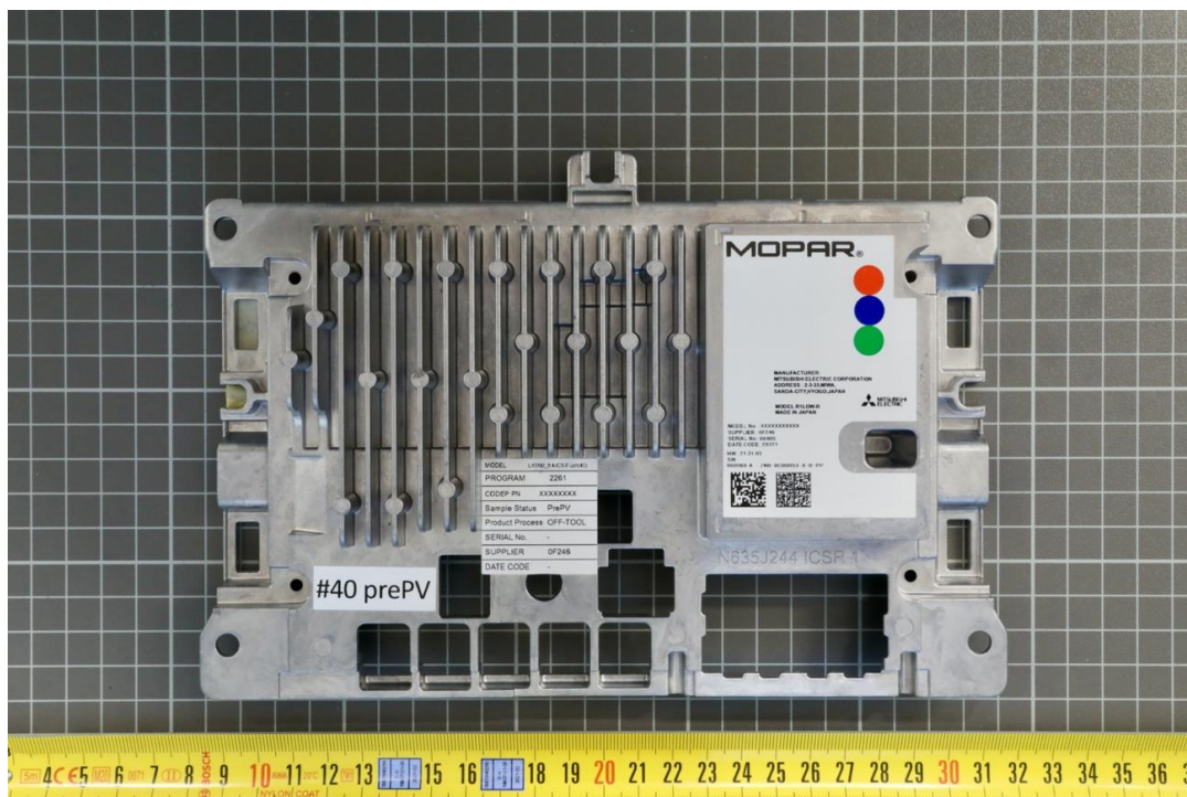
Photo No. 21: housing shell, rear view
