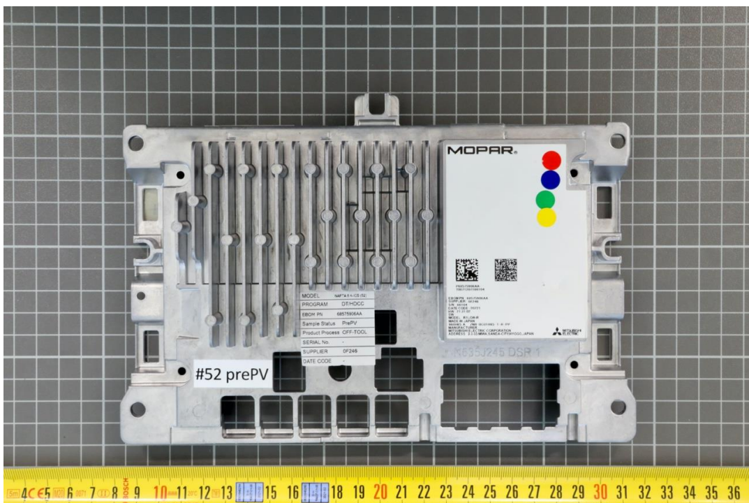
Photo No. 33: housing shell, rear view
