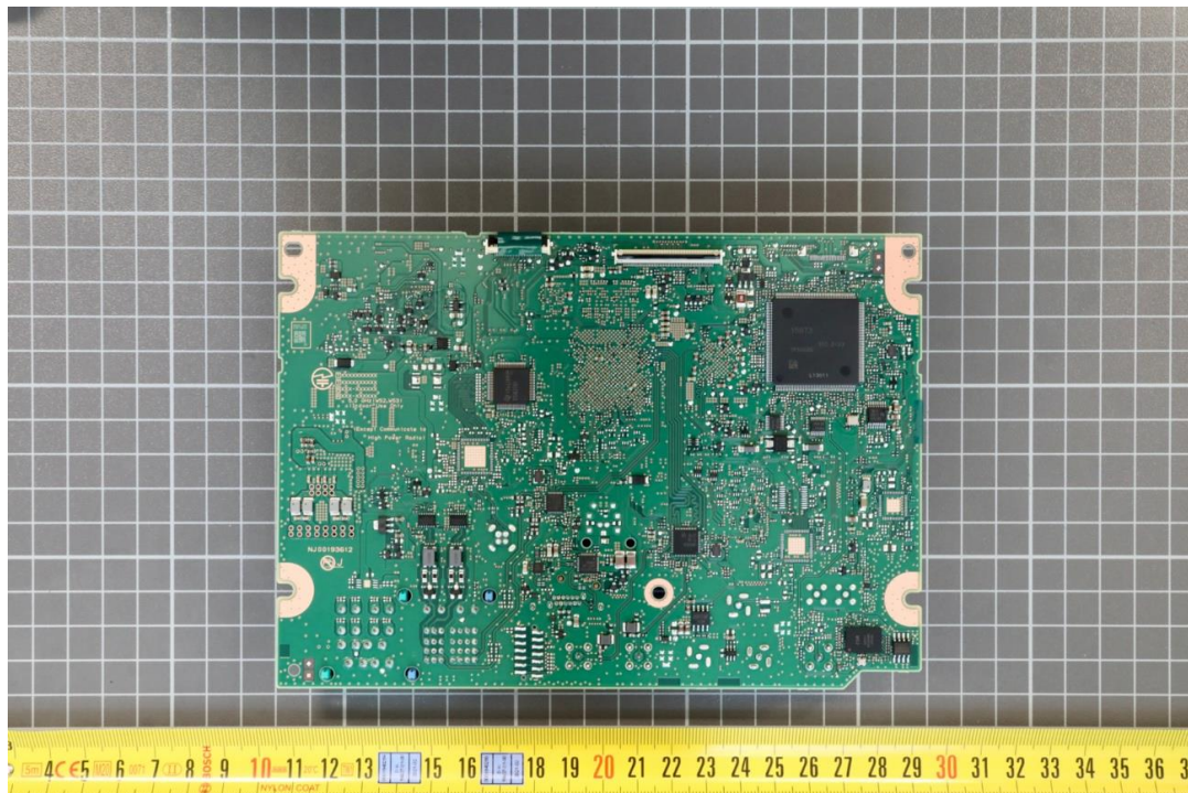
Photo No. 60: printed circuit board with interfaces, front view
