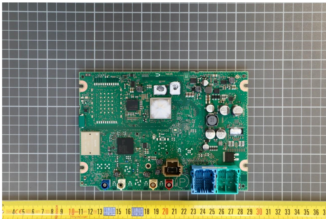
Photo No. 59: printed circuit board with interfaces, rear view
