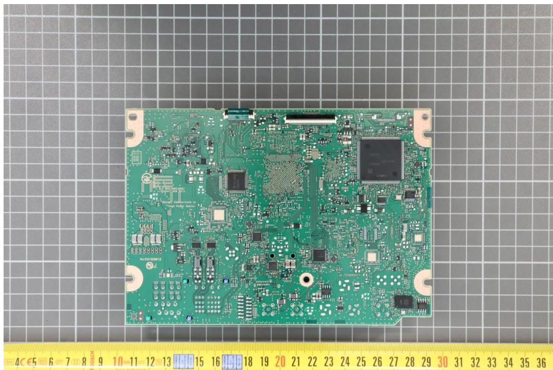
Photo No. 36: printed circuit board with interfaces, front view
