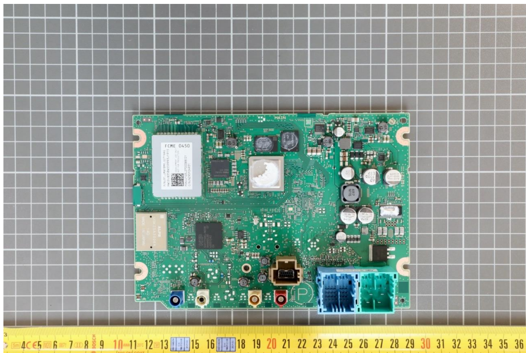
Photo No. 47: printed circuit board with interfaces, rear view
