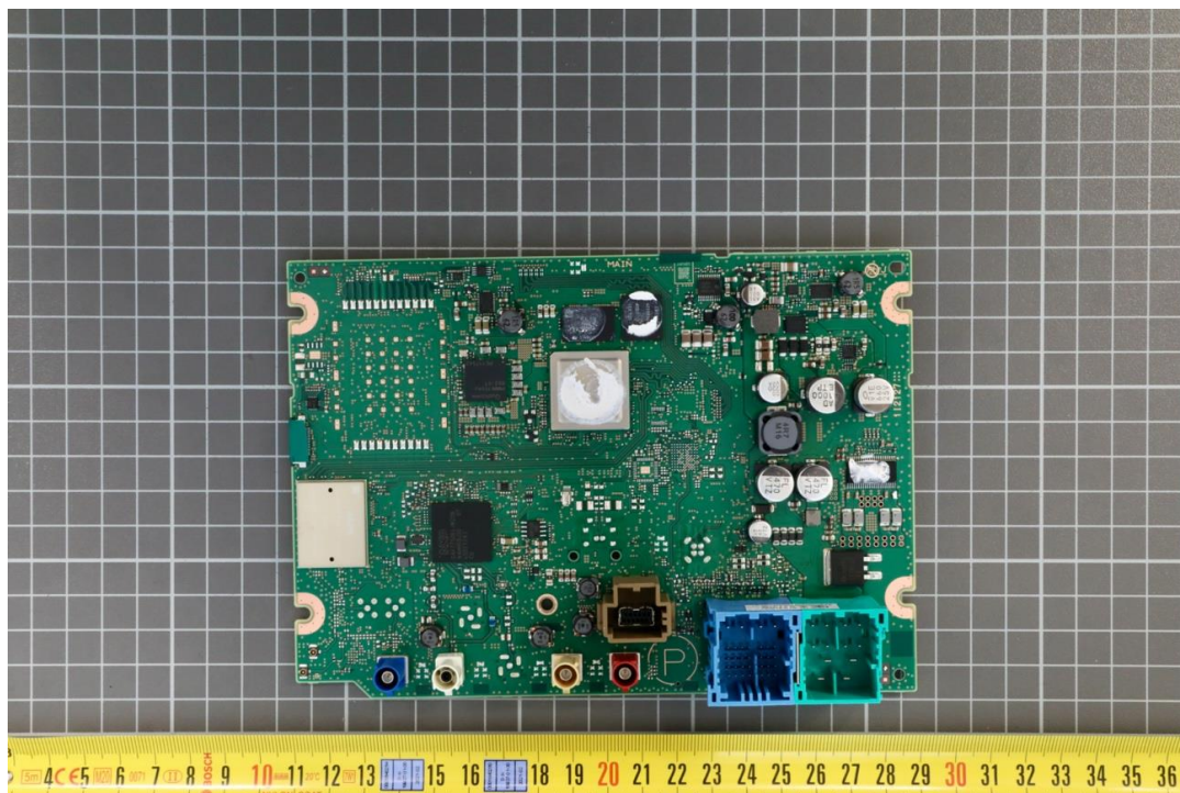
Photo No. 53: printed circuit board with interfaces, rear view
