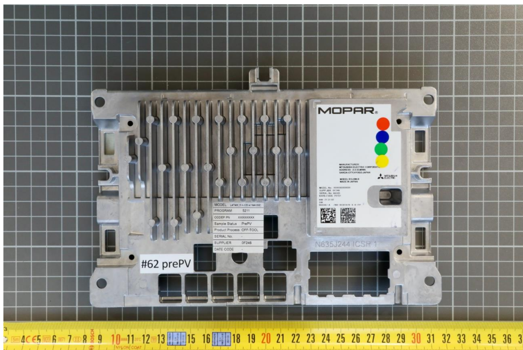
Photo No. 57: housing shell, rear view
