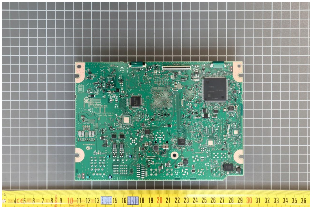
Photo No. 42: printed circuit board with interfaces, front view
