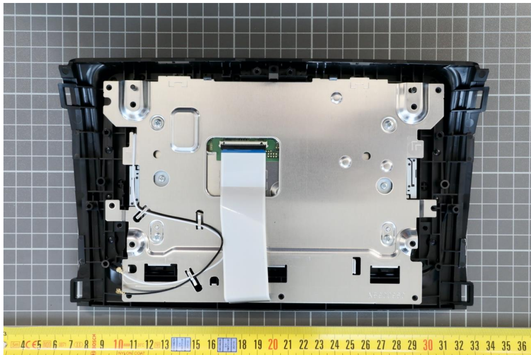
Photo No. 39: housing shell, rear view
