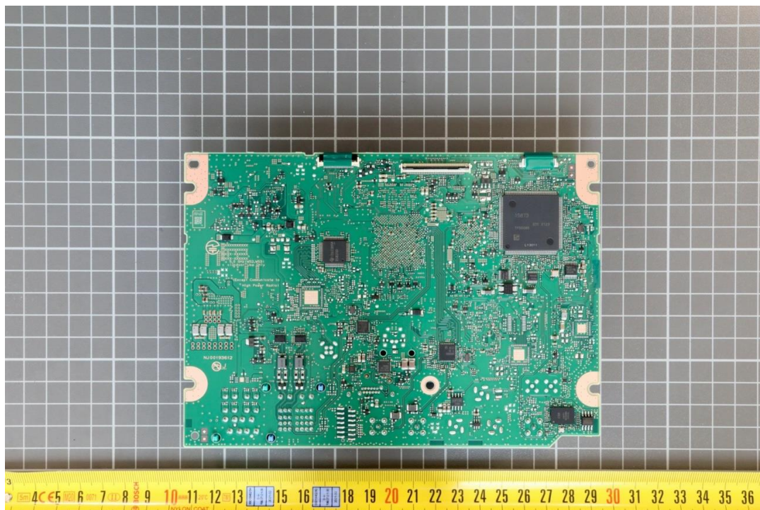
Photo No. 48: printed circuit board with interfaces, front view
