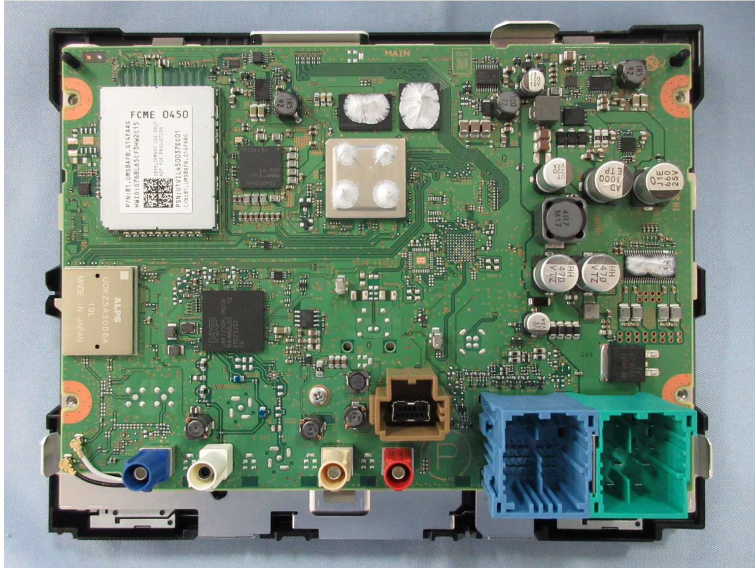
PCB-MAIN C-side
