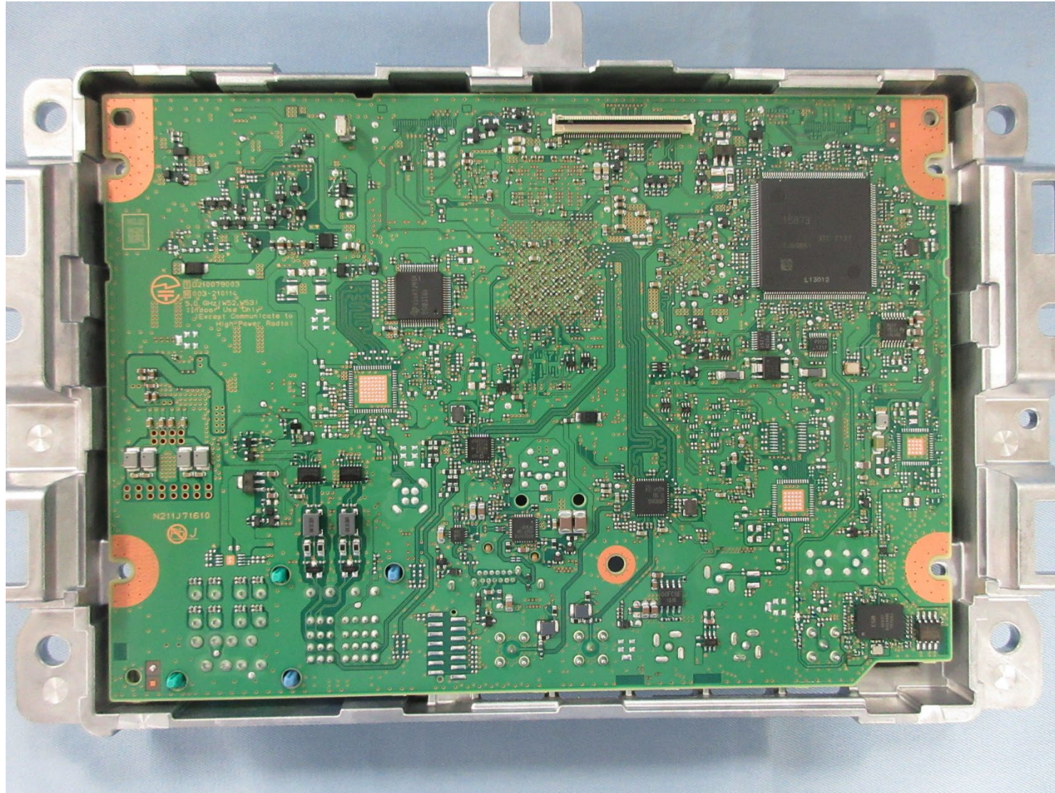
PCB-MAIN S-side
