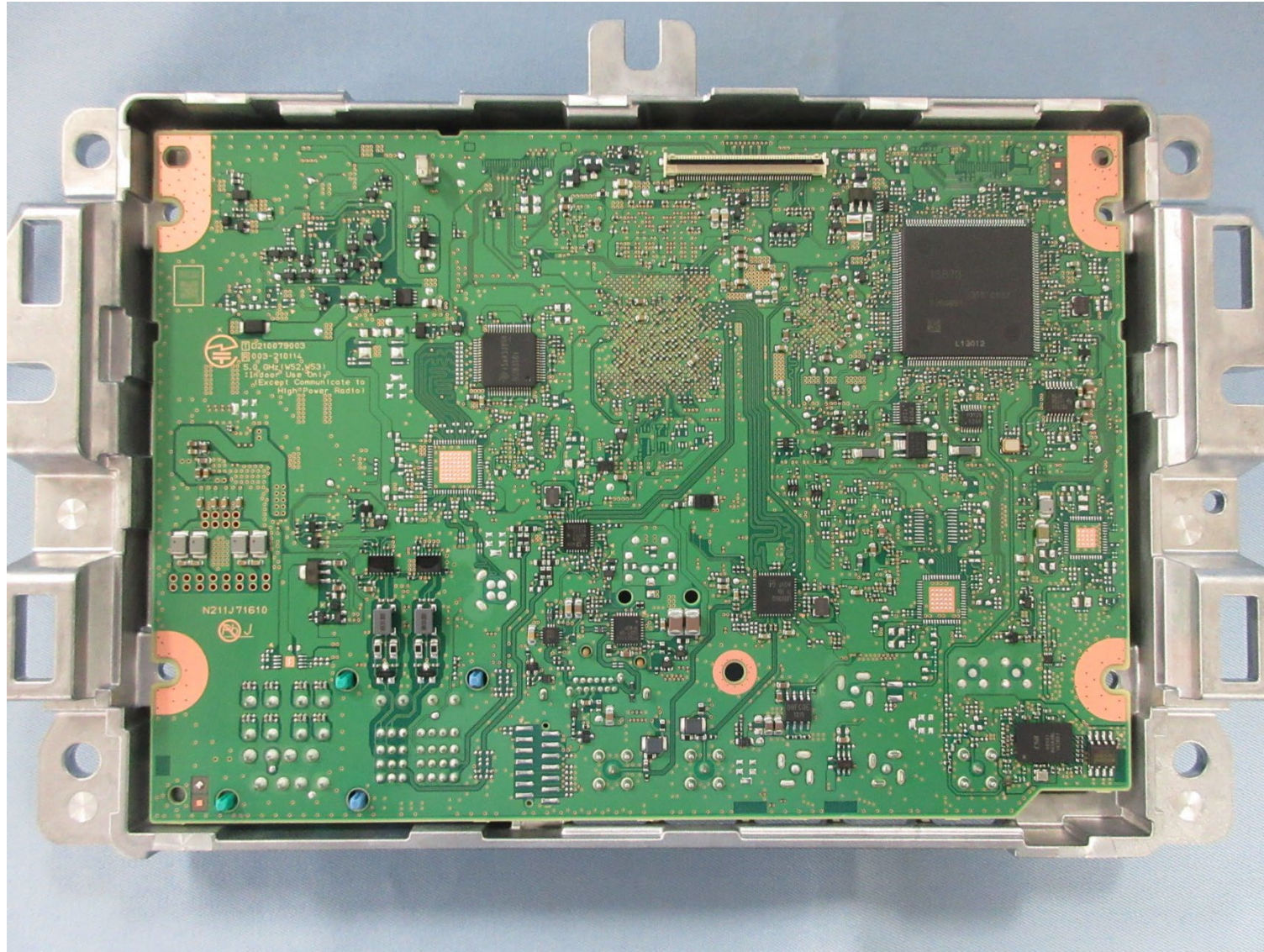
PCB-MAIN S-side
