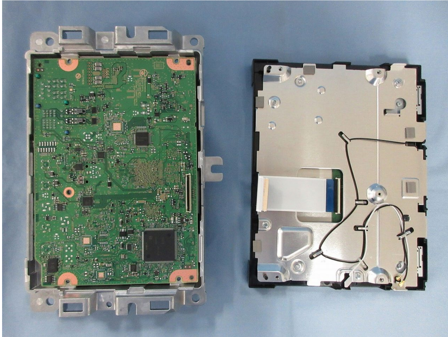
PCB-MAIN S-side
