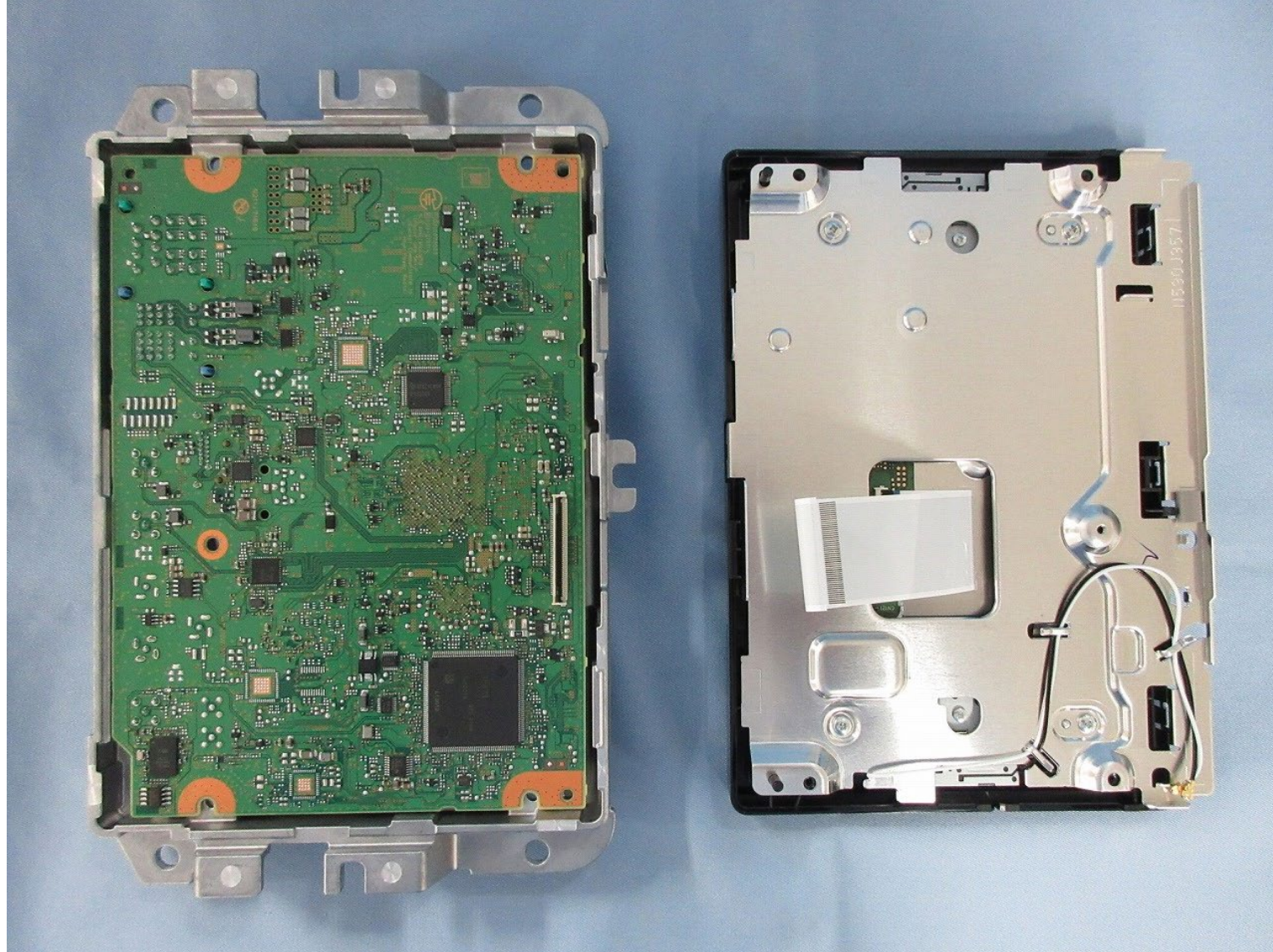
PCB-MAIN S-side
