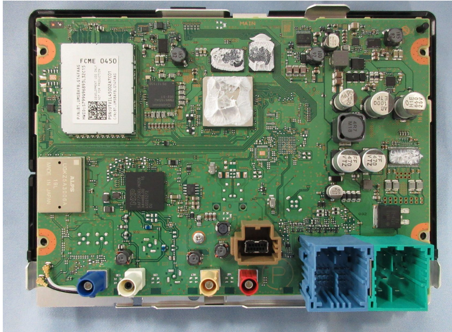
PCB-MAIN C-side
