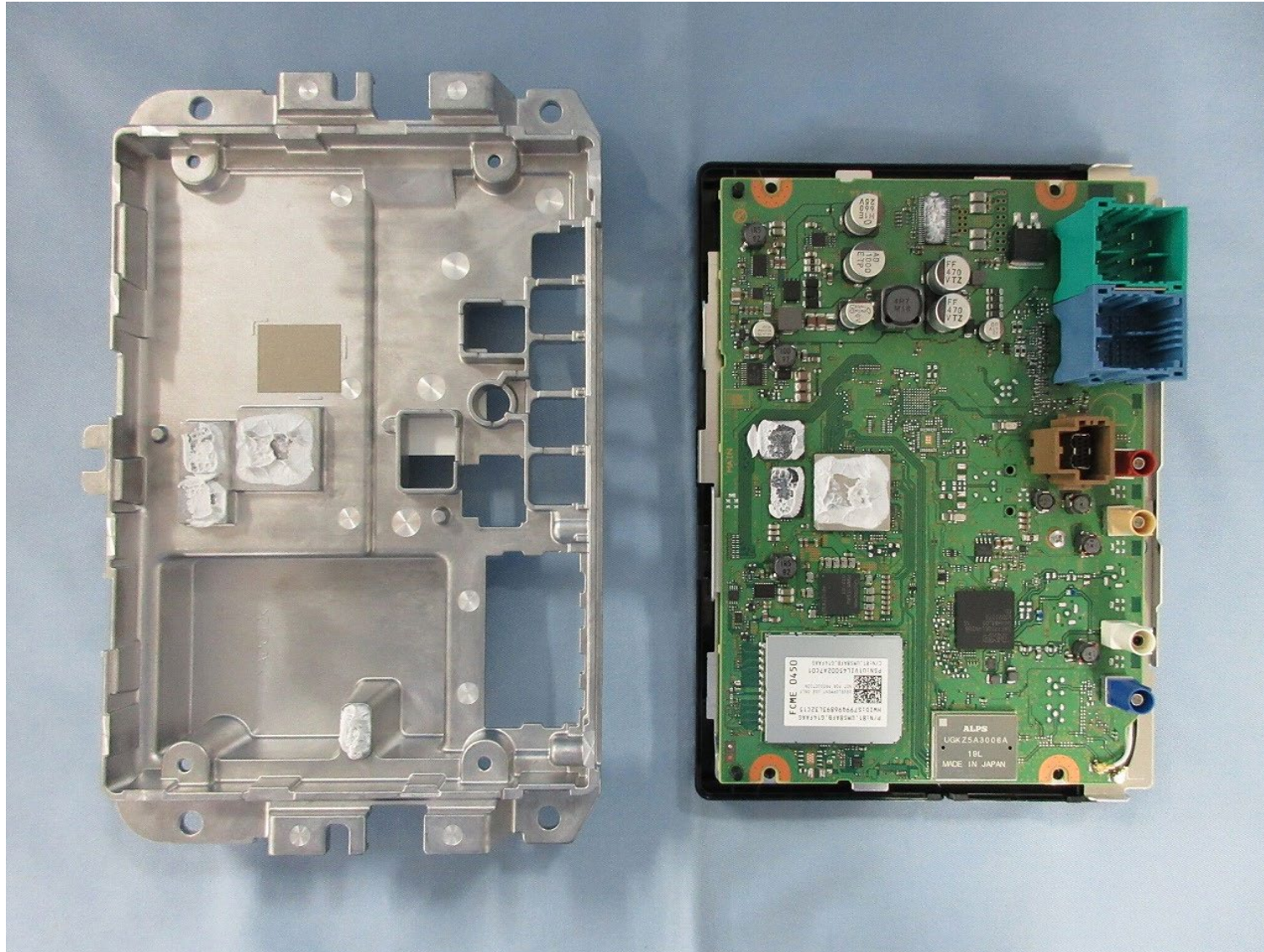
PCB-MAIN C-side
