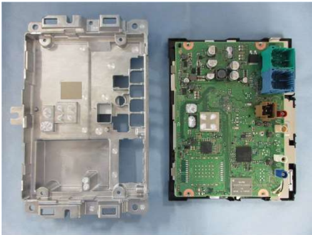
Photograph 18: EUT B
