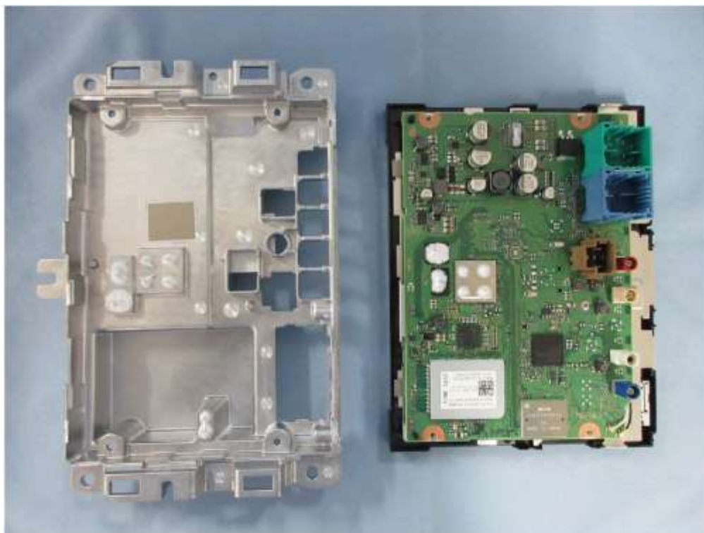
Photograph 14: EUT A
