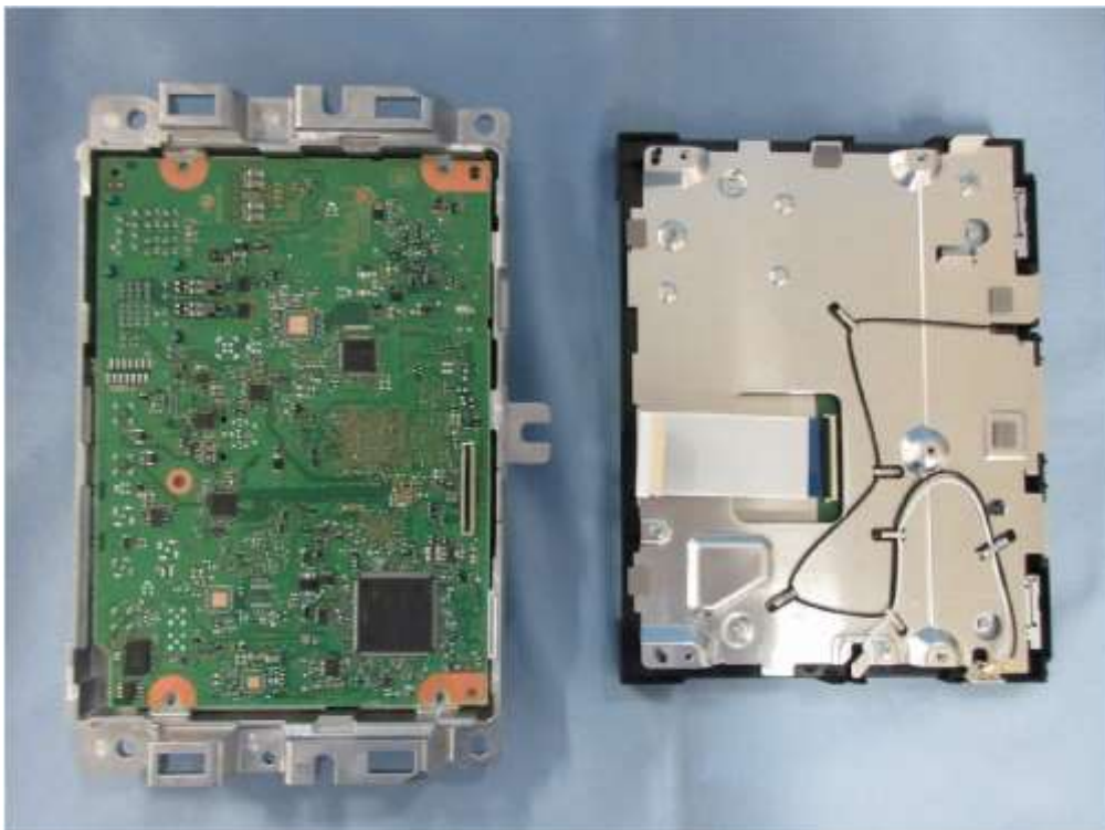
Photograph 16: EUT A
