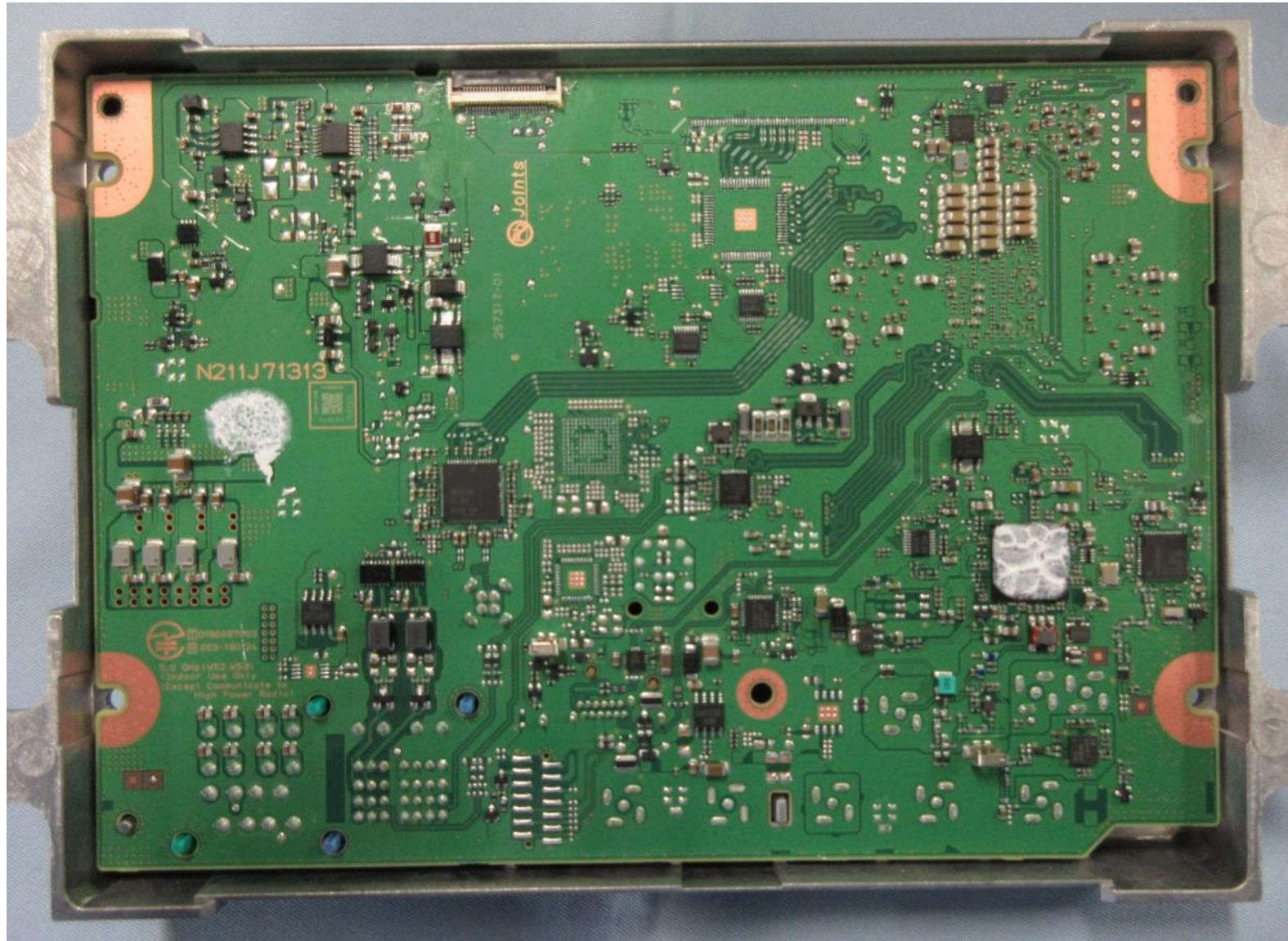
PCB-MAIN S-side
