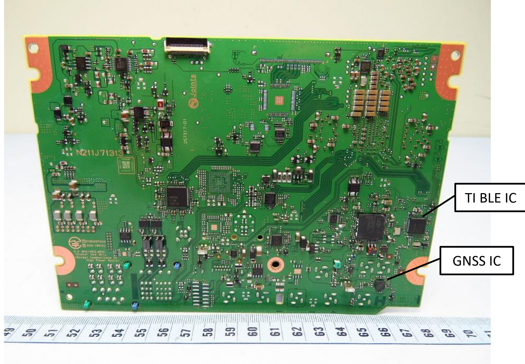
PCB-MAIN S-side
