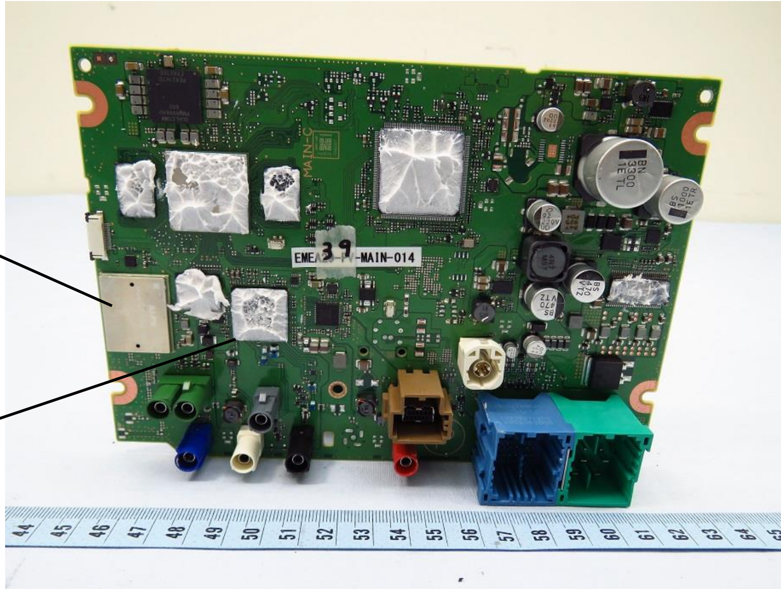
PCB-MAIN C-side
