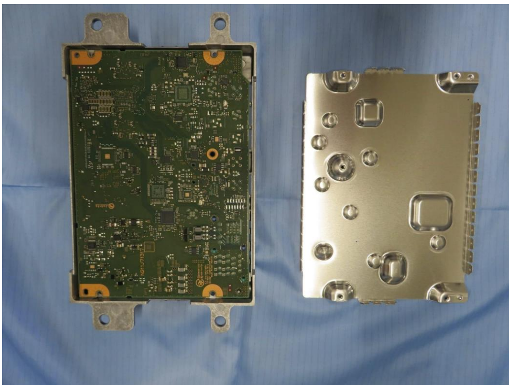
Photograph 16: EUT A
