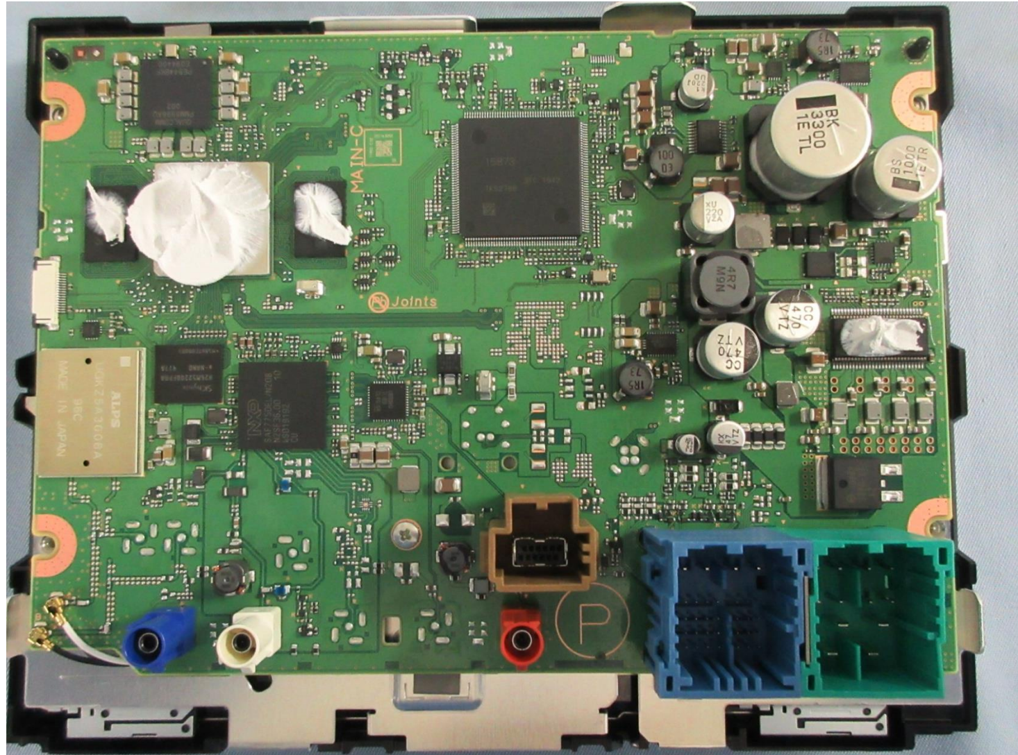
PCB-MAIN C-side
