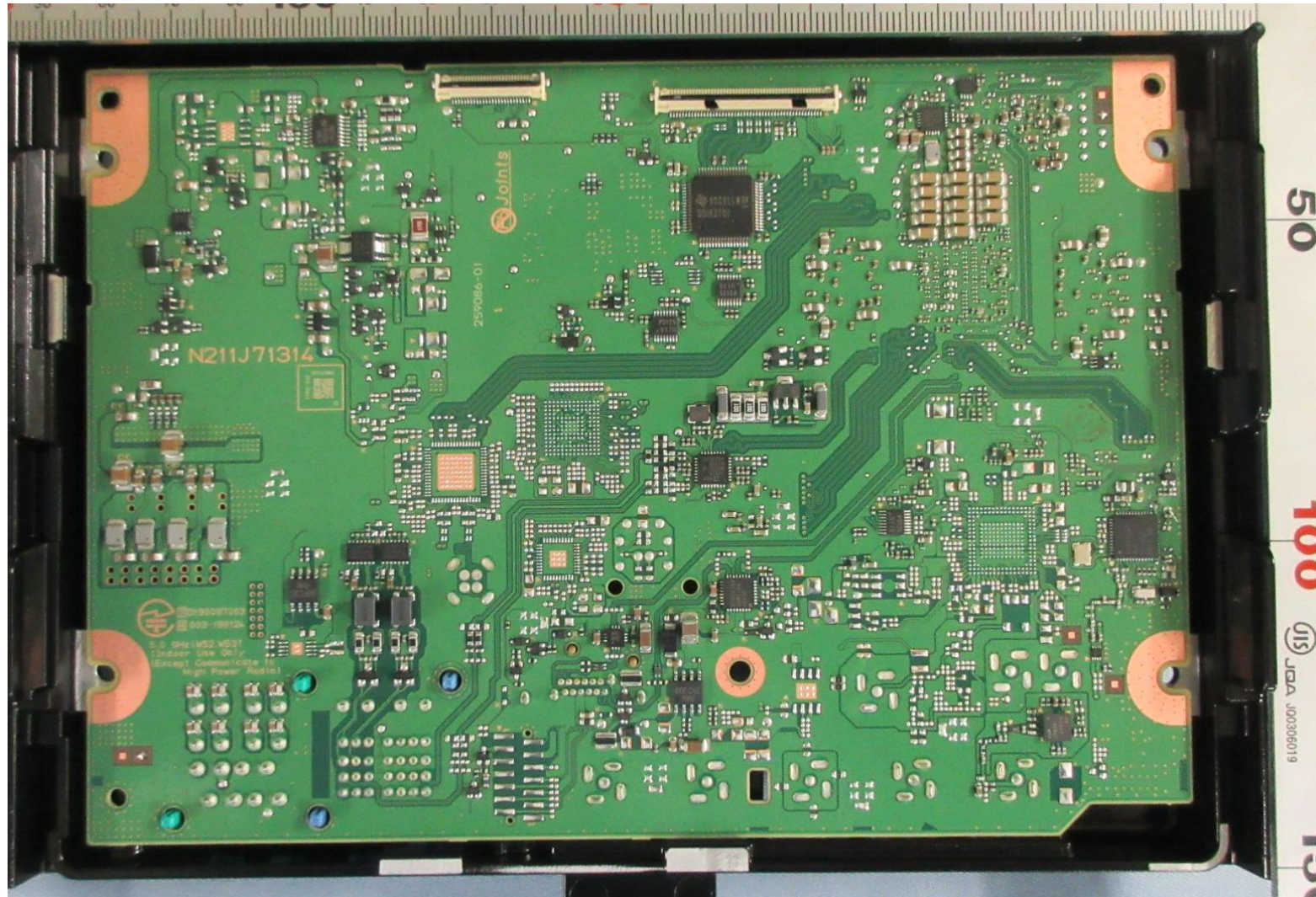
PCB-MAIN S-side
