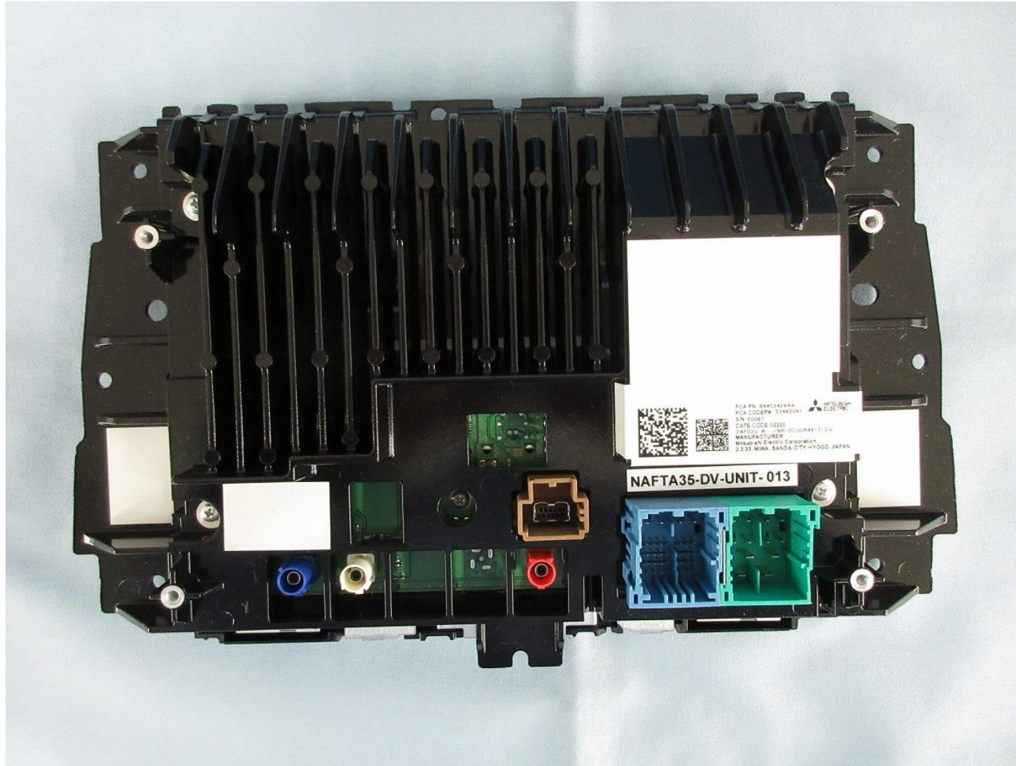
Rear side
