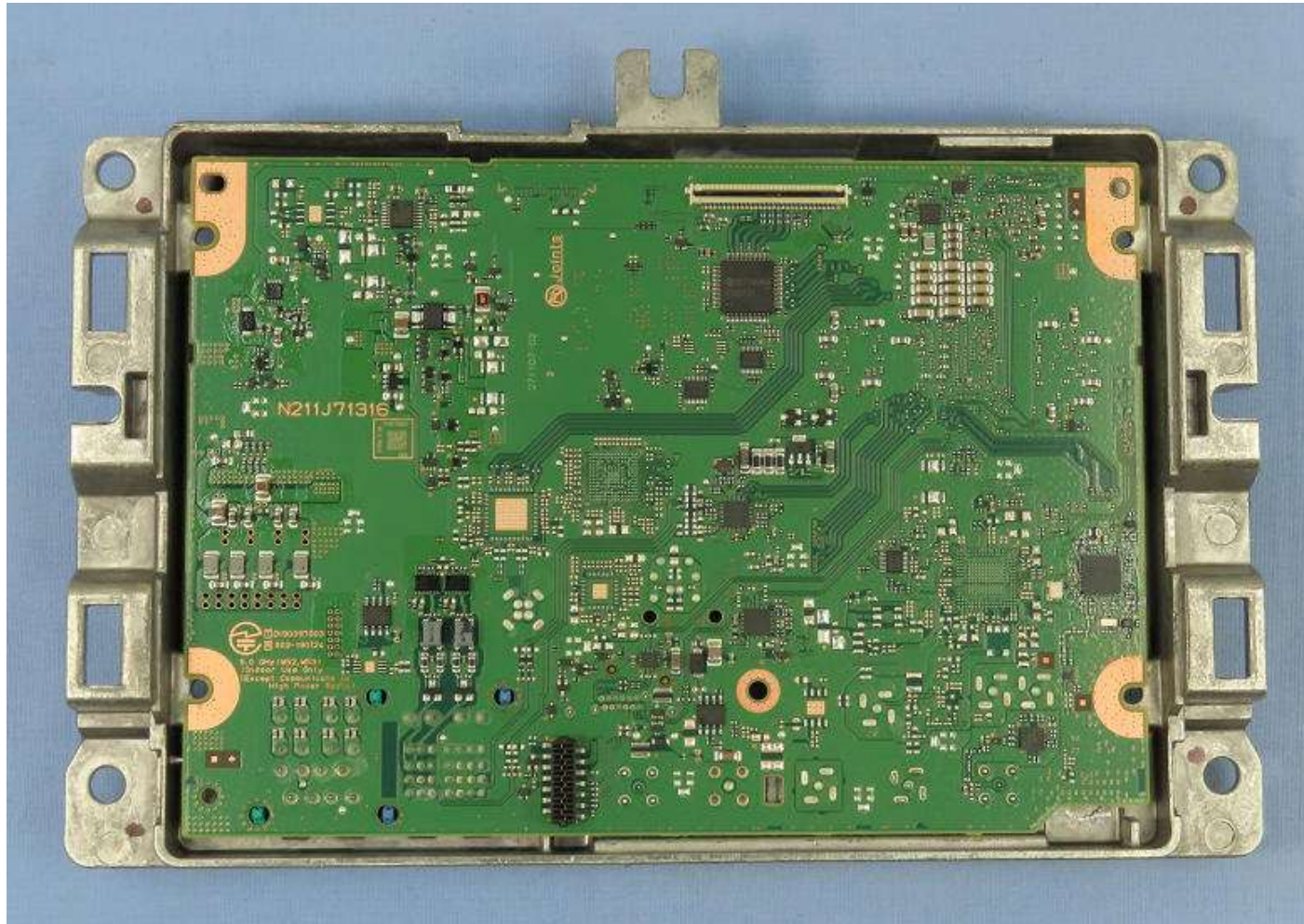
PCB-MAIN S-side
