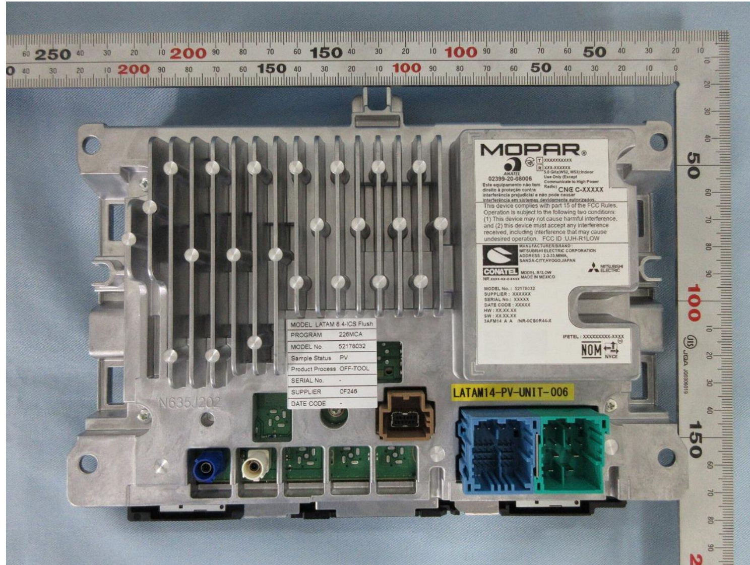
Rear side
