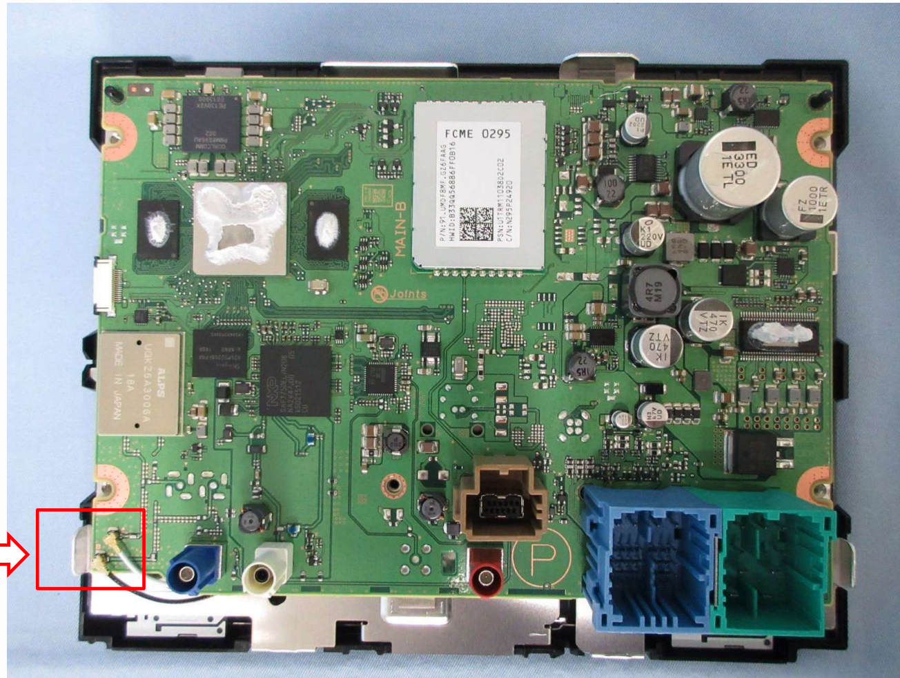
PCB-MAIN C-side
