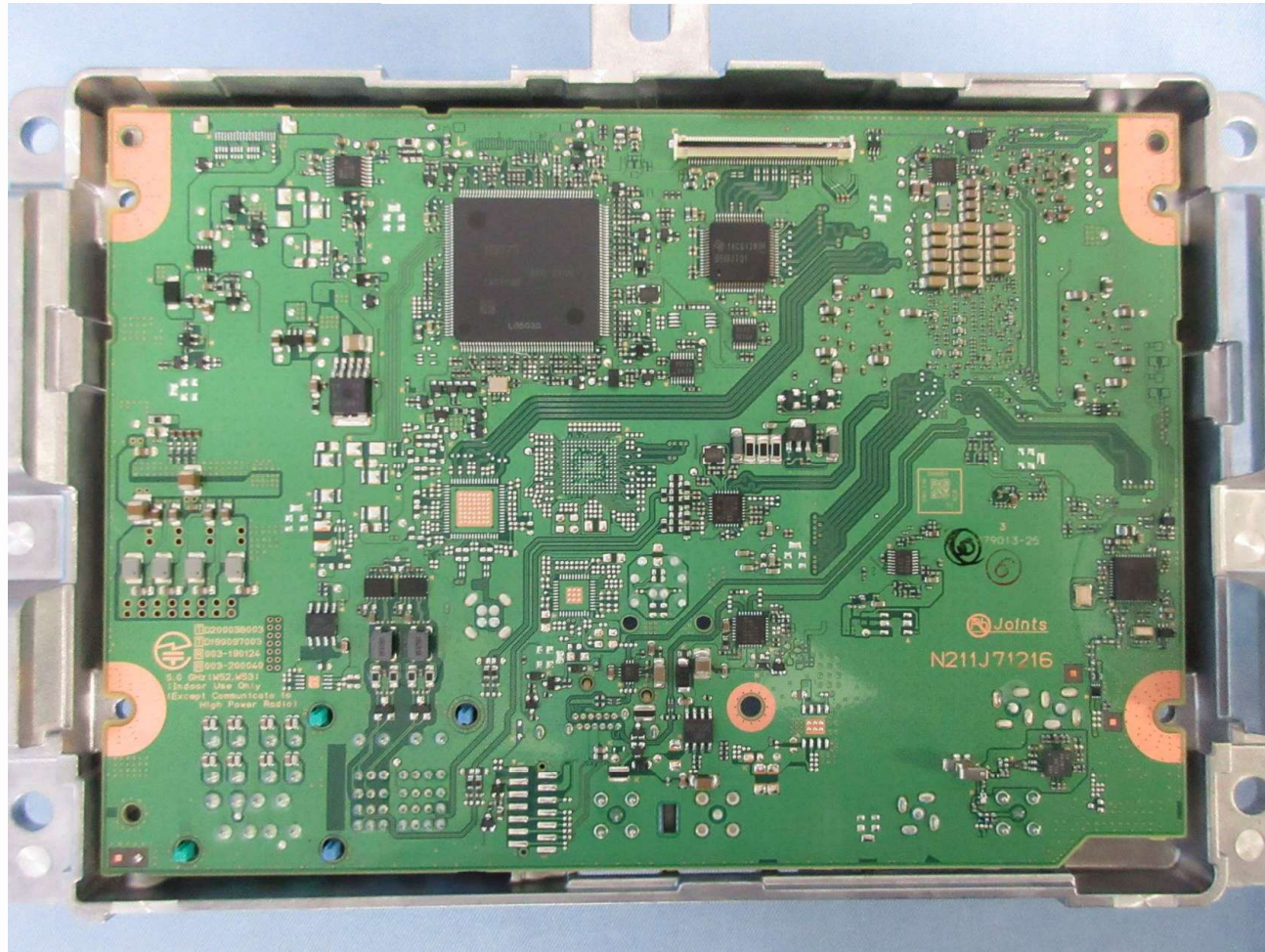
PCB-MAIN S-side
