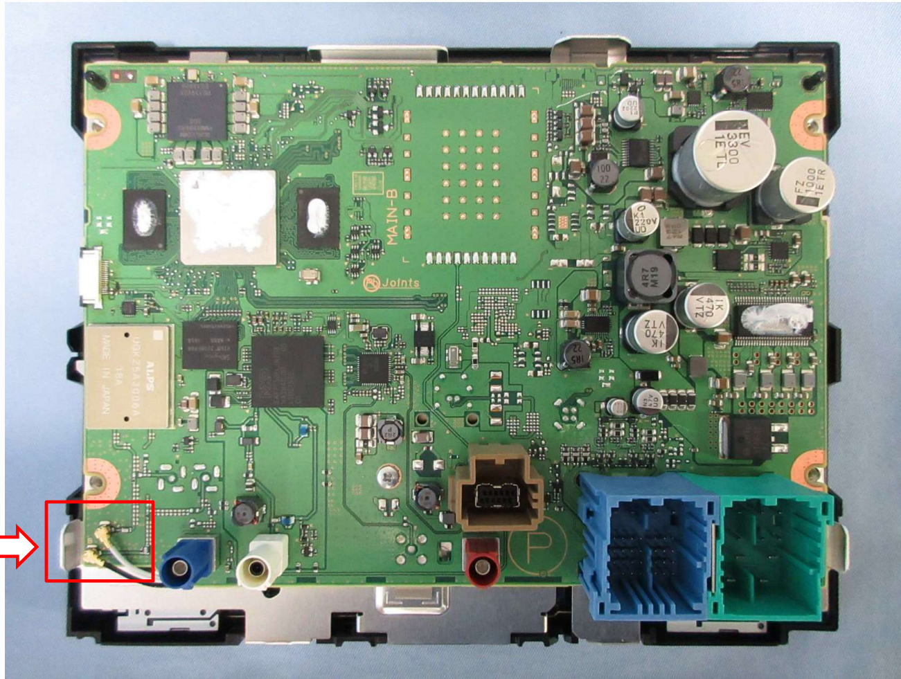
PCB-MAIN C-side
