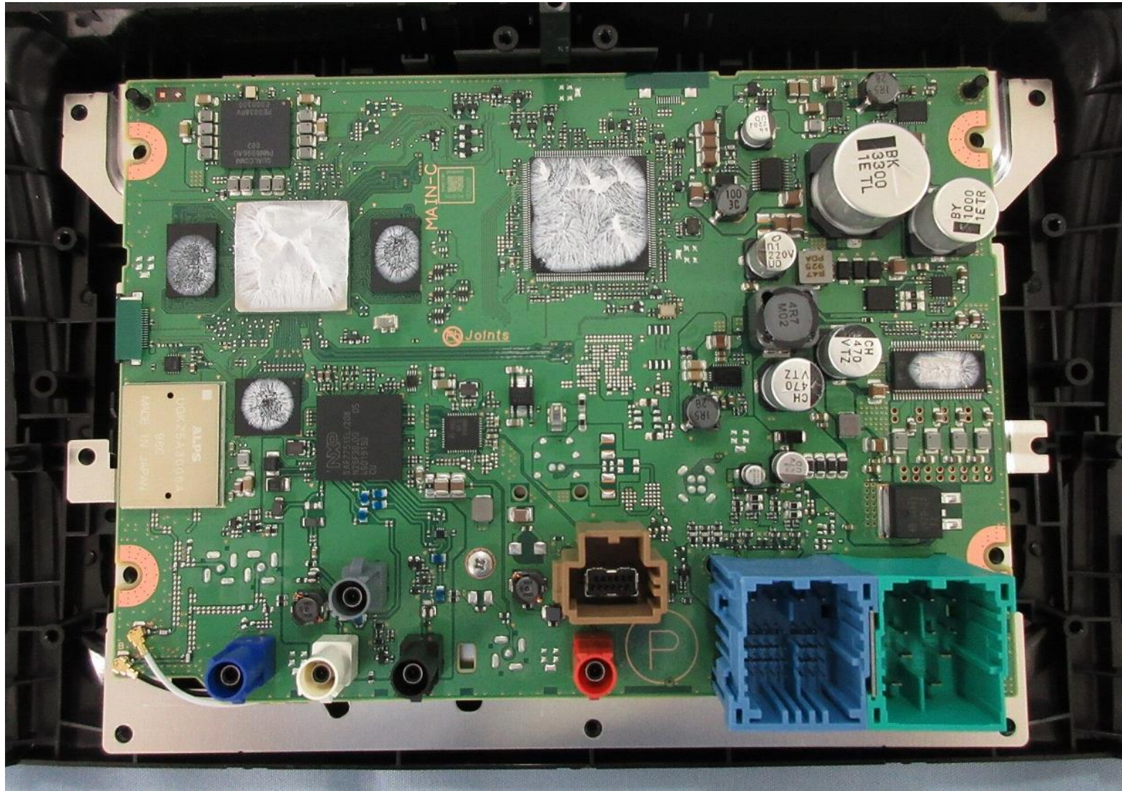
PCB-MAIN C-side
