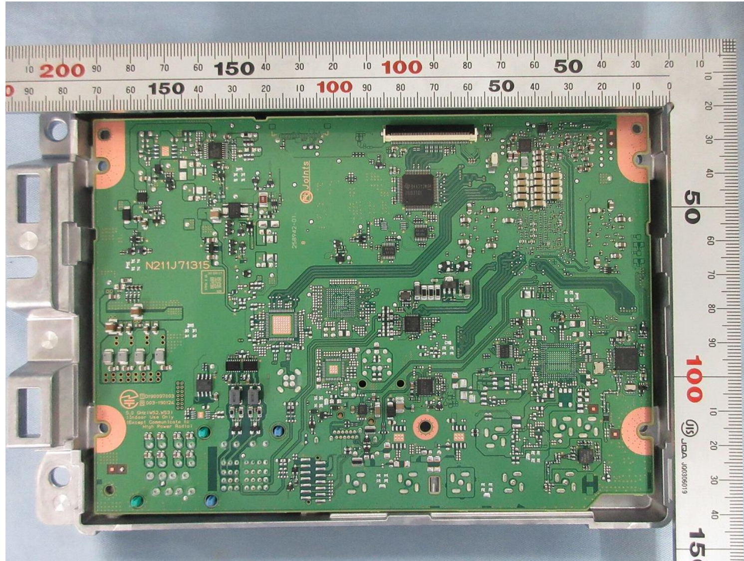
PCB-MAIN S-side
