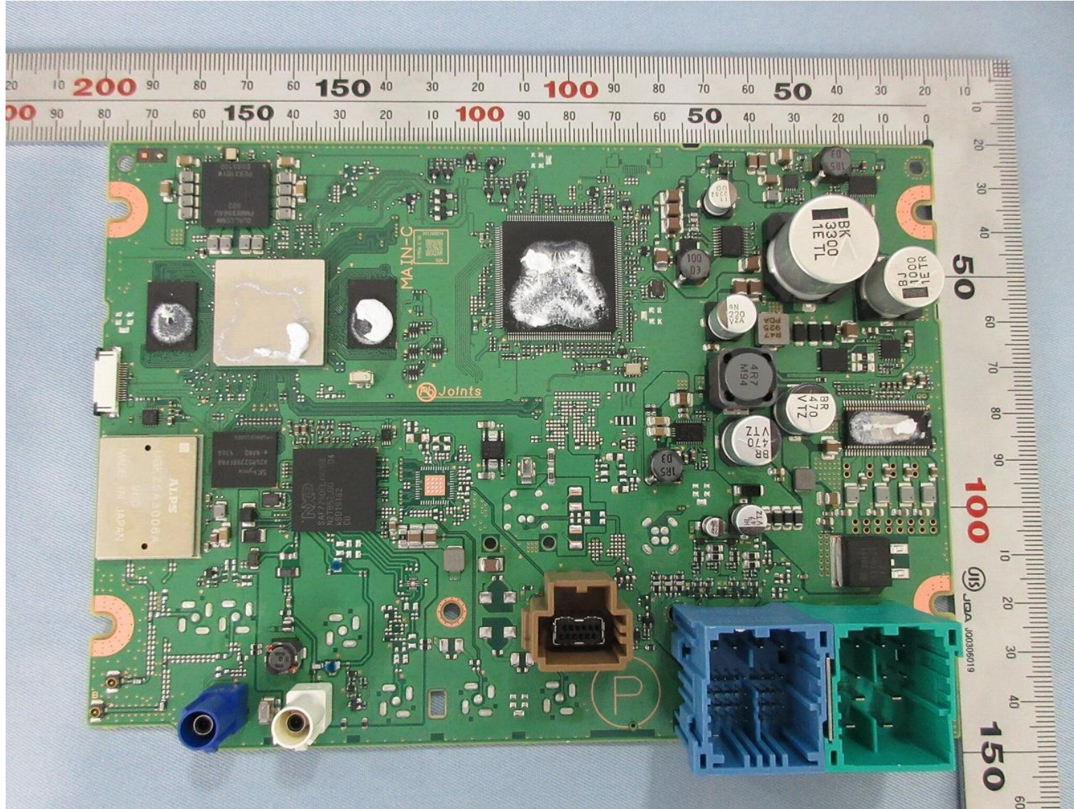
PCB-MAIN C-side
