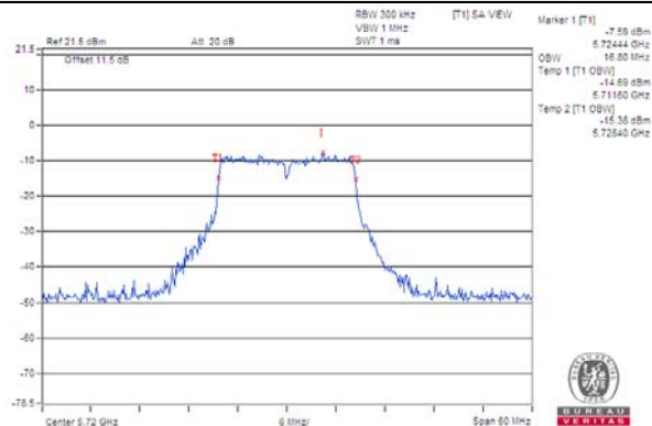
802.11n (HT20) / Chain 1 / CH 144
