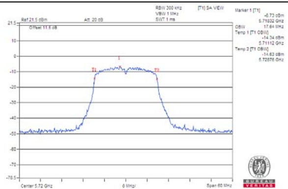
802.11n (HT40) / Chain 0 / CH 142
