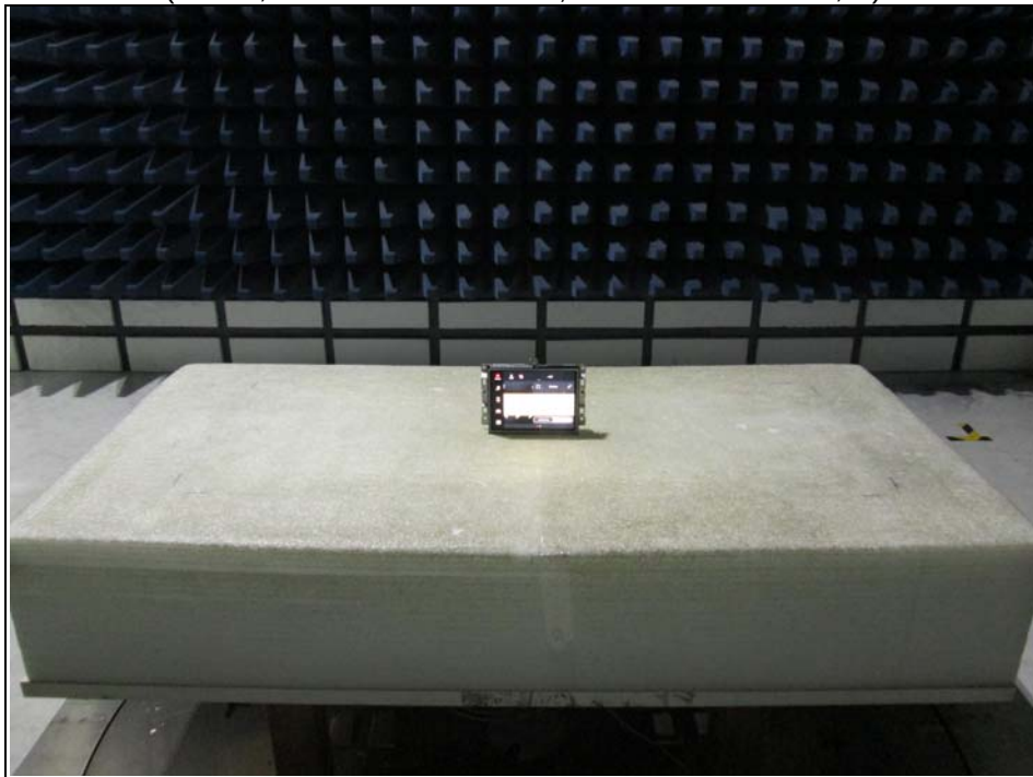
Radiated Emission Test below 1GHz (WLAN, BT EDR: Test Mode B; BT LE: Test Mode C, D)
