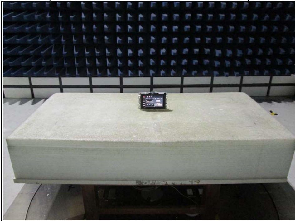
Radiated Emission Test below 1GHz (WLAN, BT EDR: Test Mode A; BT LE: Test Mode A, B)
