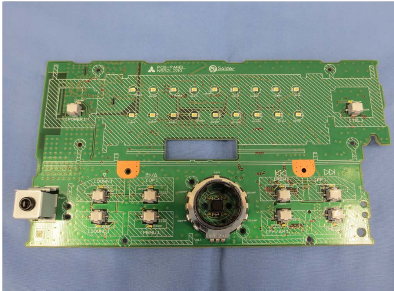
1. PCB-PANEL C-side
