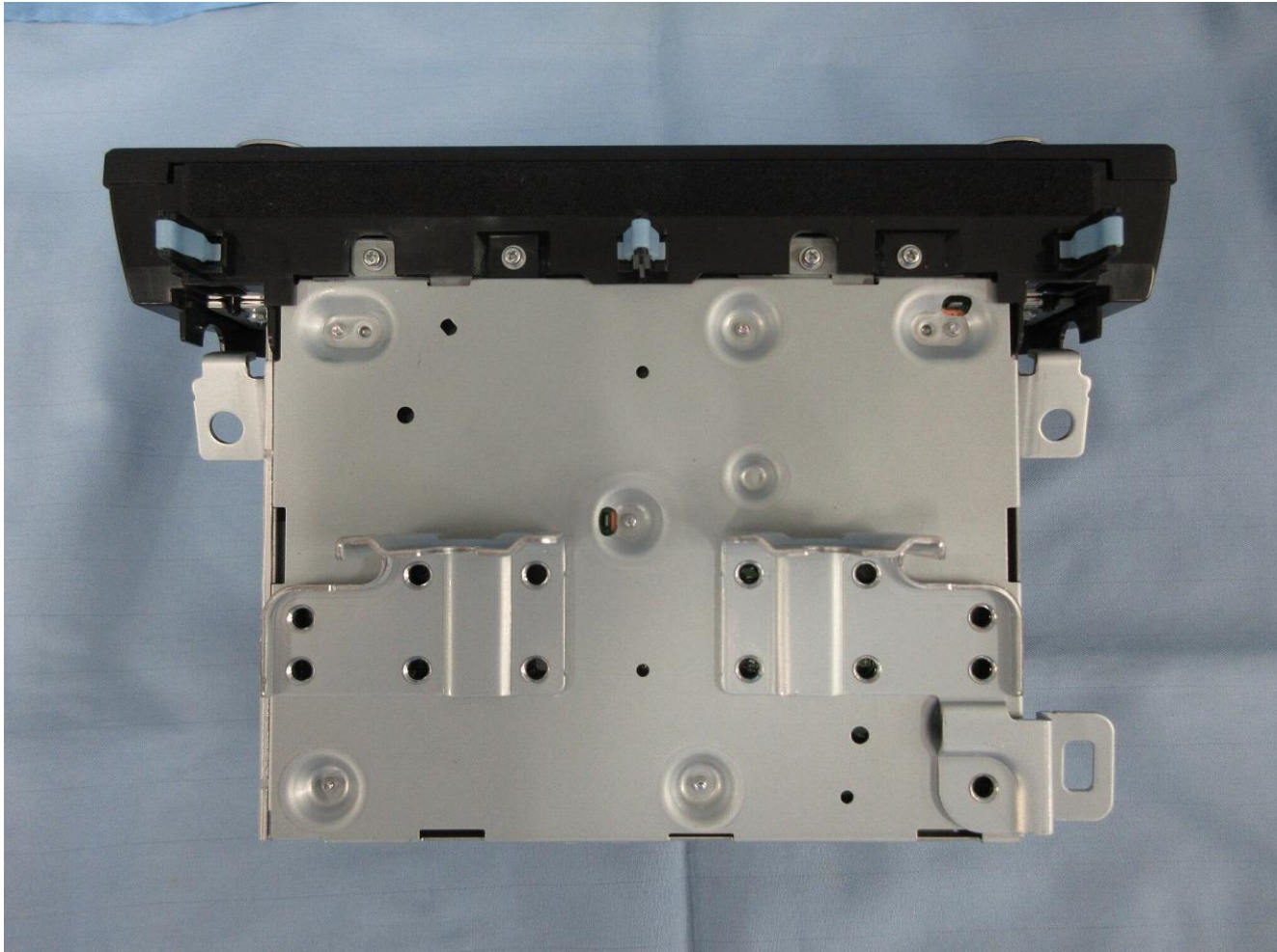
5. Bottom View
