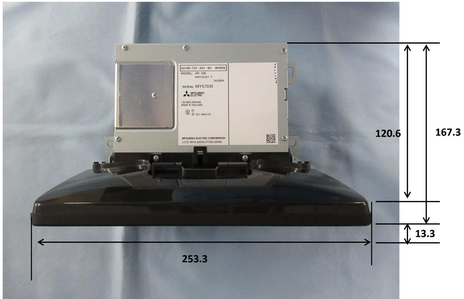
2. Top View
