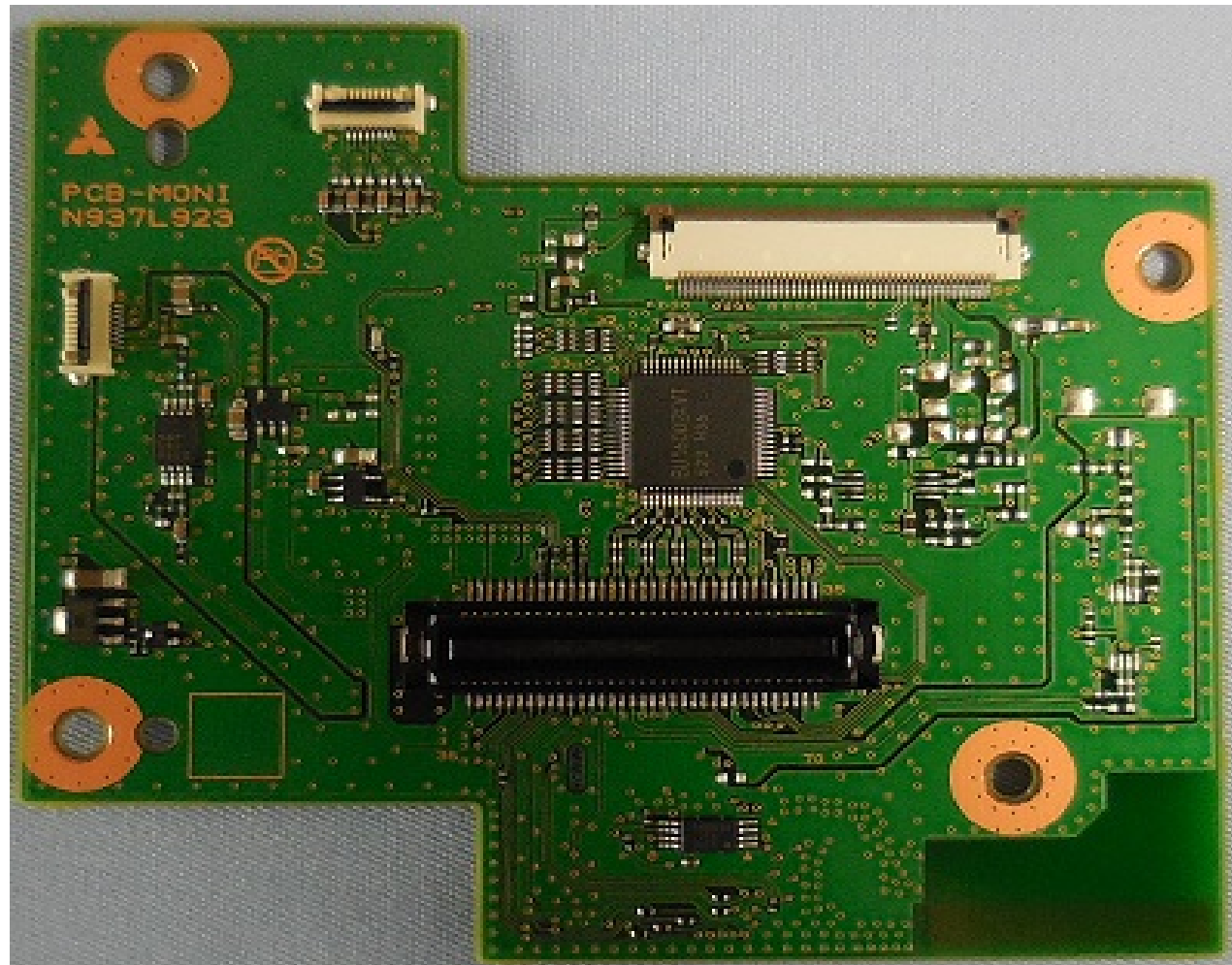
3. PCB-MONI C-side
