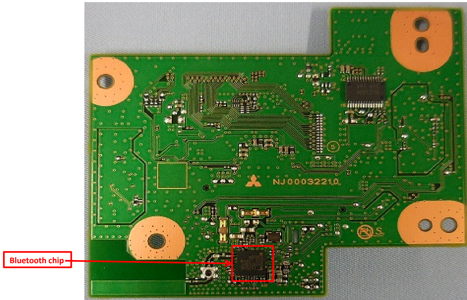
4. PCB-MONI S-side
