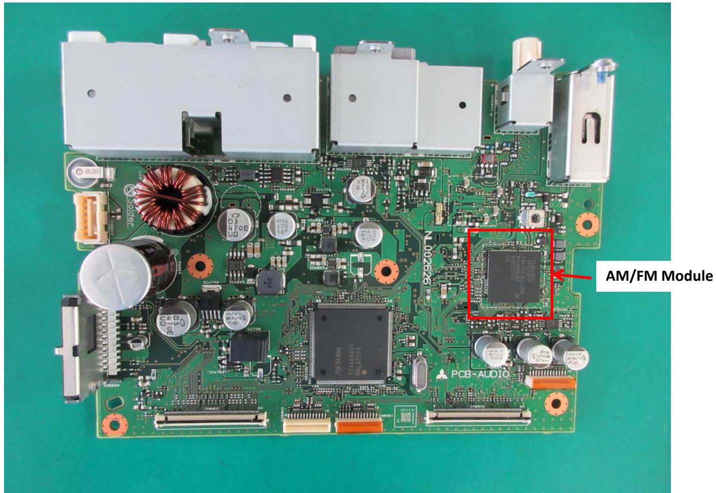
3. PCB-AUDIO C-side
