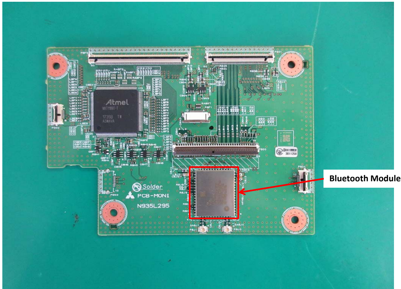
5. PCB-MONI C-side
