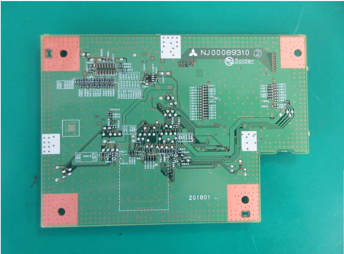
6. PCB-MONI S-side
