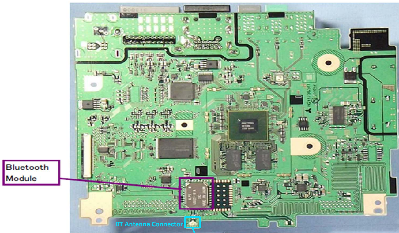
Radio module and antenna position of NR-244UH/NR-245UH (BT only)
