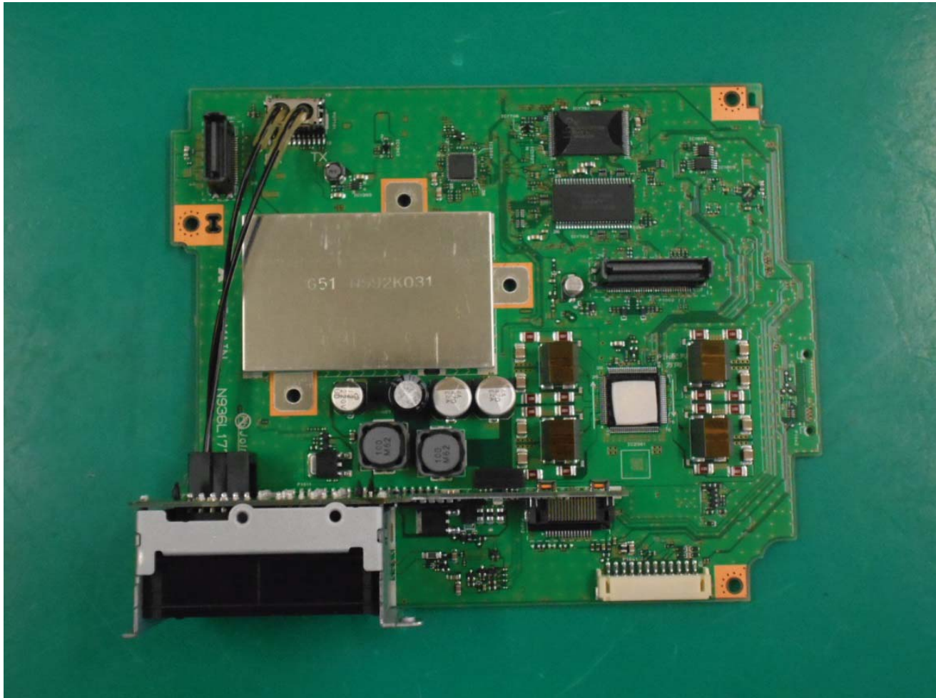
3. PCB-MAIN C-side
