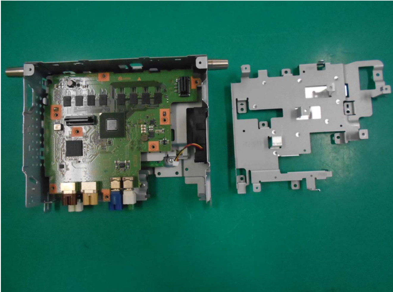
10. PCB-NVI Cover is removed.
