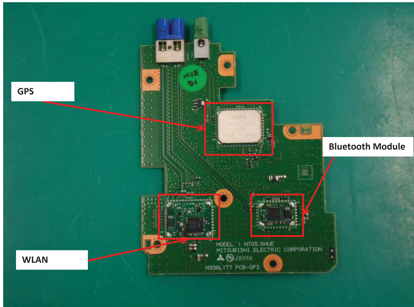
5. PCB-GPS C-side
