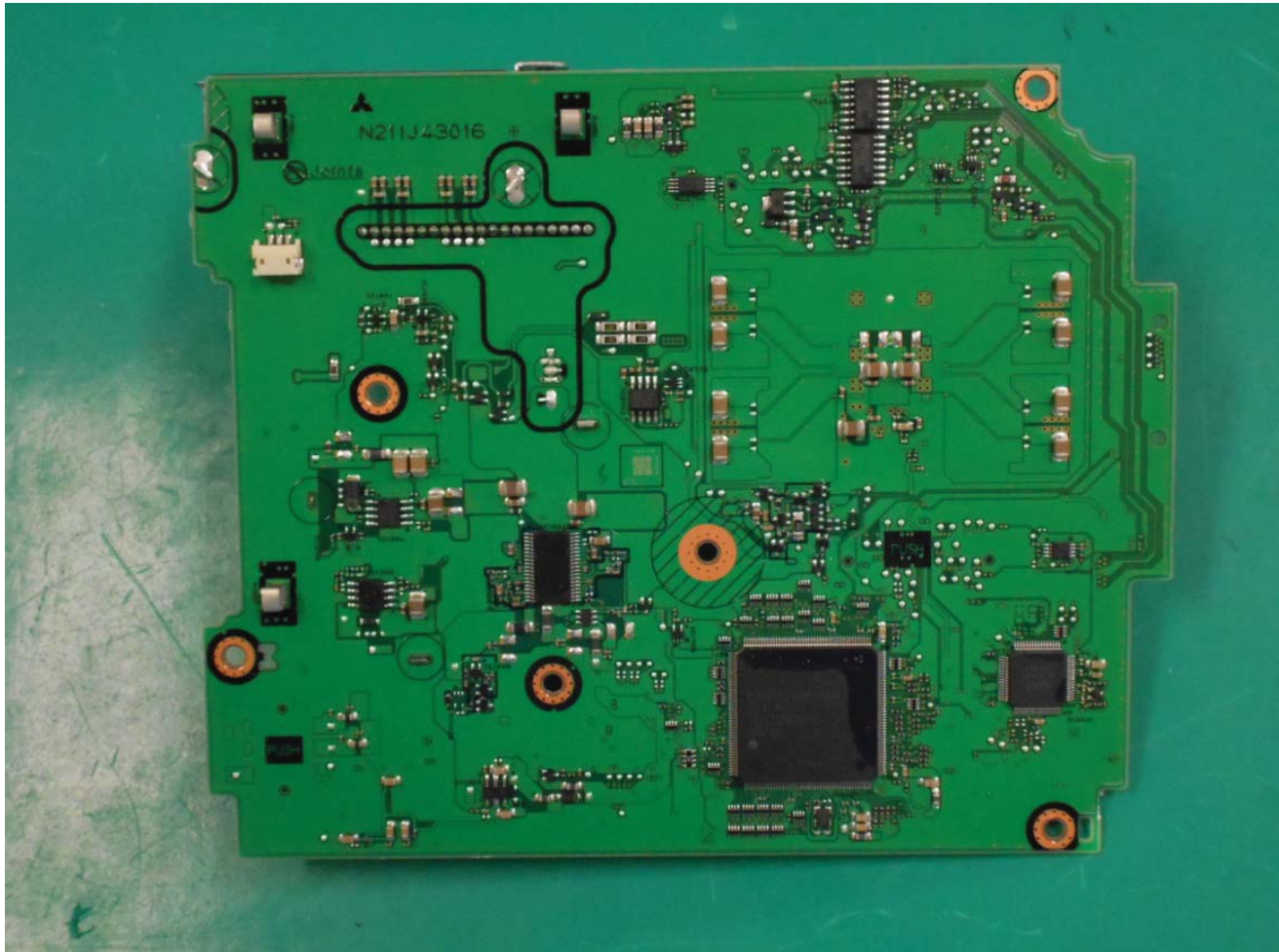
4. PCB-MAIN S-side
