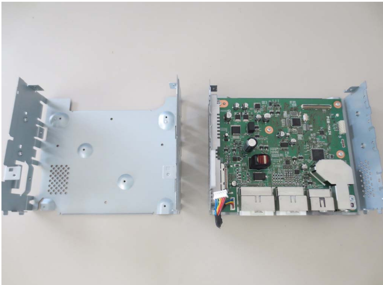
14. PCB-AUDIO case is removed.
