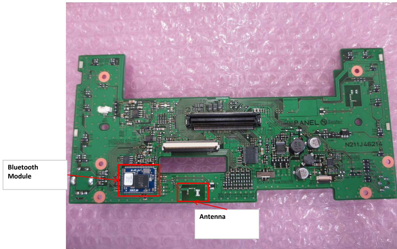
1. PCB-PANEL C-side
