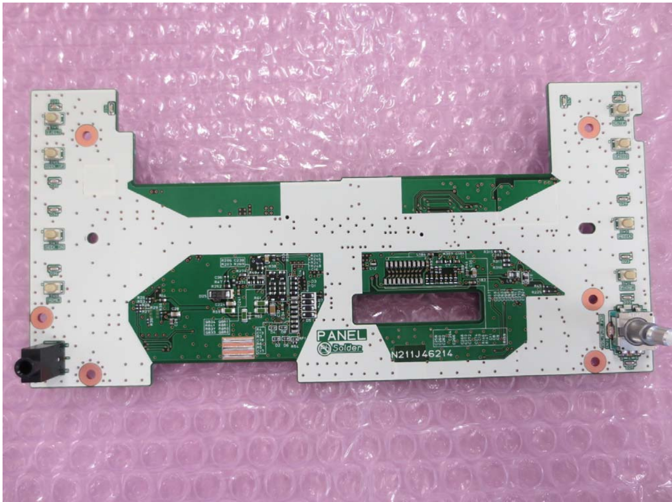
2. PCB-PANEL S-side
